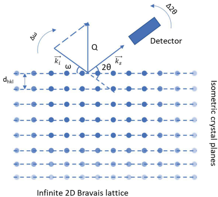
Figure 2-5 Schematic diagram of \omega/2\theta longitudinal scan.
