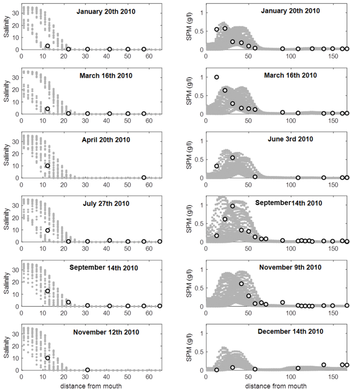
Fig. 3-5 Salinity (left panels) and SPM profiles (rights panels) along the Seine estuary for 6 dates. Dots correspond to measurements, while grey dots correspond to simulated values over 2 tidal cycle for salinity and 20 for SPM
