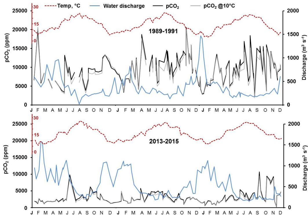
Fig. 1-6 Seasonal variations in calculated pCO 2 at the water temperature (pCO 2 ) and at 10°C (pCO 2 @10°C) values compared with variations in water discharge and temperature values (at Poses) for the two periods: 1989–1991 (atmospheric pCO 2 = 354 ppm) and 2013–2015 (atmospheric pCO 2 = 399 ppm)
