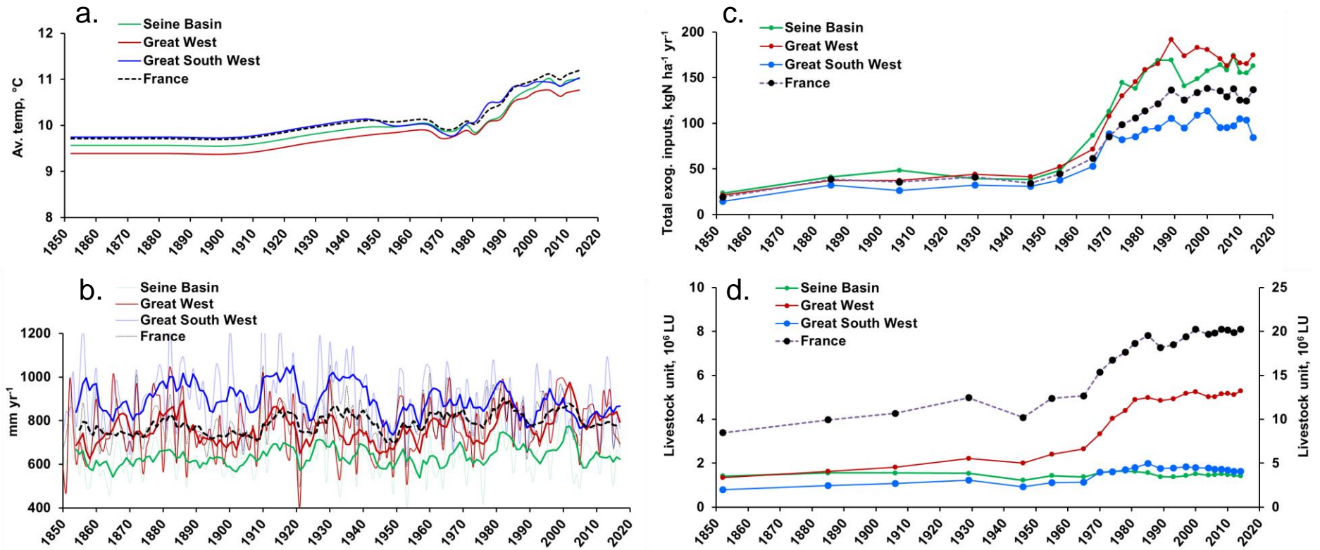
Fig. 5-3. Long-term evolution (1850–2014) for France and the three supra-regions selected in the annual average of a. temperature; b. rainfall. Long-term evolution of major indicators of agriculture in France and the three supra-regions selected for the 22 dates analysed; c. total exogenous N inputs; d. livestock size in terms of livestock units (LU).
