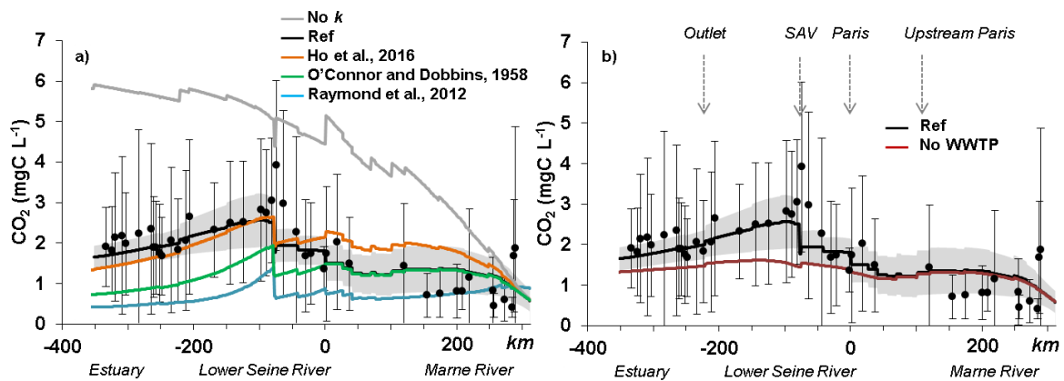
Fig. 2-12. Mean CO 2 concentrations along the main stem of the Seine River depending of a) gas transfer velocities according to O'Connor and Dobbins, (1958) (neglecting the wind); Raymond et al., 2012a, equation 5 in Table 2-2); Ho et al. (2016) (neglecting the wind). Black curve is the reference of our study and grey curve is a simulation with no gas transfer velocity. b) simulations with no discharge of TA and DIC from WWTPs.
