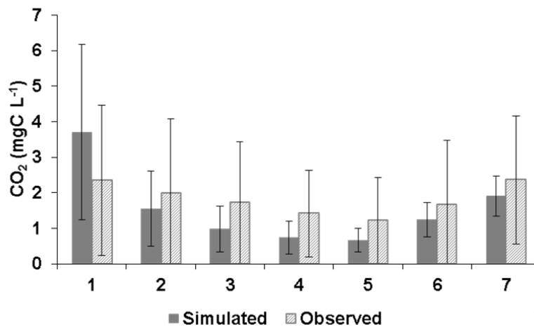
Fig. 2-4 Simulated and observed carbon dioxide concentrations in the Seine waters ( \text{CO}_2 , \text{mgC-CO}_2\text{L}^{-1} ) as a function of the stream order averaged on the period 2010 – 2013 (whiskers indicating standard deviations).
