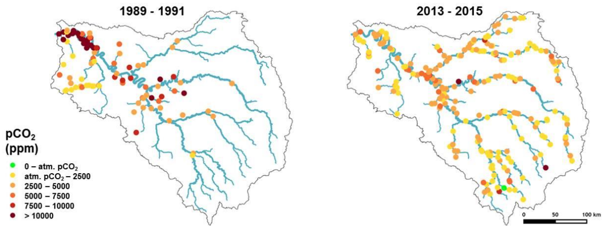
Fig. 1-7 Spatial variations in calculated p\text{CO}_2 averaged over the two periods 1989–1991 (with high organic pollution) and 2013–2015 (after wastewater treatment had been improved). Values are represented for Strahler orders superiors to 2 (Data source: AESN)
