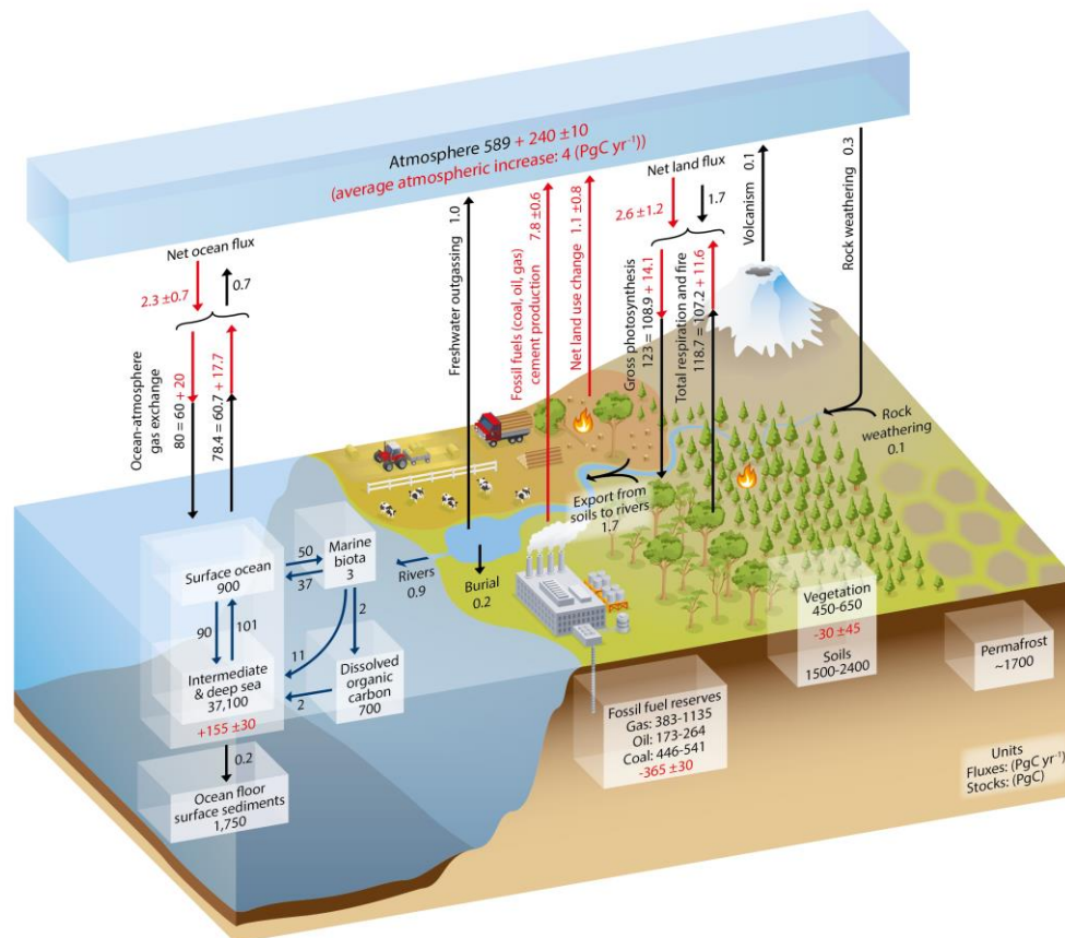
Fig. 0-2 Simplified schematic of the global carbon cycle retrieved from Ciais et al. (2013). Numbers represent carbon stocks in \text{PgC} ( 1 \text{ PgC} = 10^{15} \text{ gC} ) and annual carbon exchange fluxes (in \text{PgC yr}^{-1} ). Black numbers and arrows indicate reservoir mass and exchange fluxes estimated for the time prior to the Industrial Era, about 1750.
