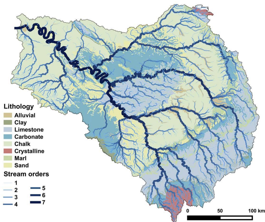
Fig. 4-9 Map of the lithology (Albinet, 1967) and stream orders (Strahler, 1952; 1957) in the Seine basin.
