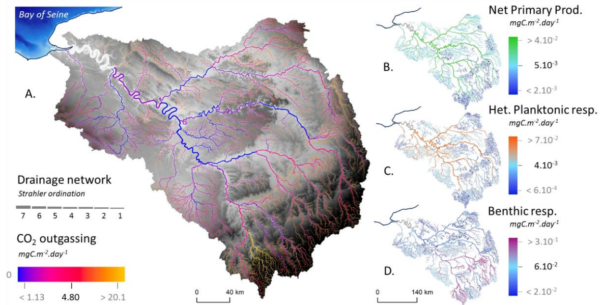
Fig. 2-7. Instream processes involved in the inorganic carbon cycle simulated by pyNuts-Riverstrahler and averaged on the period 2010-2013 for the whole Seine river network. CO 2 outgassing (A. blue - yellow, mgC m -2 day -1 ), net photosynthesis (B. blue – green, mgN m -2 day -1 ), benthic (C. blue - violet) and heterotrophic planktonic (D. blue - orange) respiration (mgC m -2 day -1 ) are represented in the hydrographic network.
