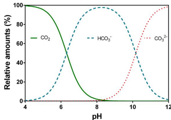
Fig. 0-3 Relative speciation (%) of carbon dioxide (CO 2 ), bicarbonate (HCO 3 - ), and carbonate (CO 3 2- ) in water according to pH retrieved from Pedersen et al. (2013). Speciation was computed with CurtTiPot (Gutz, 2012) using pK 1 =6.532 and pK 2 =10.329 at 20°C with electrical conductivity of 250 μS cm -1 (Schwarzenbach and Meier, 1958).
