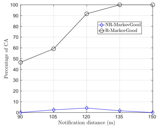
(b) MarkovGood model
