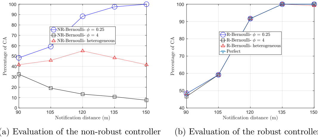
Figure 4.38: Comparing collision avoidance statistics for different localization systems under communication error modeled using Bernoulli model
