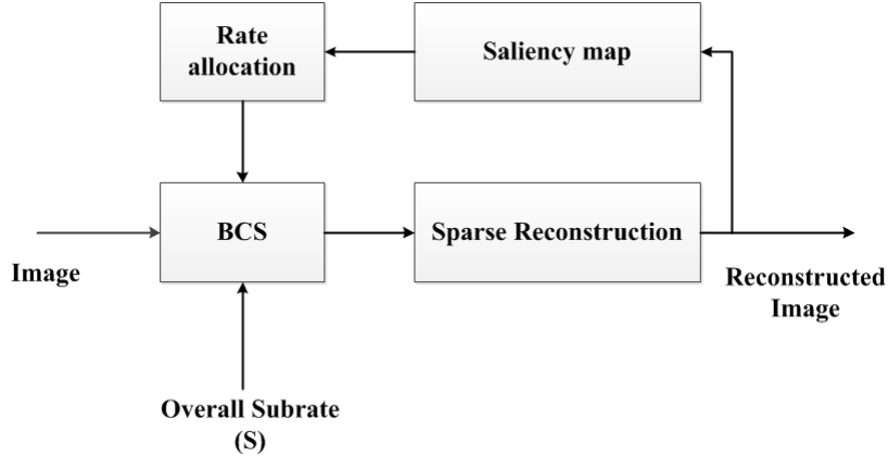
Figure 3.1: Block diagram of the SBCS-SPL framework.
