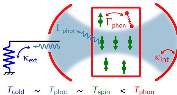
Figure 1.1: Spin radiative cooling principle. Spins (green) in a crystal (red) are coupled both to a bath of phonons at temperature T_{\text{phon}} with a rate \Gamma_{\text{phon}} and to a bath of microwave photons at a temperature T_{\text{phot}} with a rate \Gamma_{\text{phot}} , which determines their equilibrium temperature T_{\text{spin}} . The temperature of the photons T_{\text{phot}} is determined by their coupling with rate \kappa_{\text{int}} to the cavity internal losses at T_{\text{phon}} and with rate \kappa_{\text{ext}} to the load located at the cavity input. When this load is placed at low temperature T_{\text{cold}} , the intra-cavity field is radiatively cooled provided that \kappa_{\text{ext}} \gg \kappa_{\text{int}} and the spins are cooled in turn if \Gamma_{\text{phot}} \gg \Gamma_{\text{phon}} .
