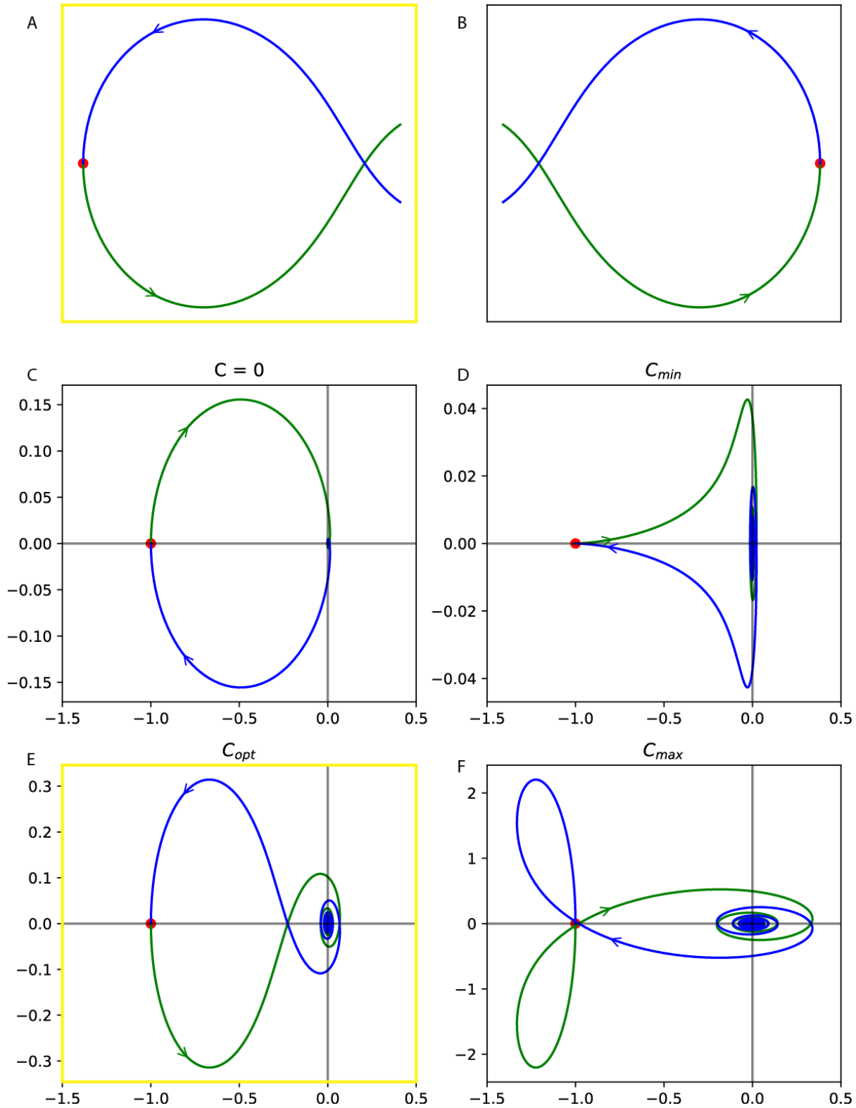
Figure 2.10 Nyquist curves.
