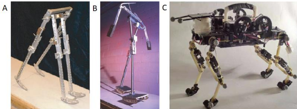
Figure 1.10 Embodied robotics. A. A passive dynamic walker based on McGeer's design. B. The Cornell passive biped with arms. C. Cheetah-Cub, a quadruped robot with compliant legs. A. and B. are taken from Collins et al. (2005), C. from Spröwitz et al (2014).
