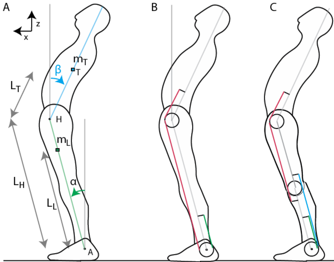
Figure 2.7 Double pendulum model of human stance. The legs can rotate around the ankle joint at A and form an angle \alpha with the vertical. The torso can rotate around the hips at H, of height L_H , and forms an angle \beta with the vertical. The legs have a mass m_L at height L_L and the torso has a mass m_T at height L_T with respect to the hips. B. Cancelling the torque of the torso weight around the hips could be achieved through the stiffness of a pluri-articular muscle (in red) whose length depends only on the torso angle; cancelling the torque of the body weight around the ankles could be achieved through the stiffness of an additional ankle muscle (in green). C. There is no muscle spanning both the hip and the ankle joints in the human body, however there is the rectus femoris (in red) which spans both the hip and the knee joints, the gastrocnemius (in blue) which spans both the knee and the ankle joints, and the soleus (in green) which spans only the ankle joint.
