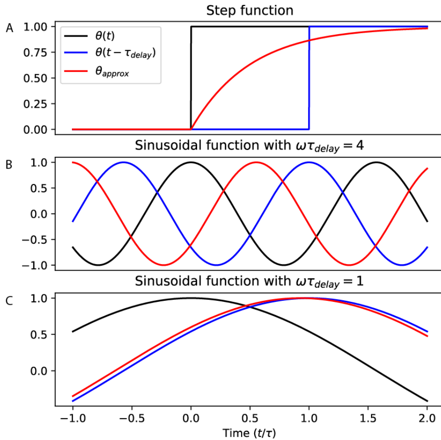
Figure 2.13 Pade approximation of the time delay.
