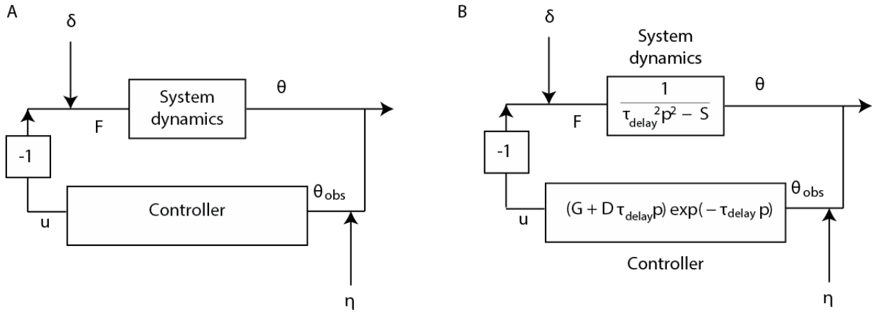
Figure 2.8 Block diagram of the controlled system
