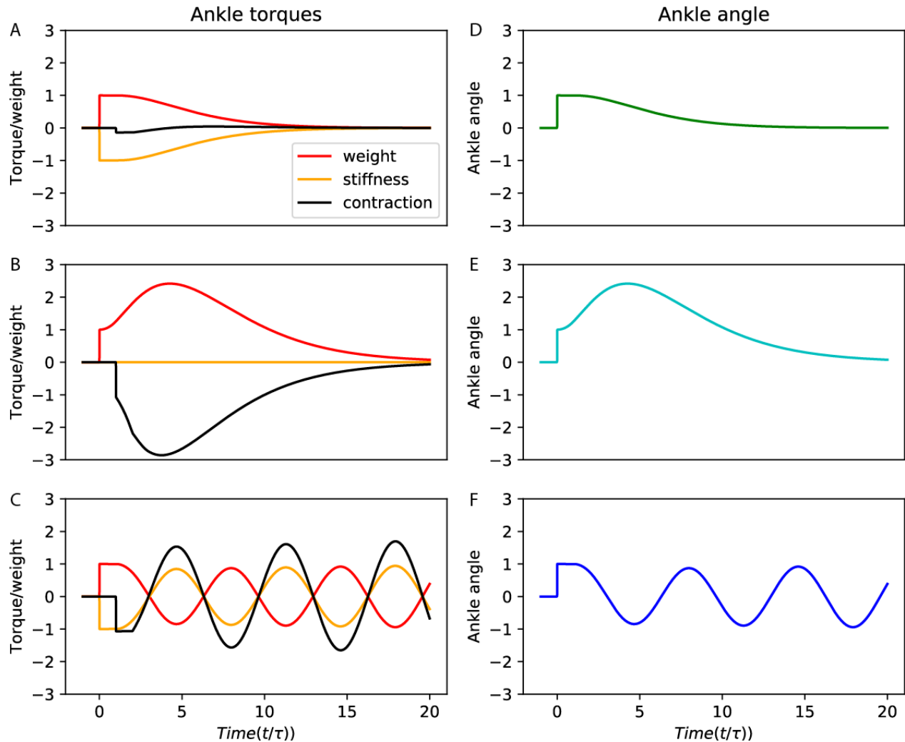
Figure 2.6 Response to perturbations. A. Response of a slow system S=0 with critical damping. B. Response of a fast system S=0.5 with critical damping. C. Response of a slow system S=0 with the same feedback controller as in B. The left panels show the time-course or the torque of weight (red), and the components of the ground reaction torque due to stiffness (orange) and feedback contraction (black), normalised to weight. The right panels show the time-course of ankle angle. The response delay (between the perturbation and the first change in contraction) is shaded in grey.
