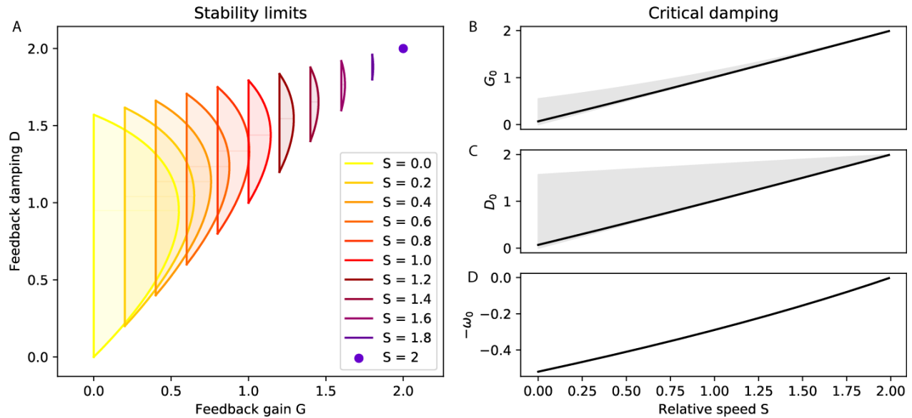
Figure 2.5 Delayed feedback control. A. Stability limits. The range of stable feedback gain G and damping D is plotted for different values of relative speed S ranging from S = 0 to the maximal S = 2 . B-D Optimal controller. B. The feedback gain G_0 , which provides critical damping is plotted in black as a function of S . The range of stable feedback gains is shaded in grey. C. The feedback damping D_0 , which provides critical damping is plotted in black as a function of S . The range of stable feedback damping is shaded in grey. D. The eigenvalue of the system with critical damping is plotted as a function of S .
