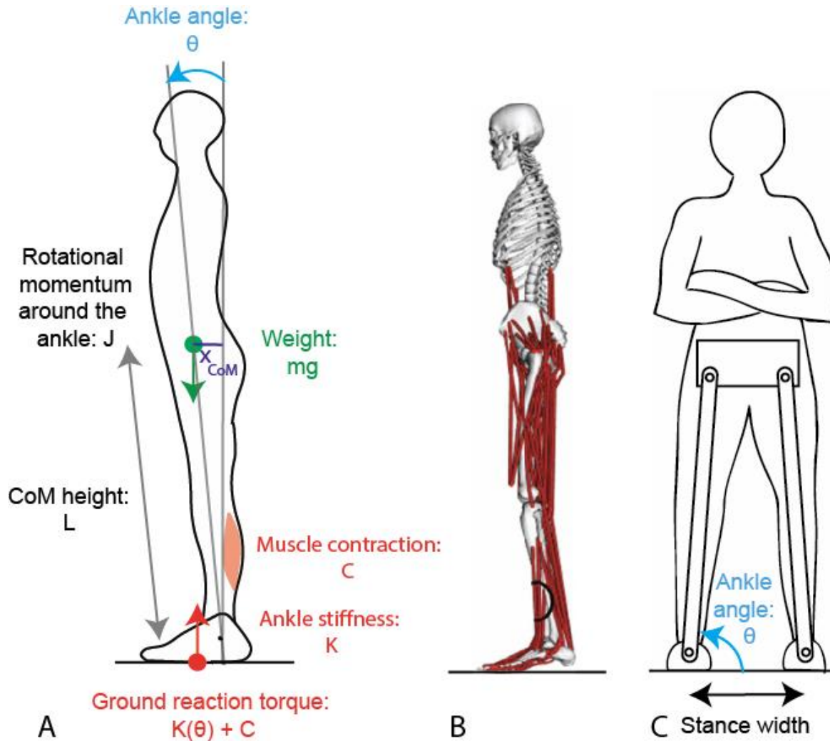
Figure 2.3 Models of stance. A. Single inverted pendulum model used in Loram and Lakie (2007). The external forces acting on the body are the weight (green arrow), whose torque around the ankle depends on ankle angle \theta , and the ground reaction force (red arrow) whose torque depends on both ankle angle and muscle contraction. B. Detailed model used in De Groot et al. (2017). C. Single dimensional model of lateral stance used in Bingham et al. (2011).
