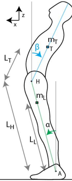
Figure 6.2 Double pendulum model of human stance.
