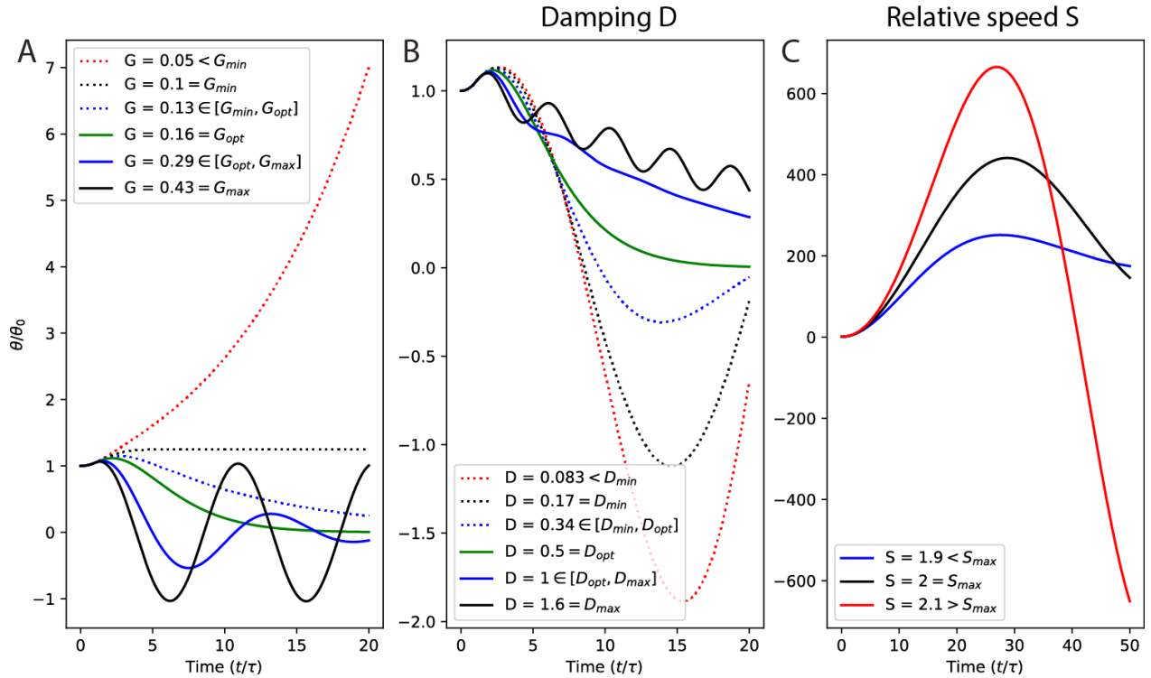
Figure 2.12 Response to a perturbation.
