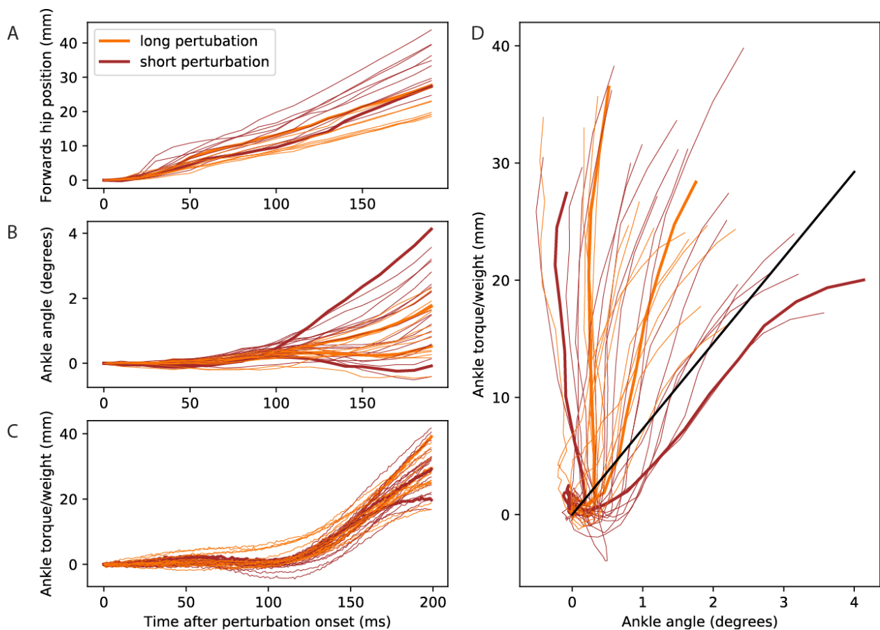
Figure 4.6 Ankle stiffness.
