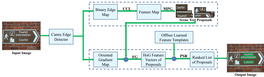
FIGURE 4.1 – The framework of the proposed scene text proposal technique, including a max-pooling based grouping strategy for scene text proposal generation and a low-level feature based proposal ranking ( CCL : Connected Component Labelling, MPG : Max-Pooling based Grouping, FG : Feature Generation, PSR : Proposal Scoring Ranking)
