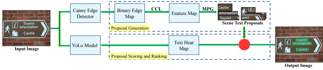
FIGURE 6.5 – The proposed framework for future development of maxpooling based scene text proposal by adopting a YoLo model for scoring proposals. CCL is connected component labelling and MPG is maxpooling based grouping.
