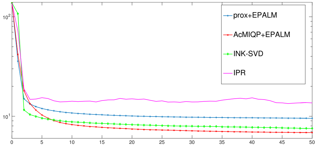
Figure 5.1 – The convergence of the exact \ell_0 based incoherent dictionary learning algorithm (AcMIQP+EPALM) and its comparison to the prox+EPALM, the INK-SVD and IPR algorithms
