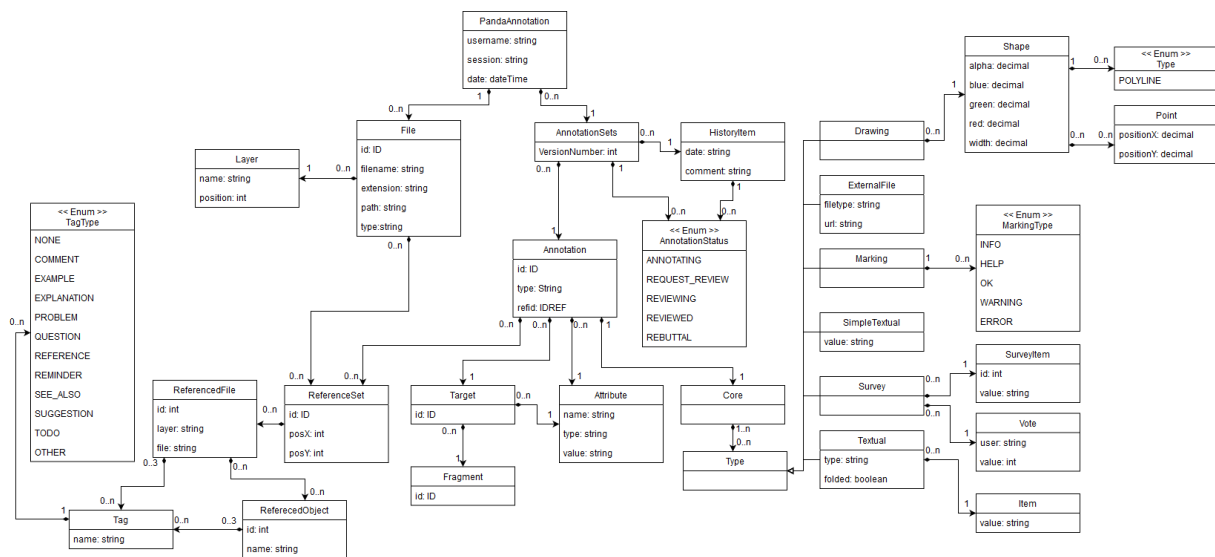
Figure 6-2 Graphical representation of the XSD
