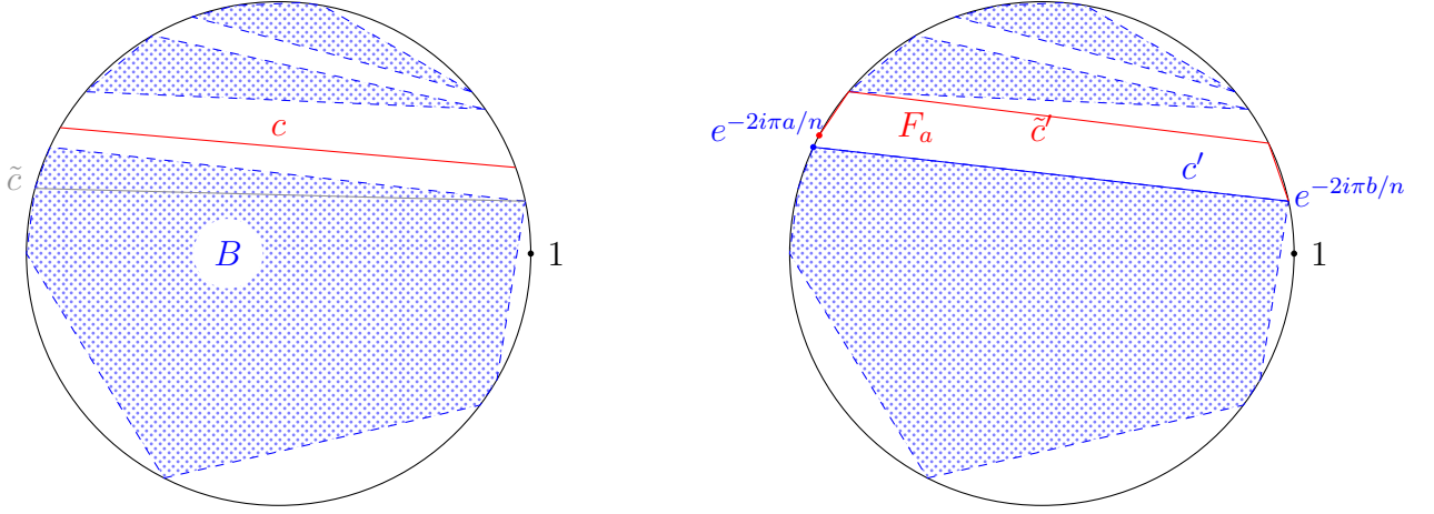
Figure 3.14: Left: the red chord c is a large chord of \overleftarrow{C}_u^{(n)} , and the gray chord \tilde{c} is a chord of C_{n-u}^{(n)} , which is close to c . B denotes the block of P_{n-u}^{(n)} containing \tilde{c} . Thus, the boundary of B necessarily contains a chord inbetween c and \tilde{c} . Right: the blue chord c' is a large chord of P_{n-u}^{(n)} , and the red chords are the chords of \overleftarrow{C}_u^{(n)} that are part of the boundary of F_a . Among these chords, with high probability, one of them (denoted by \tilde{c}' here) is not far from c' .
