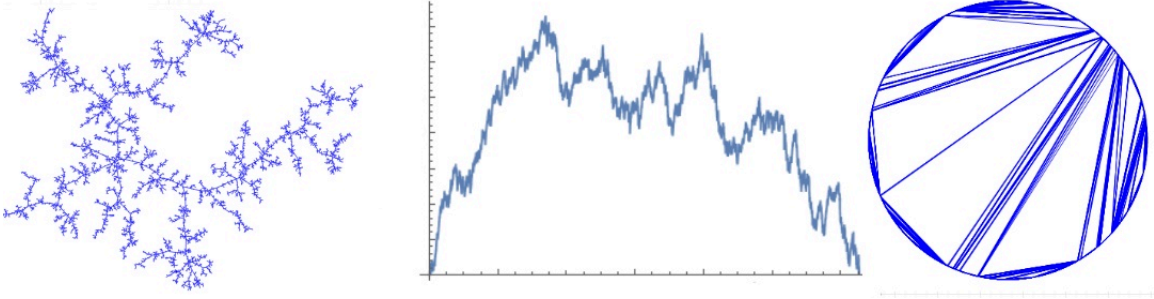
Figure 3.3: An approximation of (\mathcal{T}^{(2)}, H^{(2)}, \mathbb{L}_\infty^{(2)}) .
