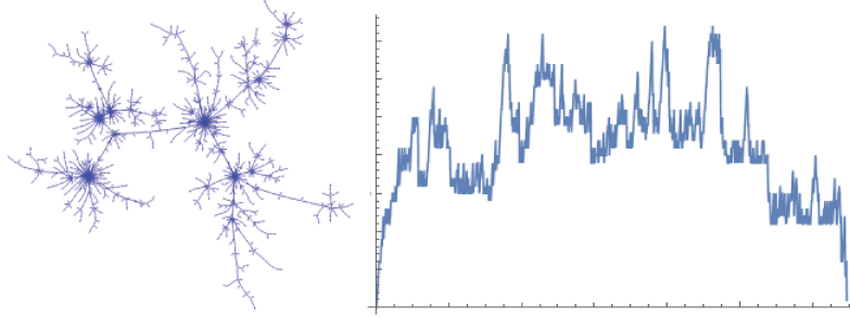
Figure 3.1: An approximation of (\mathcal{T}^{(1.5)}, H^{(1.5)}, \mathbb{L}_\infty^{(1.5)}) .
