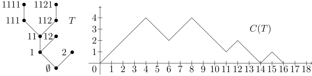
Figure 3.7: A tree T with 9 vertices labelled à la Neveu, and its contour function (C_t(T))_{0 \leq t \leq 18} .
