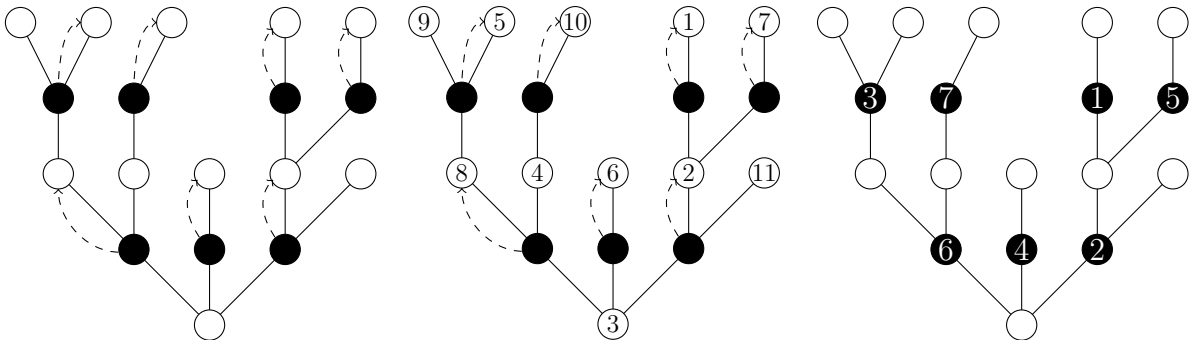
Figure 4.11: The coupling between labels of black and white vertices in a tree: arrows go from a black vertex u to the white vertex lc(u) . Left: the coupling between vertices. Middle: a uniform labelling of the white vertices. Right: the induced labelling of the black vertices
