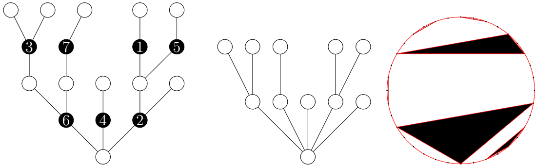
Figure 4.9: A labelled bi-type tree T , its associated white reduced tree T^\circ and the lamination \mathbb{L}_6^\bullet(T) .
