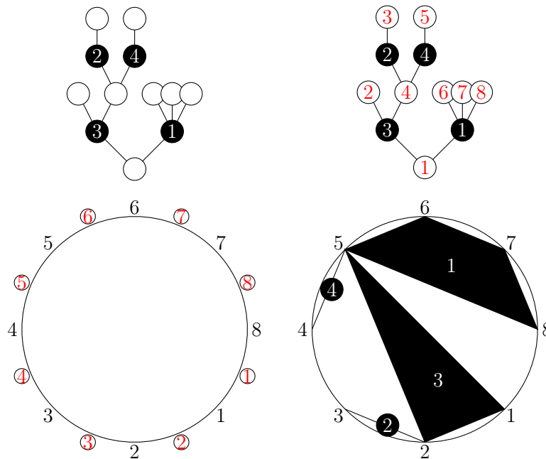
Figure 4.16: An example of the inverse bijection \Phi_8 \circ (\Psi_8)^{-1} . Top-left: a tree T \in \mathfrak{U}_8 . Top-right: the tree T with labels on its white vertices, following the white exploration process. Bottom-left: the locations of the arcs corresponding to these white vertices, on the circle. Bottom-right: the associated colored lamination. We recover from this: \Psi_8^{-1}(T) = (5678)(23)(125)(45) .
