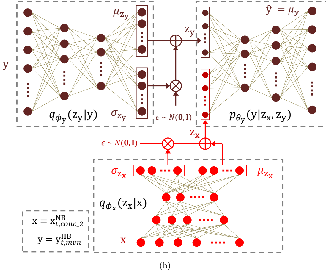
Figure 6.4: A feature extraction scheme using (a) VAE and (b) CVAE.
