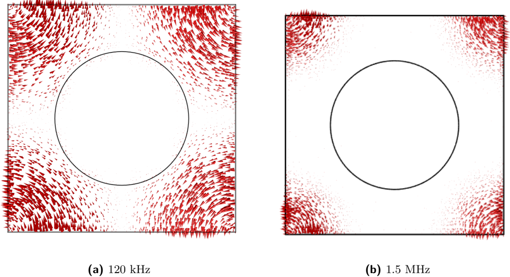
Figure 4.39: Eddy current
