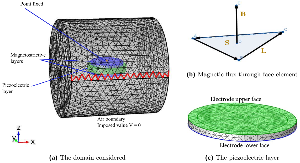
Figure 2.3: Boundary conditions
