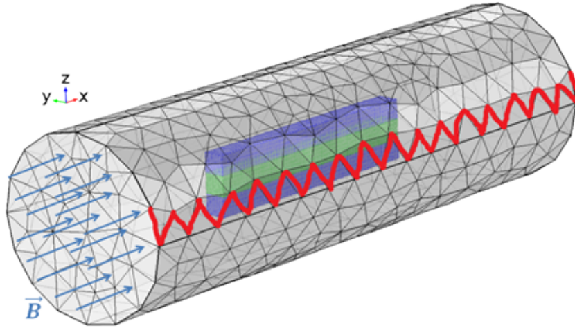
Figure 3.18: The study domain enveloping the magnetolectric device. In red the cutting path on which nonzero edge values of \mathbf{a} are applied to impose the magnetic flux.
