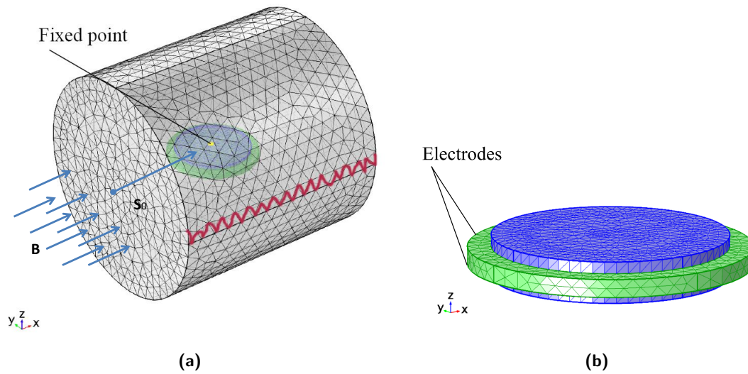
Figure 3.2: Mesh and boundary condition magnetostrictive layer in blue color and piezoelectric layer in green color
