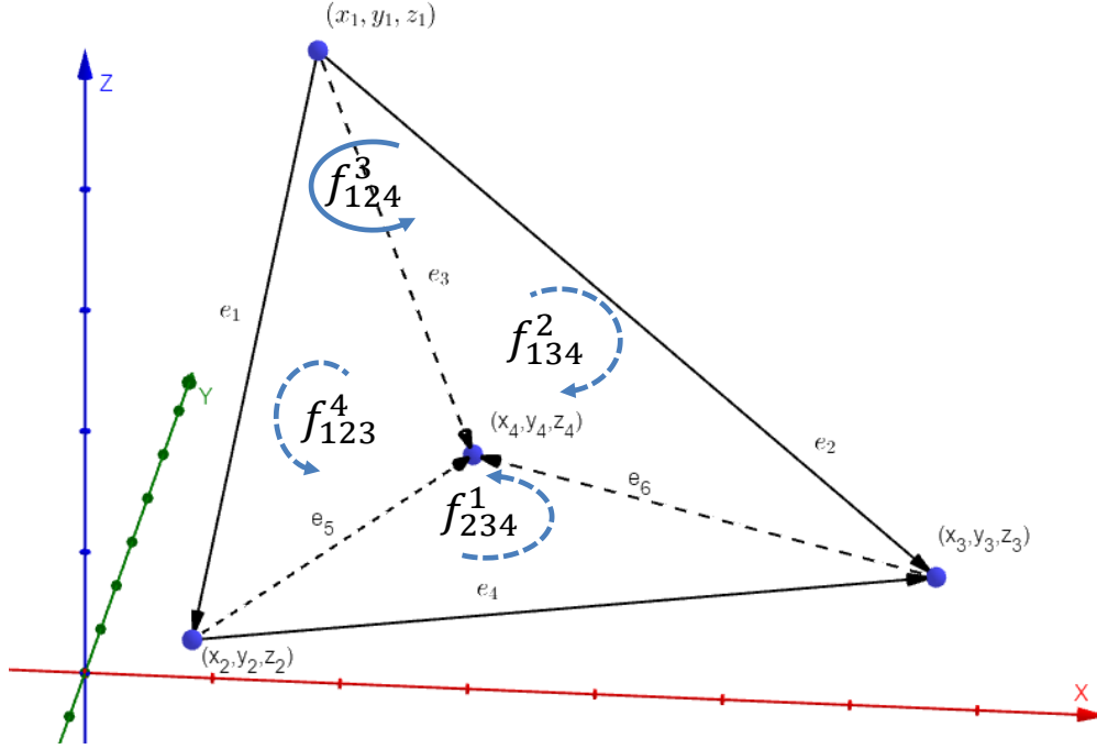
Figure 2.2: Tetrahedral element
