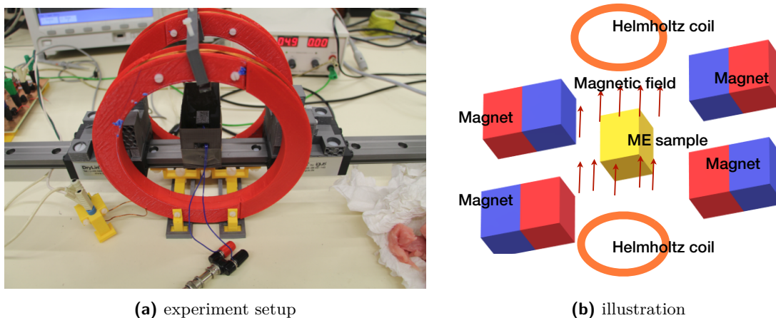
Figure 2.1: Measurement of ME coefficient
