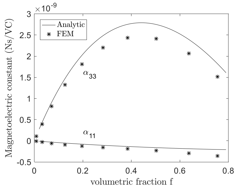
Figure 4.15: Effective magnetolectric moduli as the function of volume fraction f of piezoelectric phase.
