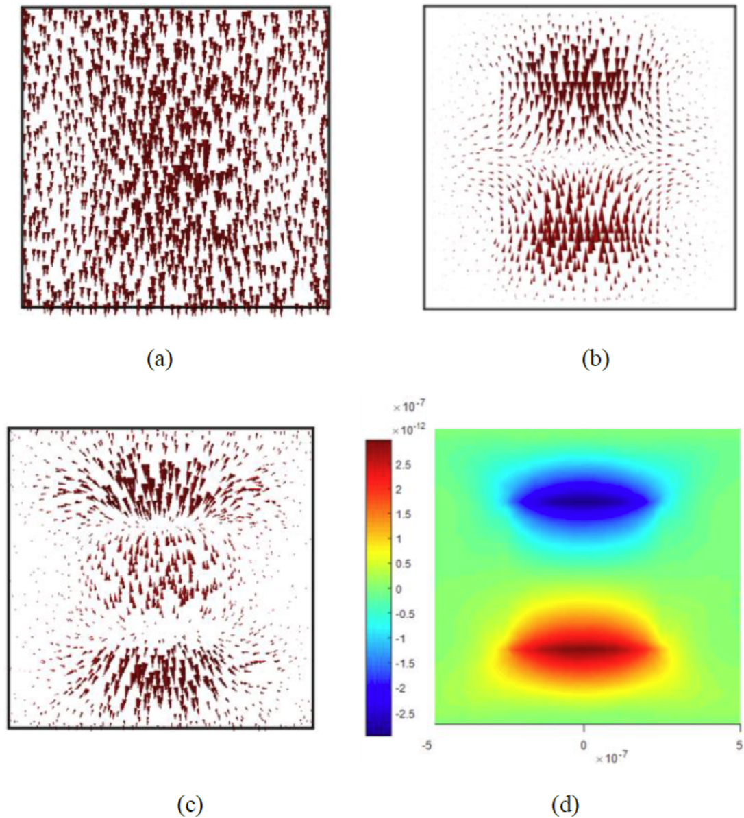
Figure 4.26: The magnetic field (a), displacement field (b) the electric field (c) and the electric potential (d) distributions on a cutting plane when \vec{H}_3 is applied.
