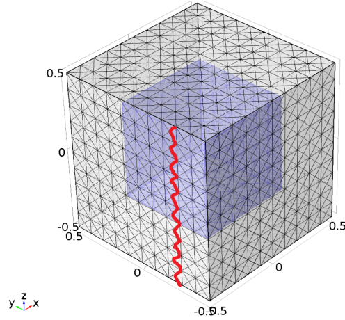
Figure 4.3: Mesh of a periodic REV cell. In red: cutting edges on which nonzero edge values of a are applied to allow the magnetic flux crossing the cell.
