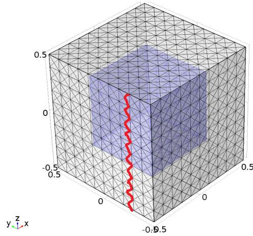
Figure 4.3: Mesh of a periodic REV cell. In red: cutting edges on which nonzero edge values of a are applied to allow the magnetic flux crossing the cell.
