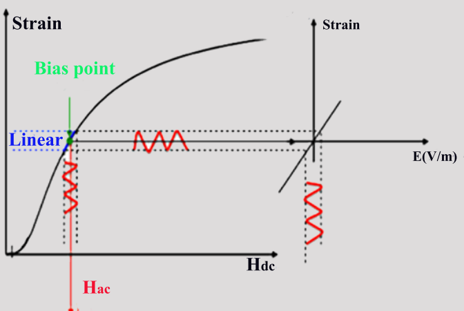
Figure 2.4: Bias-point in magnetoelectric analysis
