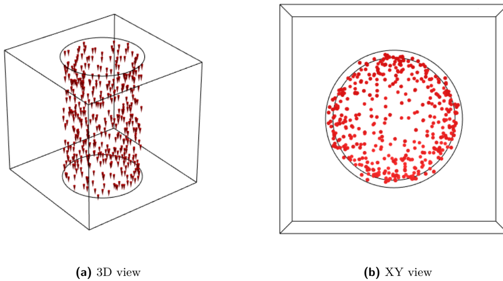
Figure 4.18: Electric displacement D_3 distribution when E_3 is applied
