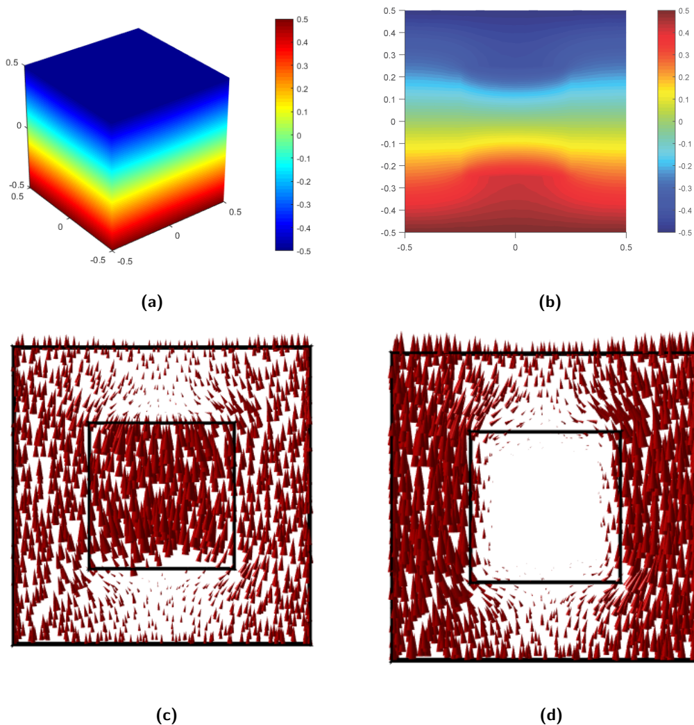
Figure 4.30: The electric potential 3D view (a), electric potential on cutting plane (b) the electric field (c) and the electric displacement (d) distributions on a cutting plan when \vec{E}_3 is applied.
