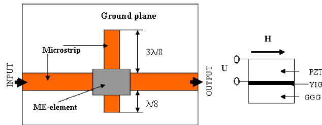
Figure 1.17: ME phase shifter [56]
