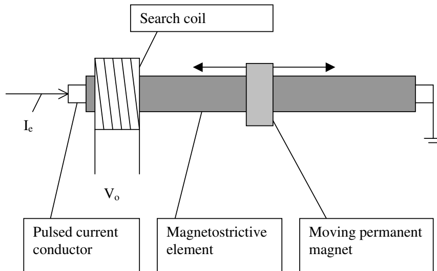
Figure 1.6: Schematic diagram of the magnetostrictive delay lines in measuring position [17]
