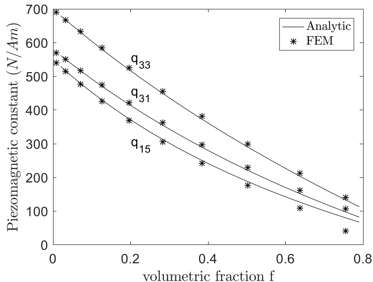
Figure 4.14: Effective piezomagnetic moduli as the function of volume fraction f of piezoelectric phase.
