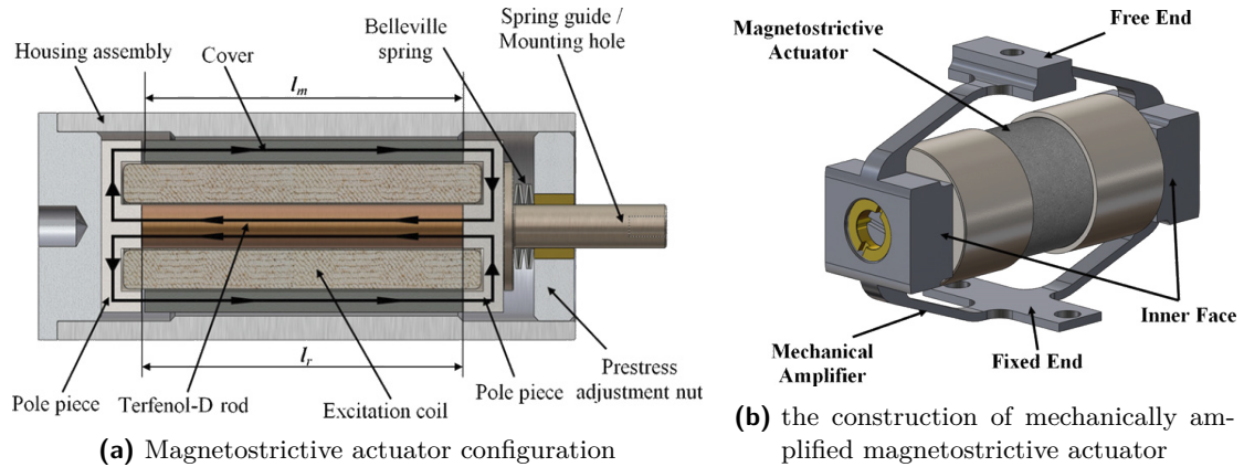
Figure 1.4: Magnetostrictive actuator [15]
