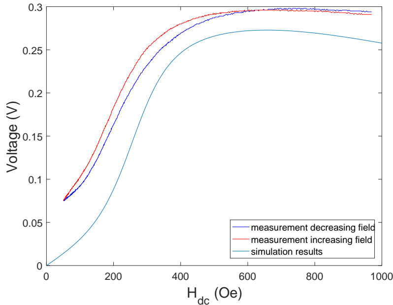
Figure 3.12: ME voltage coefficient as a function of DC magnetic field ( \mathbf{H}_{dc} ).
