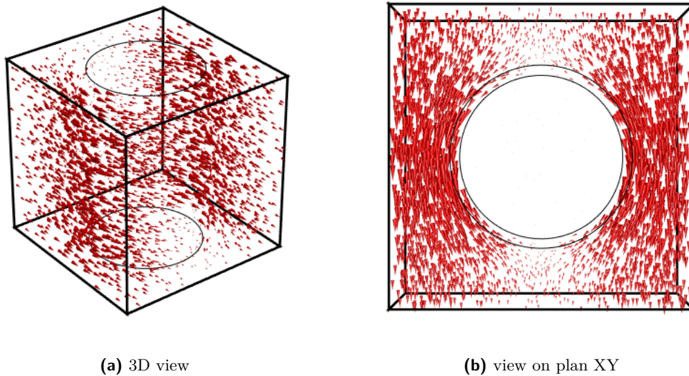
Figure 4.6: Uniaxial magnetic induction \vec{B}_1 is applied
