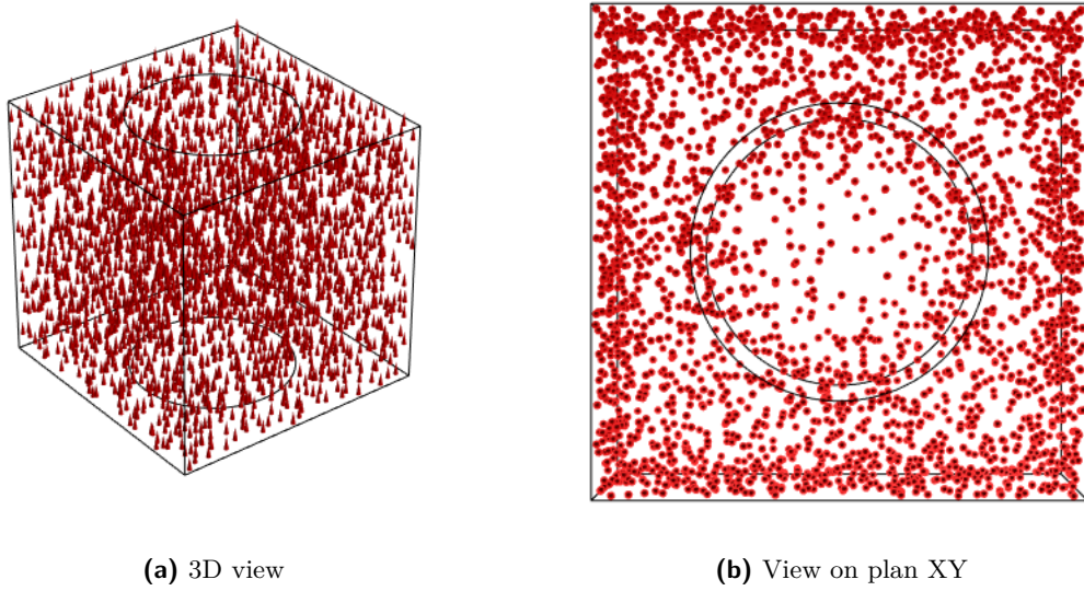
Figure 4.11: Magnetic field H_3 distribution of magnetolectric composite reinforced by fiber piezoelectric when B_3 is applied
