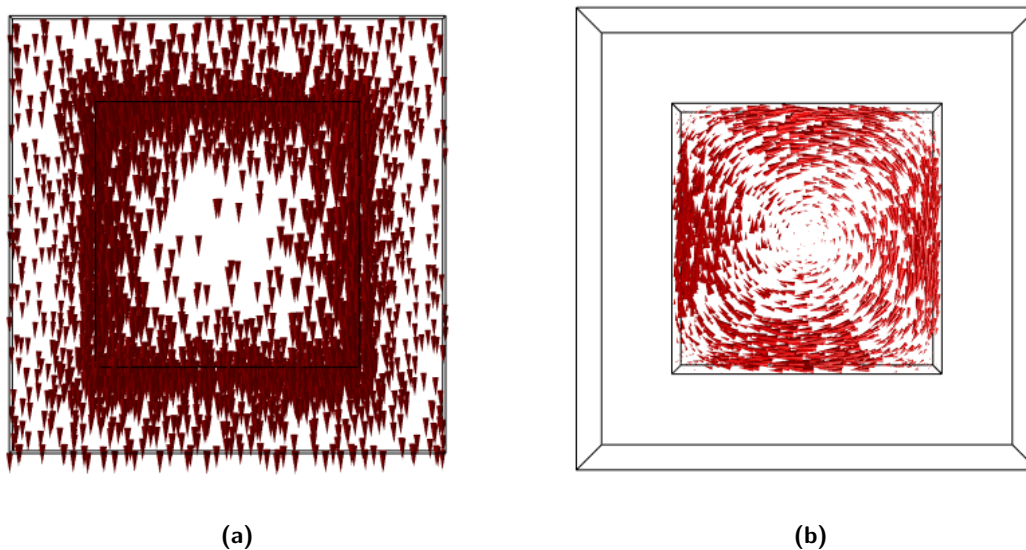
Figure 4.36: Magnetic field (a) and eddy current (b) @ 300kHz
