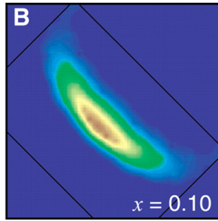
(b) Spectral intensity of \text{Ca}_{2-x}\text{Na}_x\text{CuO}_2\text{Cl}_2 , x = 0.10 , in the top right corner of the Brillouin zone. [149]
