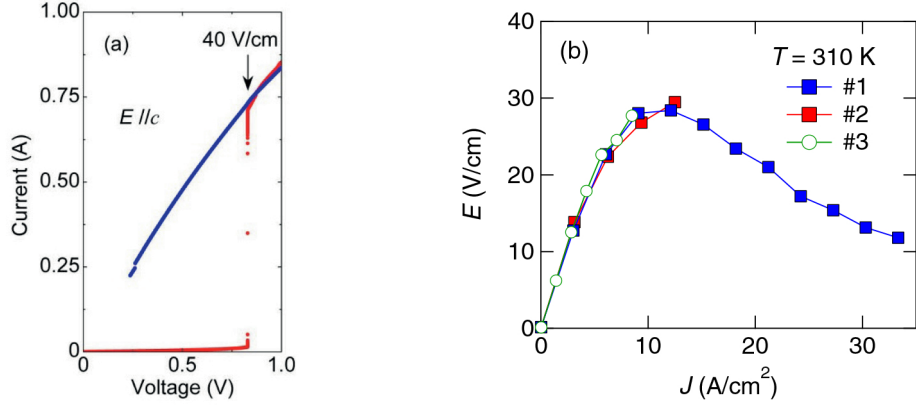
(a) IV characteristics, T = 295\text{K} . [115]
