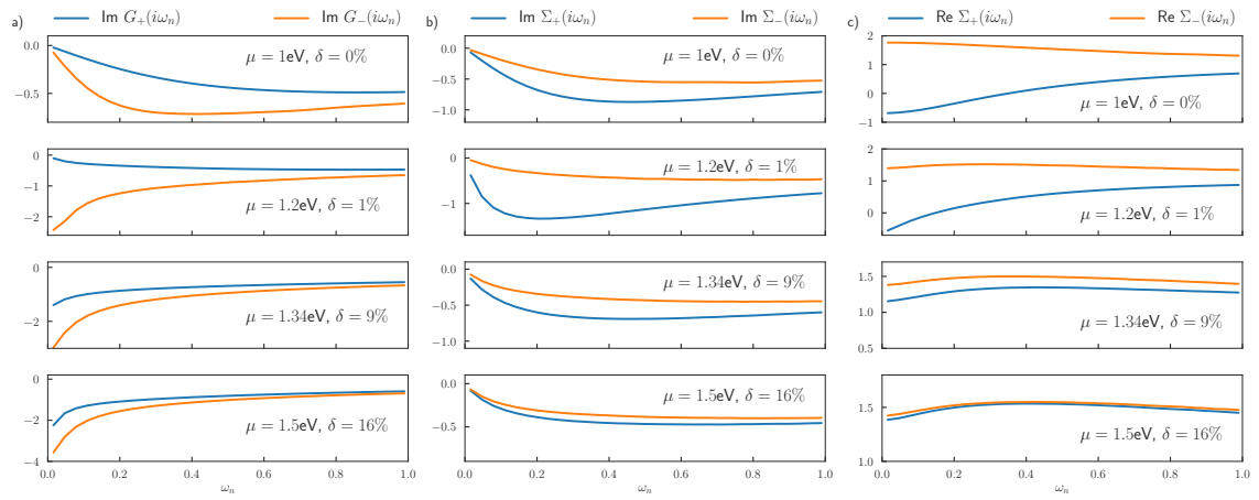
Figure A.1 – Evolution in the even - odd basis of a) the imaginary part of the Green's function G_{\pm}(i\omega_n) , b) the imaginary part of the self-energy \Sigma_{\pm}(i\omega_n) , c) the real part of \Sigma_{\pm}(i\omega_n) as a function of the Matsubara frequency \omega_n . On all plots, the even (odd) contribution is plotted in blue (orange).
