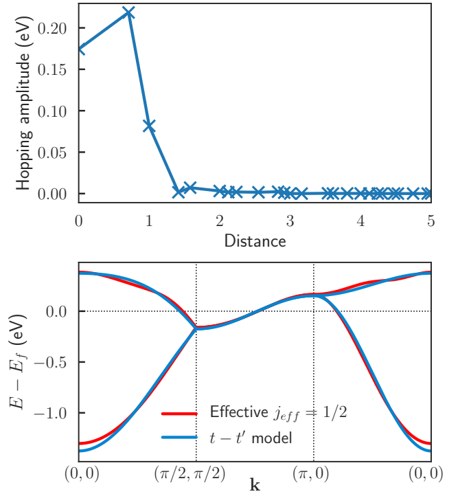
FIG. 3. Upper panel: Real-space hopping amplitudes of the effective j_{\text{eff}} = 1/2 Hamiltonian with respect to the distance (the intersite distance is normalized to 1). Lower panel: Comparison between the effective j_{\text{eff}} = 1/2 bands (red) with E = 0 and the folded dispersion obtained by keeping only the nearest- and next-nearest-neighbor hopping terms ( t = -0.219 eV and t' = -0.082 eV, respectively). Bands are plotted in reciprocal space, along the (0,0) - (\pi/2,\pi/2) - (\pi,0) - (0,0) path of the full Brillouin zone. \Delta_t = 0.15 eV, t_0 = 0.35 eV, e_1 = -1.5 eV, and \lambda = 0.57 eV.
