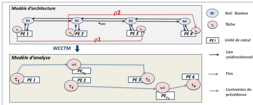
FIGURE 7.5 – Worst Case Communication Time Model (WCCTM) - Exemple de transformation
