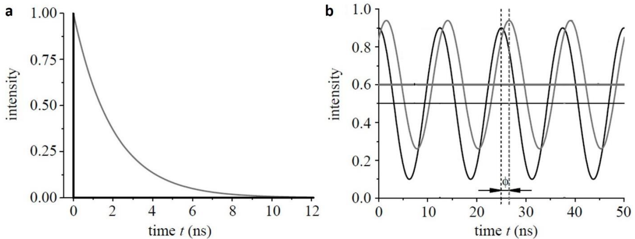
Figure 2.9 Typical examples of two time-resolved measurements for the determination of luminescence decay times. a. Time-domain measurement; b. Frequency-domain measurement. Excitation is displayed in black, emission with a decay time is displayed in grey. (Adapted with permission from reference [140]. Copyright 2013 The Wiley-VCH Verlag GmbH & Co. KGaA.)
