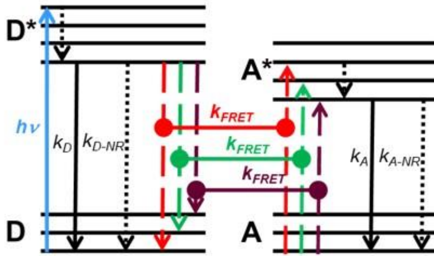
Figure 2.5 Basic FRET principle described in simplified energy level scheme (Jablonski diagram). The donor is excited ( h\nu ) from an electronic ground state (D) to an excited state (D*), then goes to an excited electronic ground state by inner relaxation (dotted arrow), then goes to ground state by radiative decay ( k_D ), non-radiative decay ( k_{D-NR} ) or FRET ( k_{FRET} ). The FRET process from D* to A* occurs when they share the same electronic transition (the difference between the respective energy levels need to be equal, vertical dashed lines in red, green and purple color). After FRET, the acceptor is in an excited state (A*), followed by radiative decay ( k_A ) or non-radiative decay ( k_{A-NR} ) to its ground state (A). (Adapted with permission from reference [140]. Copyright 2013 The Wiley-VCH Verlag GmbH & Co. KGaA.)
