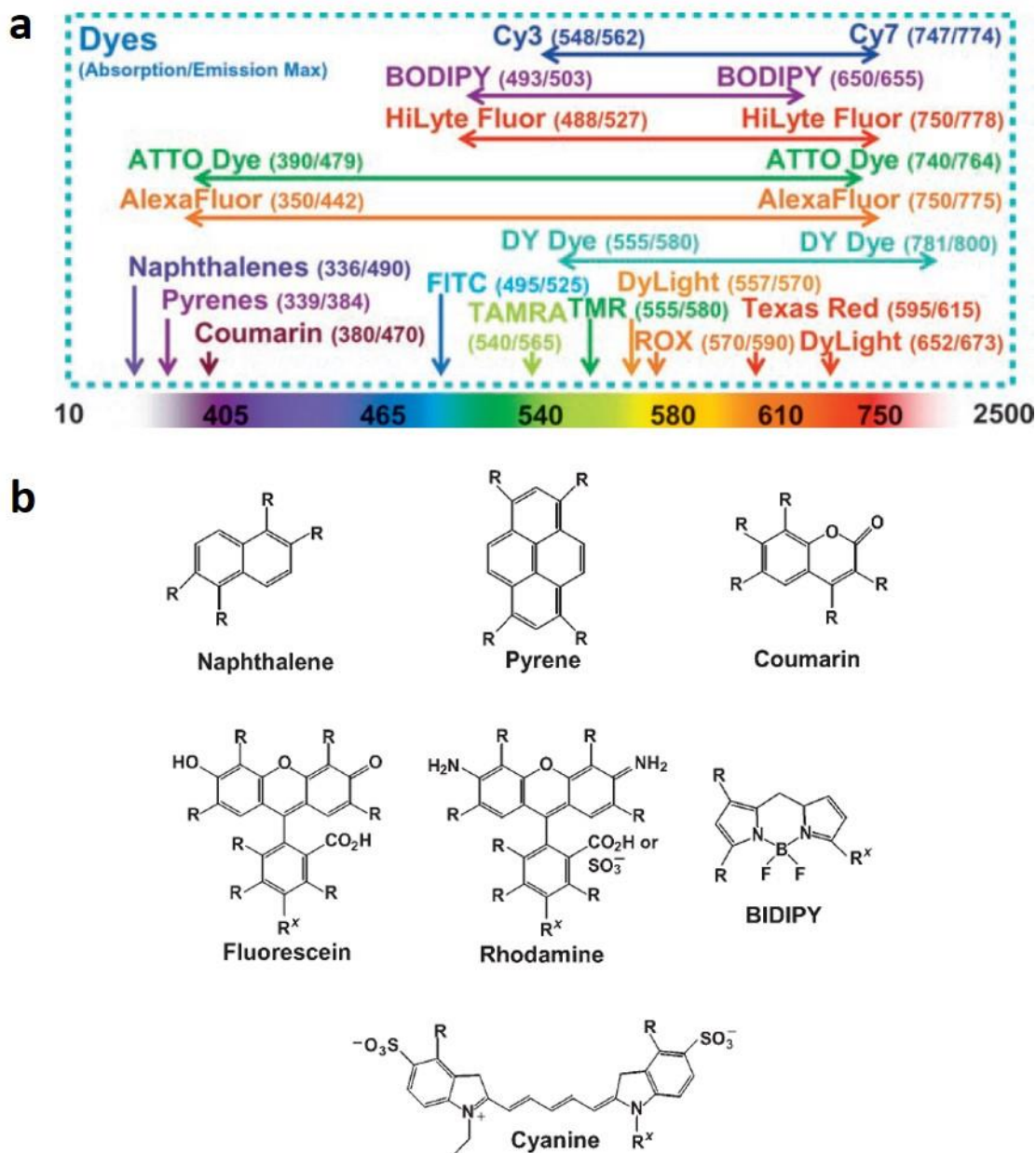
Figure 2.16 a. Common fluorescent dyes. Absorbance and emission maxima along with spectral regions covered by a particular dye family are highlighted. FITC is fluorescein-based dyes; TAMRA, TMR, and ROX are rhodamine-based dyes; Cy3 to Cy7 are cyanine-based dyes; b. Chemical structures of common ultraviolet/visible/near-infrared fluorescent dyes. R marks the typical position of substituents position; R^x marks the typical position of the bioconjugation linker. (Adapted with permission from reference [168]. Copyright 2006 WILEY-VCH Verlag GmbH & Co. KGaA, Weinheim.)
