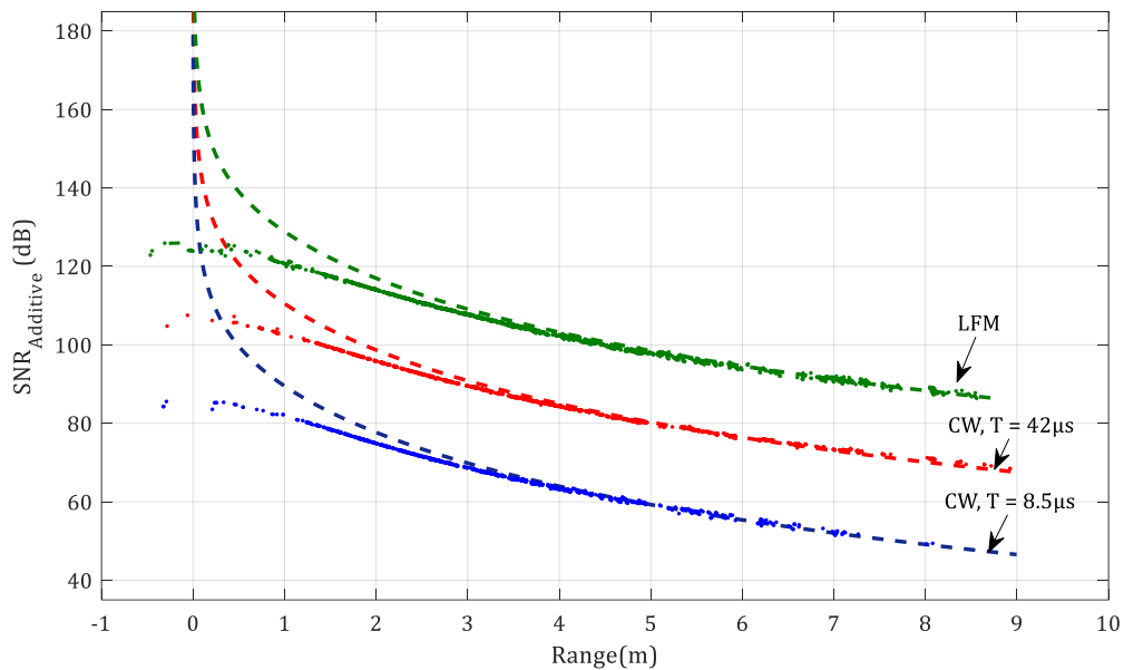
Figure 52 SNR accounting additive noise only, estimated for LFM (80 \mu\text{s} ), CW (8.5 \mu\text{s} ) and CW (42.75 \mu\text{s} )
