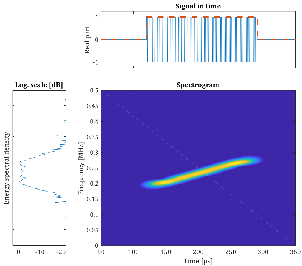
Figure 46 Spectrogram of a Linear Frequency Modulated Pulse (LFM) with rectangular envelope
