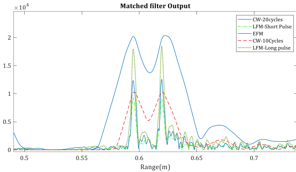
Figure 51 Matched filter outputs with different transmit pulses
