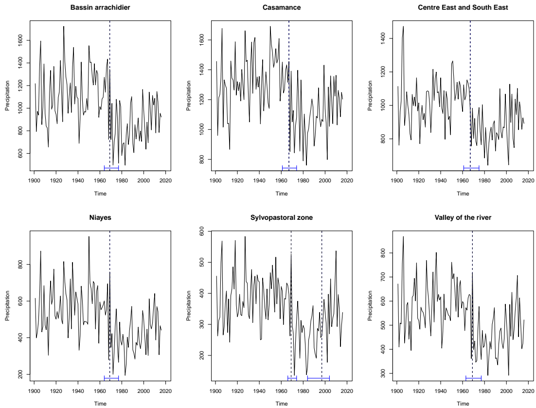
Figure 1.91 Breaks in total annual precipitation in the agroecological zones of Senegal.
