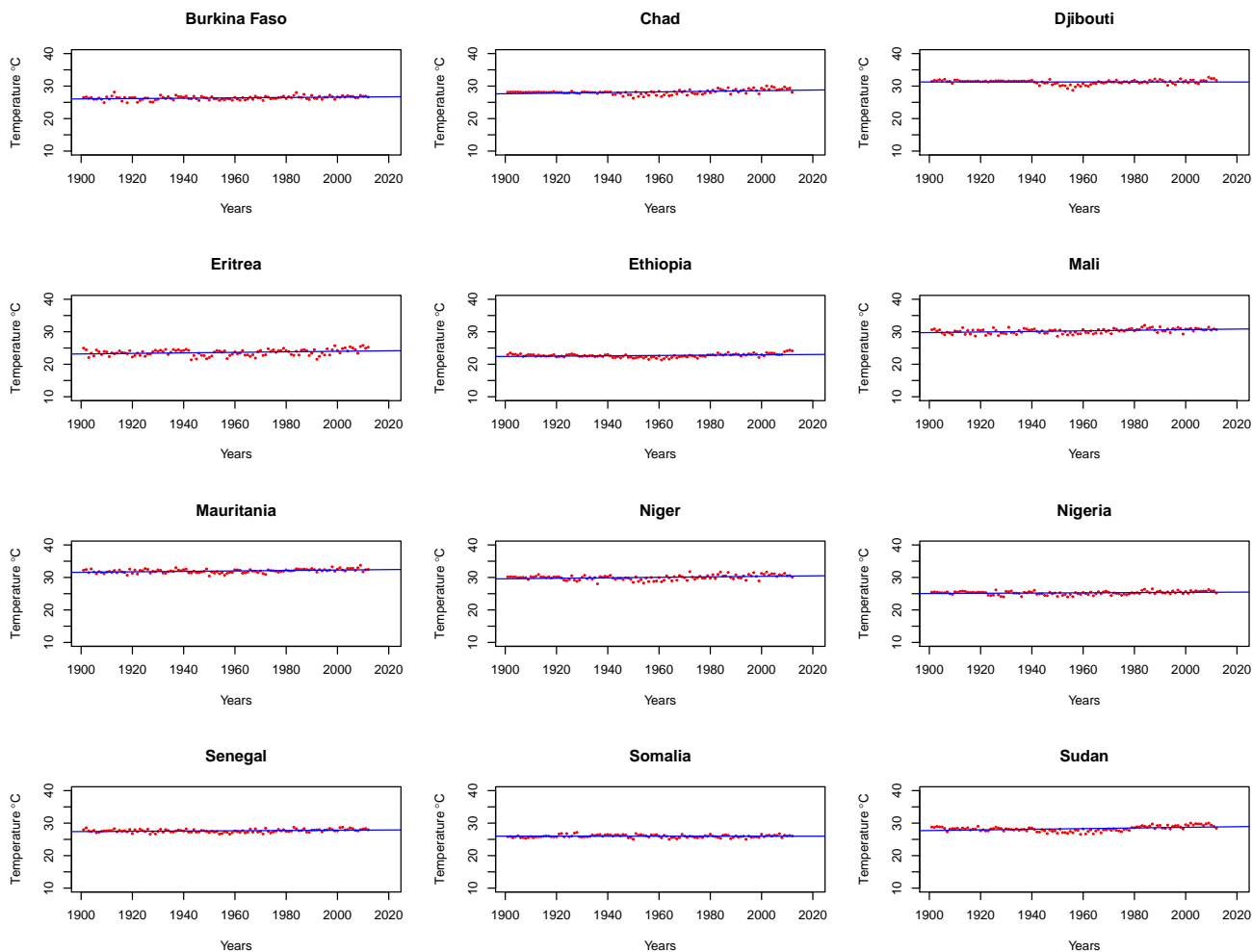
Figure 1.4 Minimum annual temperature during the rainy season in the Sahel countries from 1901 to 2016
