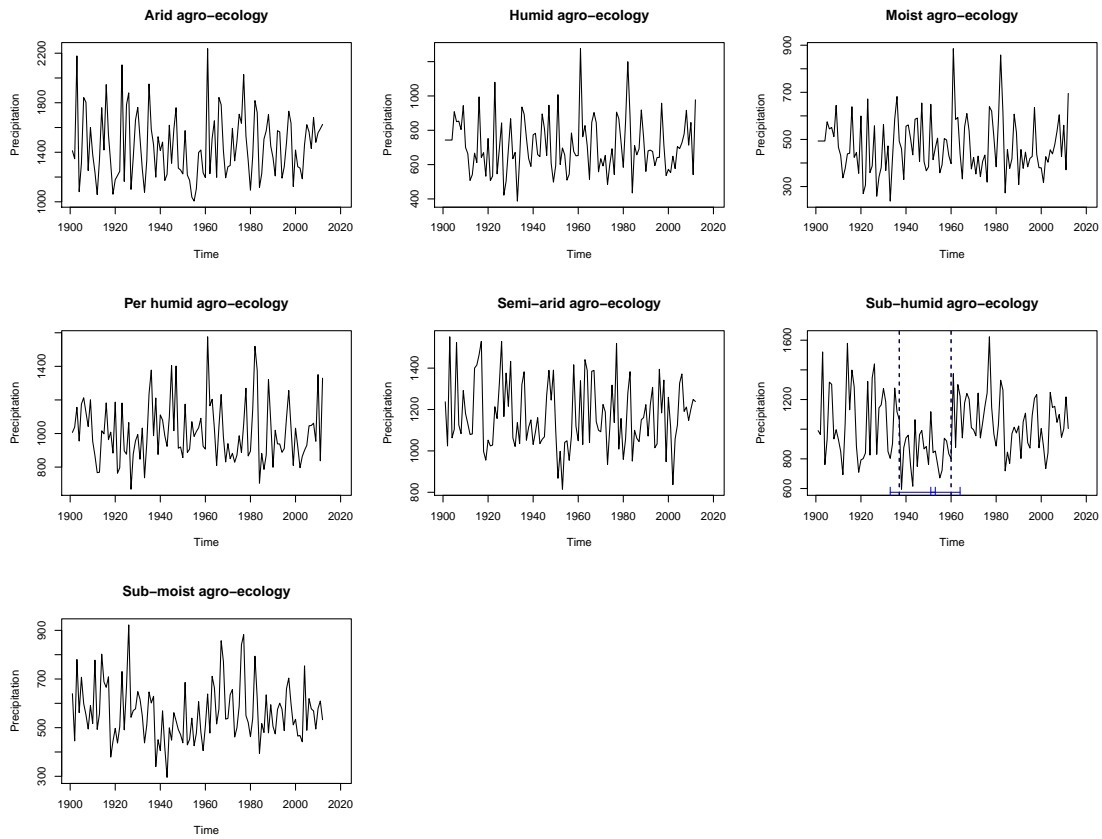
Figure 1.51 Breaks in total annual precipitation in the agroecological zones of Ethiopia.
