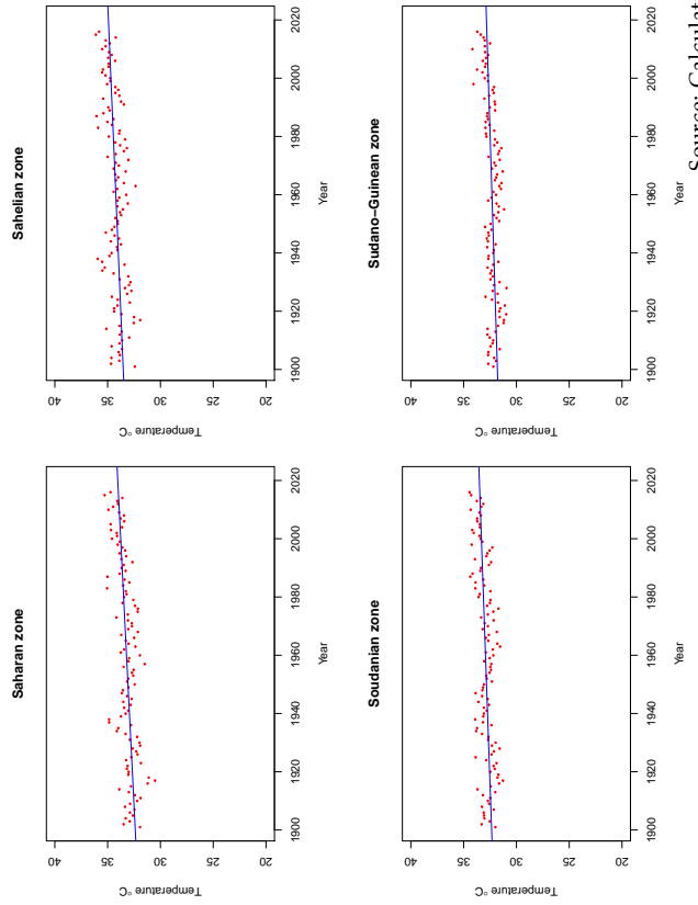
Figure 62.c: Maximum annual temperature
