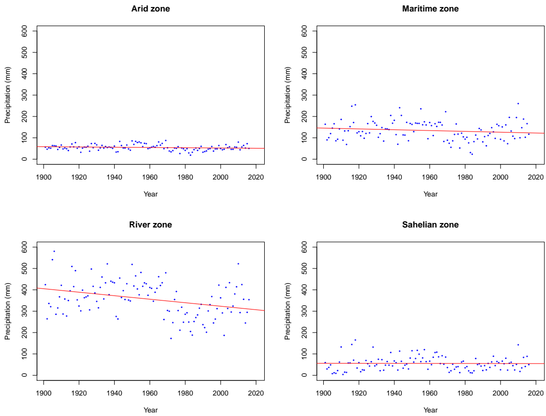
Figure 1.65 Evolution of the sum annual rainfall (mm) from 1901 to 2016 in the agroecological zones of Mauritania
