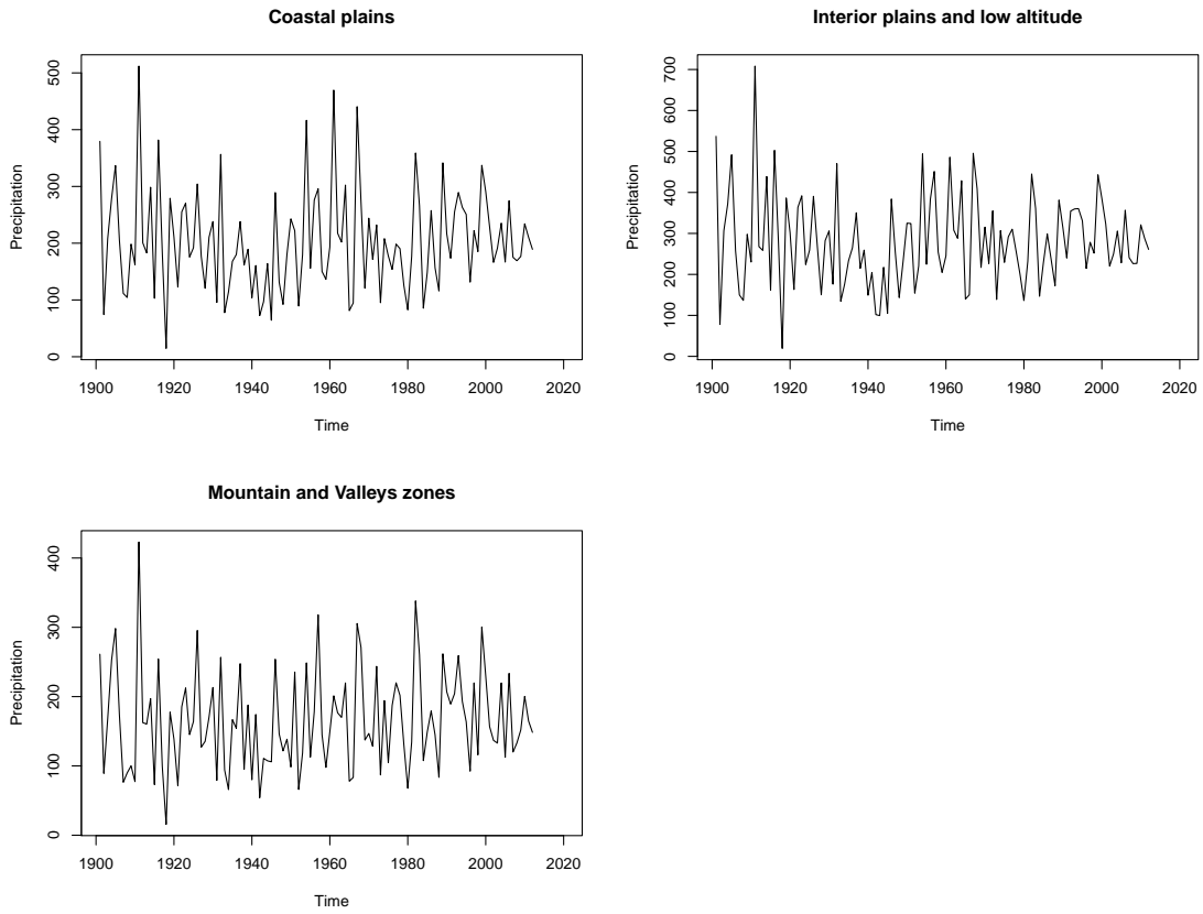
Figure 1.43 Breaks in total annual precipitation in the agroecological zones of Djibouti.
