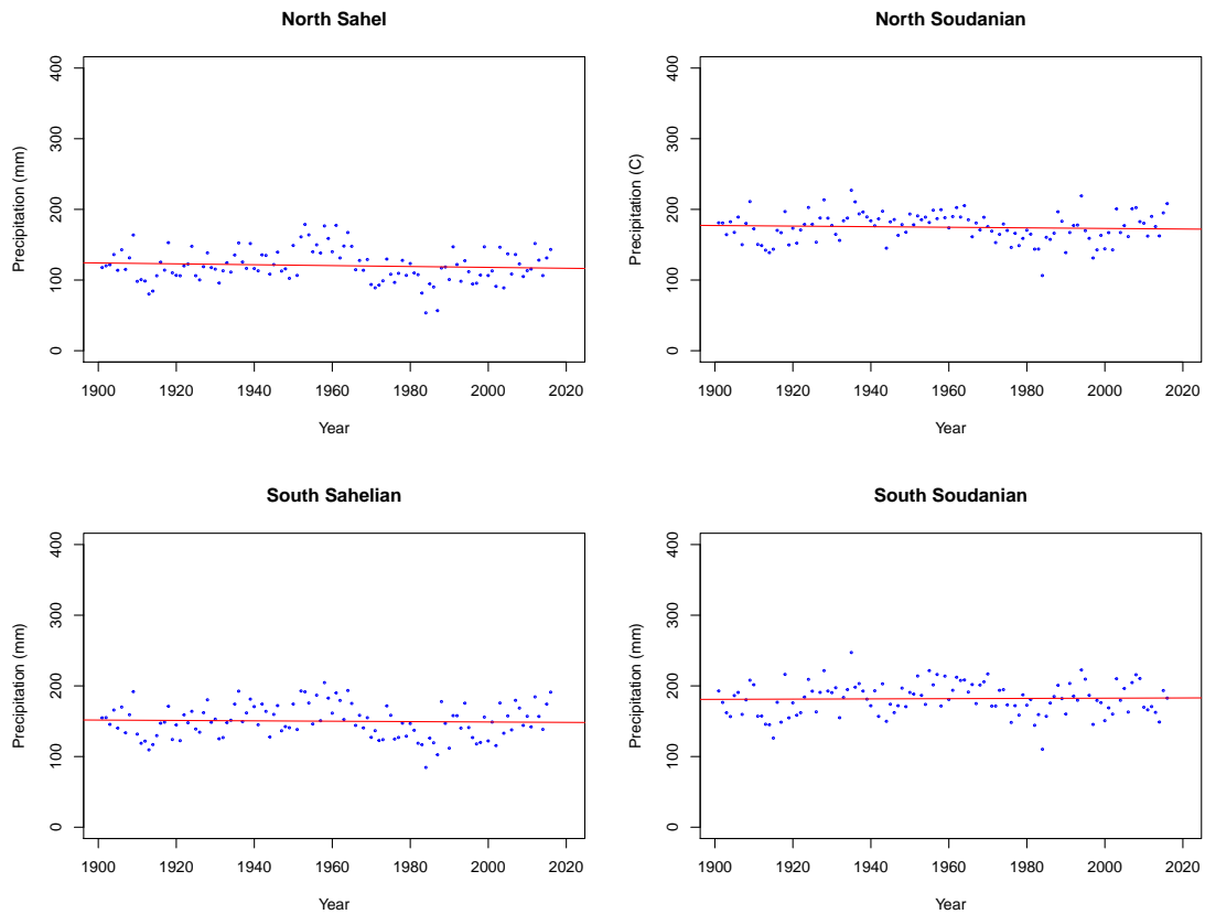
Figure 1.26 Evolution of the seasonal annual rainfall (mm) from 1901 to 2016 in the agroecological zones of Burkina Faso.
