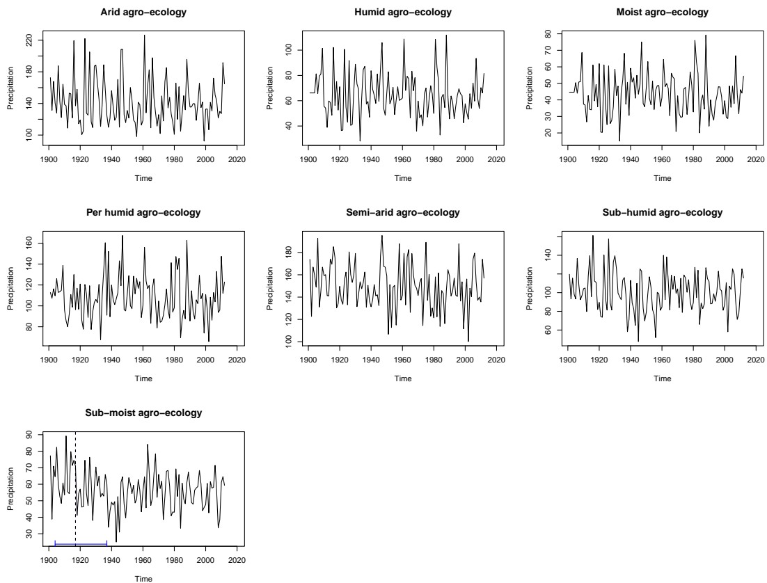
Figure 1.52 Breaks on seasonal precipitation in the agroecological zones of Ethiopia.
