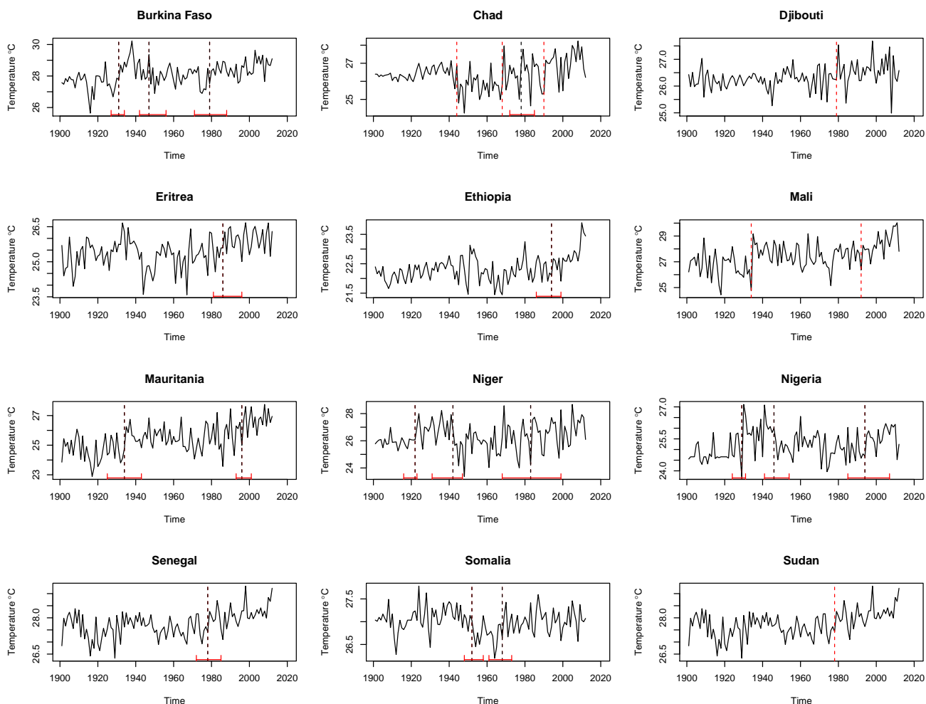
Figure 1.14 Endogenous detection of structural breaks in annual median temperature in the Sahel countries during the dry season from 1901 to 2012.
