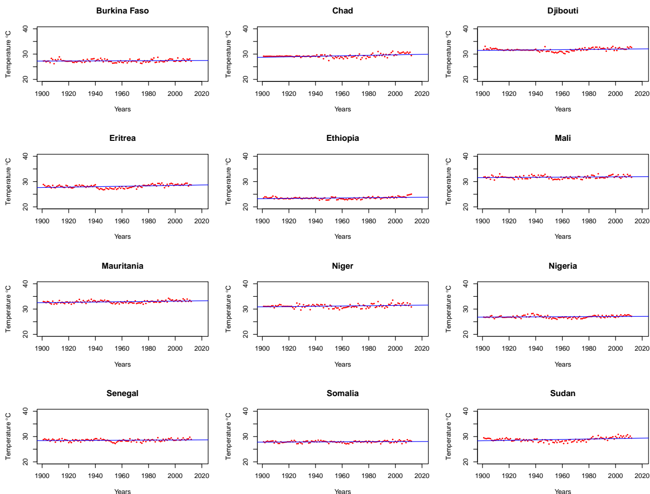
Figure 1.5 Annual median temperature during the rainy season in the Sahel countries from 1901 to 2016
