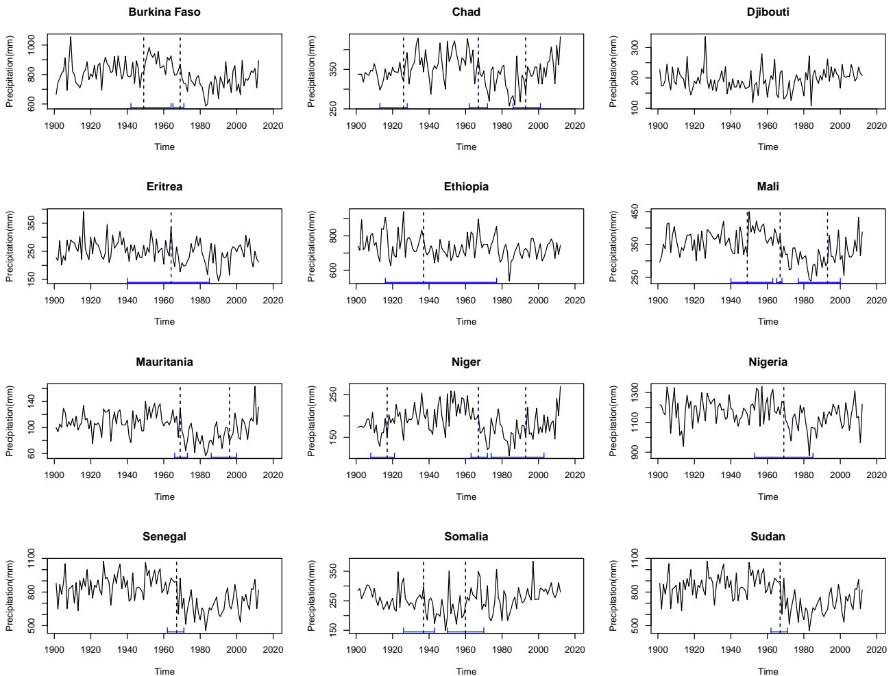
Figure 1.19 Endogenous detection of structural breaks in Total annual precipitation from 1901 to 2012 at the level of the Sahel countries.
