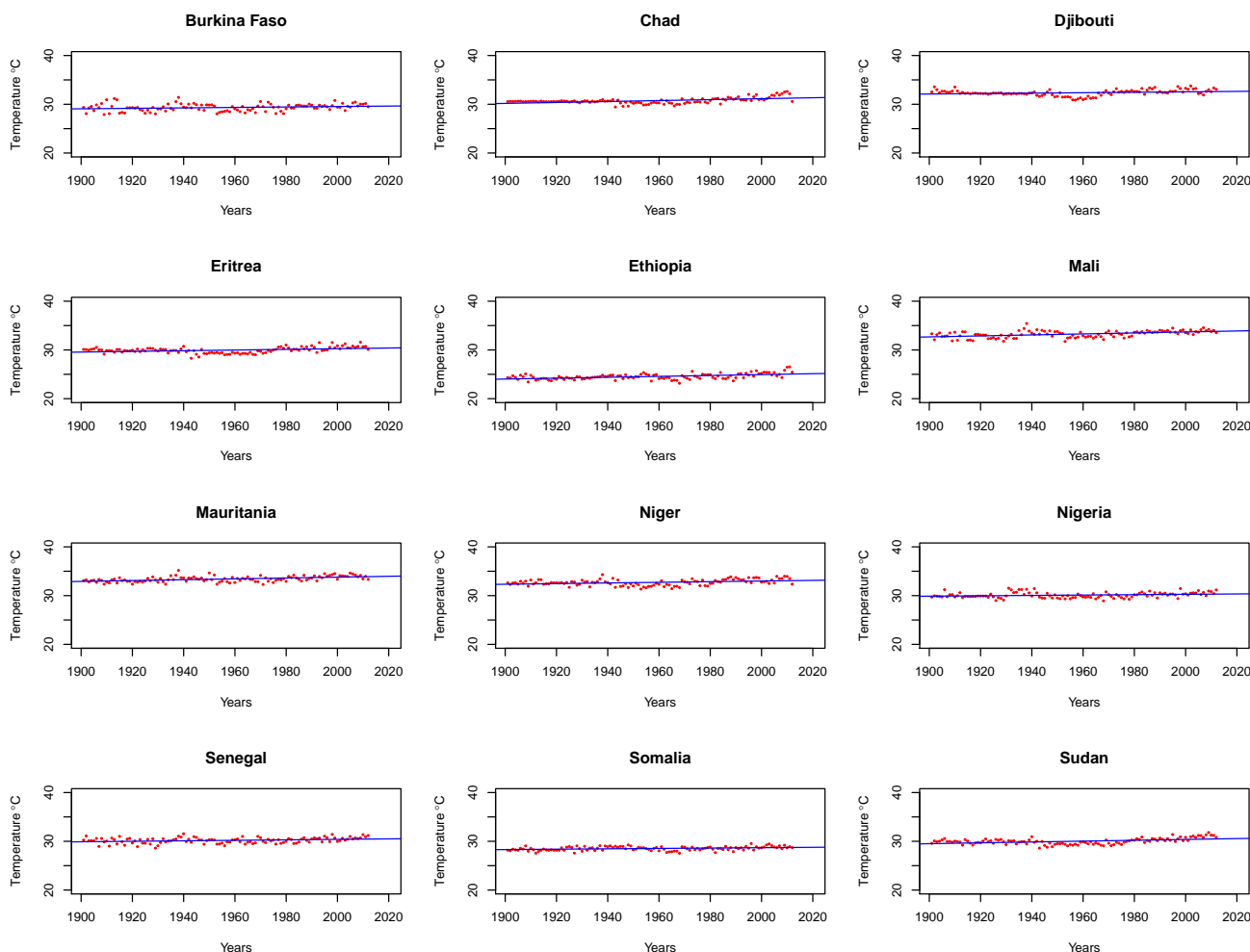
Figure 1.6 Maximum annual temperature during the rainy season in Sahel countries from 1901 to 2016
