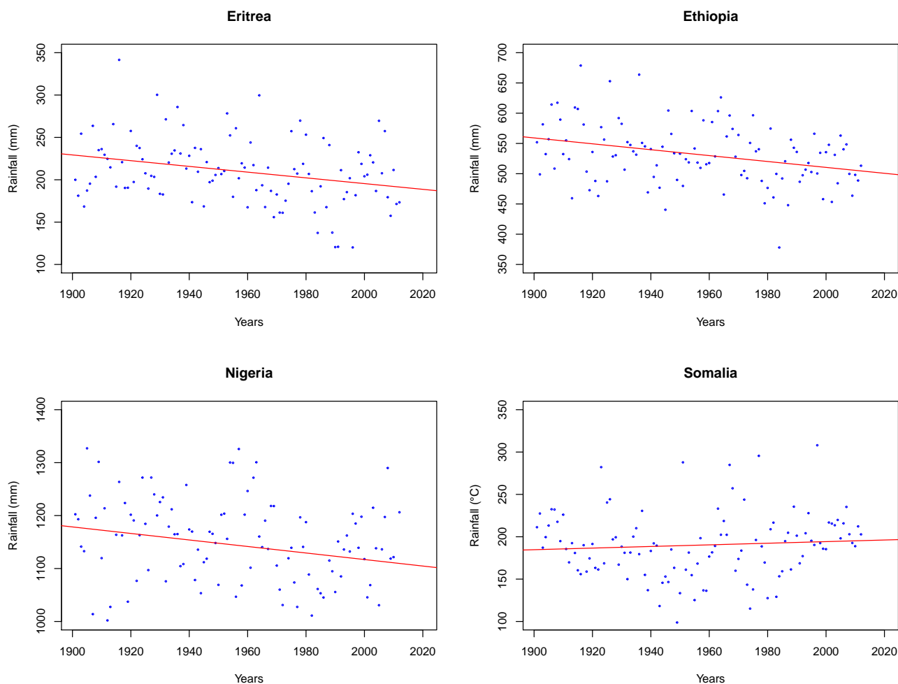
Figure 1.18 Precipitation during the rainy season for multi-season countries from 1901 to 2012
