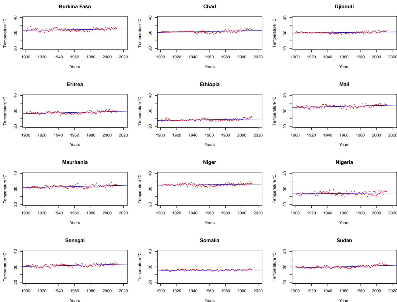
Figure 1.9 Maximum annual temperature during the dry season in Sahel countries from 1901 to 2016
