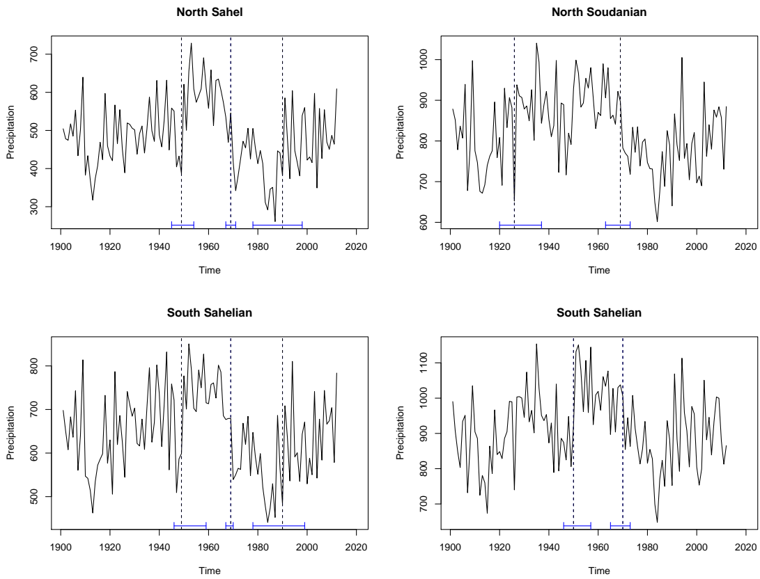
Figure 1.27 Breaks in total annual precipitation in the agroecological zones of Burkina Faso.
