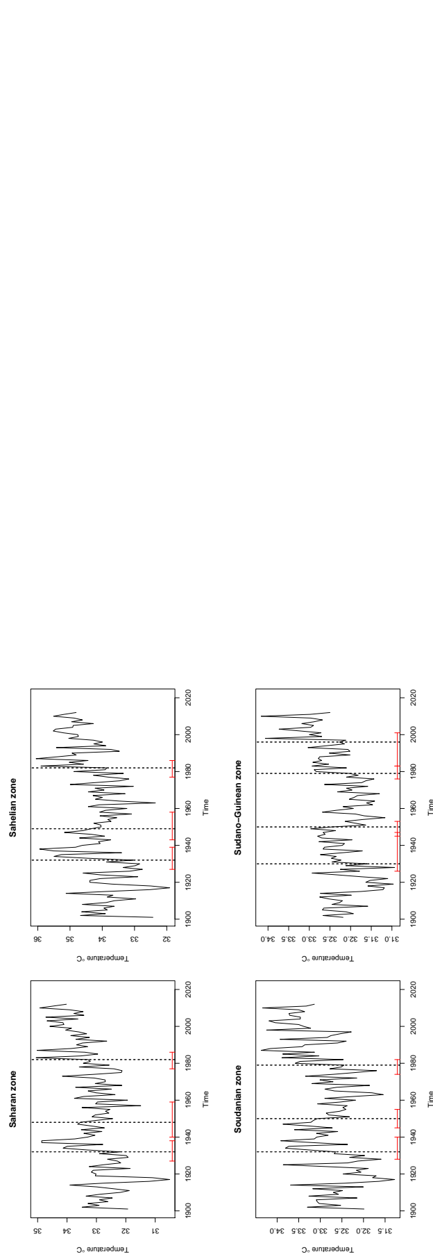
Figure 29.c: Maximum annual temperature
