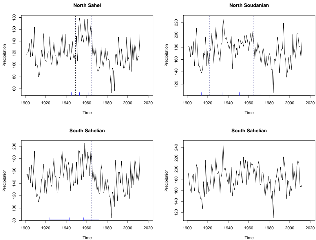
Figure 1.28 Breaks on seasonal precipitation in the agroecological zones of Burkina Faso.
