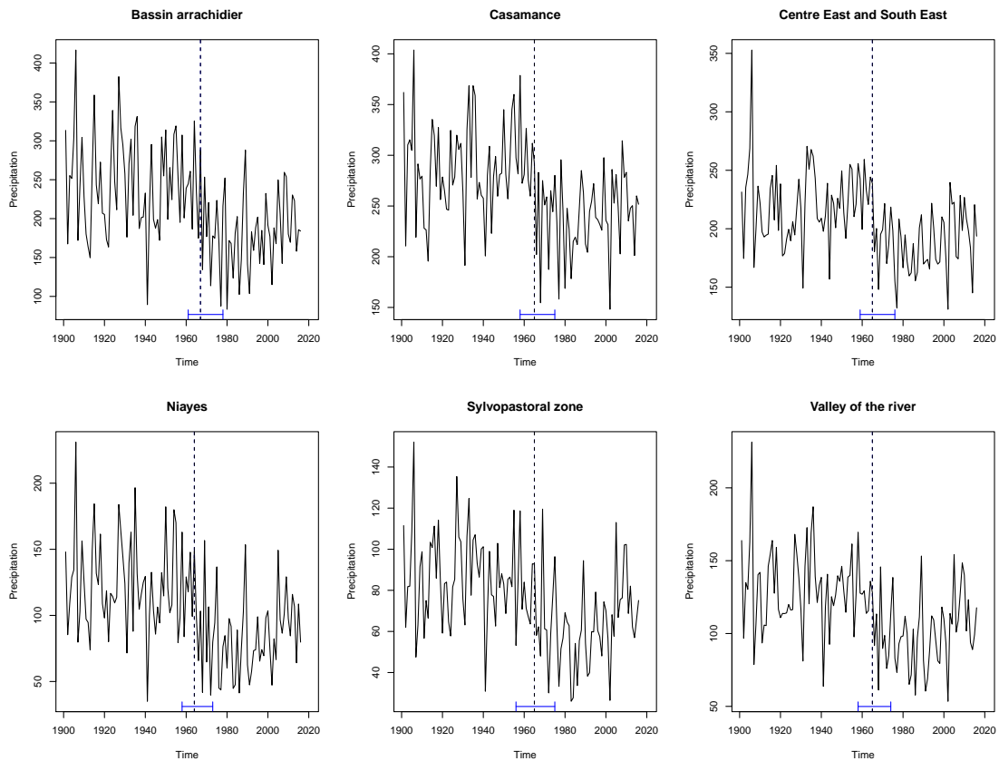
Figure 1.92 Breaks on seasonal precipitation in the agroecological zones of Senegal.
