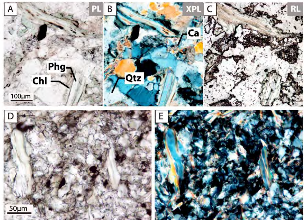
Figure 6. Thin-section pictures of mineral assemblages showing mica and chlorite crystals growing together. Chlorite (Chl), quartz (Qtz), phengite (Phg) and calcite (Ca) in CMR1 sample in (a) plane polarized light (PL), (b) cross-polarized light (XPL), and (c) reflected light (RL). Chlorite, mica, and quartz assemblage from finer fraction of CMR1 in (d) PL and (e) XPL. All the mica-chlorite couples obtained in this study originated from this finer fraction. Chlorite temperatures obtained from the different fractions are homogeneous and have similar distributions.
