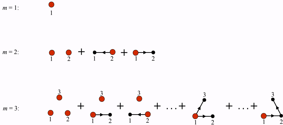
Figure 2.1: The expansion of the determinant of the matrix \bar{G} in directed spanning forests for N = 1, 2, 3 . Ellipses mean sum over the permutations of the vertices of the preceding graph. Each vertex of a directed tree, except for the root, has exactly one incoming edge and an arbitrary number of outgoing edges. The root can have only outgoing edges. A factor r_k r_j K_{kj} is associated with each edge \langle jk \rangle . A factor D_j is associated with the roots of each connected tree, which is symbolised by a red dot.
