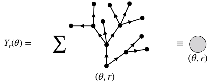
Figure 2.2: The sum over all trees growing out of a fixed root. In defining Y_r(\theta) , we have extracted a factor Lp'(\theta)r out of the weight (2.15) of the root. Thus, all vertices appearing in this diagram have the same weight.
