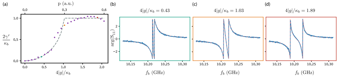
Figure 4.10: (a) Direct coupling measurement (purple square) to the readout mode as a function of the pump amplitude. We obtain the calibration for the coupling g from the fit (dashed gray line). (b) to (d) Blue solid line : phase of the measured reflection coefficient on the buffer port for various pump amplitudes. Red dashed line : corresponding curve obtained by tuning \gamma^r , which allows us to plot one dot in (a). The color of each frame corresponds to the color of its corresponding dot in figure (a).
