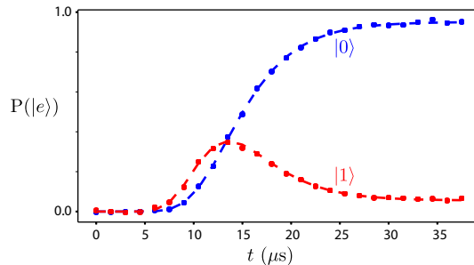
Figure 4.8: Example of photon number calibration by monitoring the readout state during decay. Squares: Measured occupation probabilities of Fock states |0\rangle and |1\rangle . Dashed lines: theory prediction with \kappa_r = 1/T_r = 250 \times 2\pi kHz and initial photon number \bar{n} = 31.8 . Red corresponds to a selective \pi pulse for 1 photon in the readout mode, blue to 0 photon.
