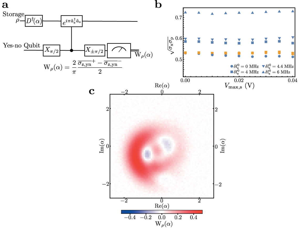
Figure 5.7: Direct Wigner tomography of the storage mode a . Circuit diagram of a Wigner tomography using a parity measurement based on dispersive interaction. After a 100 ns displacement pulse on the storage mode, an unconditional \pi/2 pulse is applied to the yes-no qubit. The qubit evolves freely during a time \Delta\tau = 337 ns \approx 1/2\chi_{s,yn} before a new \pm\pi/2 pulse is sent and the state of the yes-no qubit is measured using the readout resonator. b . Calibration of the quadrature axes for Wigner tomography. Blue dots represent the standard deviation of the quadratures of the displaced thermal equilibrium state of the storage mode as a function of drive amplitude for various detuning using the photon number calibration alone (see section 5.2.2.1). In contrast, yellow dots show the same standard deviation with the noise based quadrature calibration. c , Wigner tomography of the storage mode. Here, the mode was prepared in two steps. First, the storage mode is displaced by a pulse with an amplitude 1.7 and then the multiplexing qubit is driven at a single tone at f_{mp} - 1.4\chi_{s,mp} during 750 ns with an amplitude \Omega = \chi_{s,mp}/2 . The appearance of negative values in the Wigner function demonstrate that one can prepare non classical states in the storage mode using the multiplexing qubit backaction alone.
