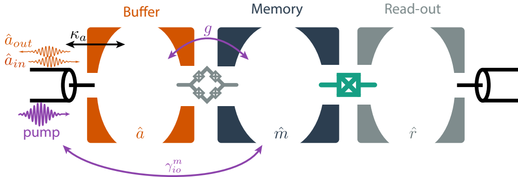
Figure 3.2: Scheme of the complete Quantum Node. The buffer resonator in orange is well coupled to the transmission line with a coupling rate \kappa_a . The buffer resonator is parametrically coupled to the high Q memory resonator in dark blue through the JRM. When a pump is applied at the difference between frequencies of the memory and the buffer \omega_p = \omega_a - \omega_m , leads to an effective coupling of the memory to the transmission line at a rate \gamma_{io}^m . The transmon qubit in green is coupled both to the memory and to a dedicated readout resonator in grey. The latter is coupled to another transmission line for the readout operations.
