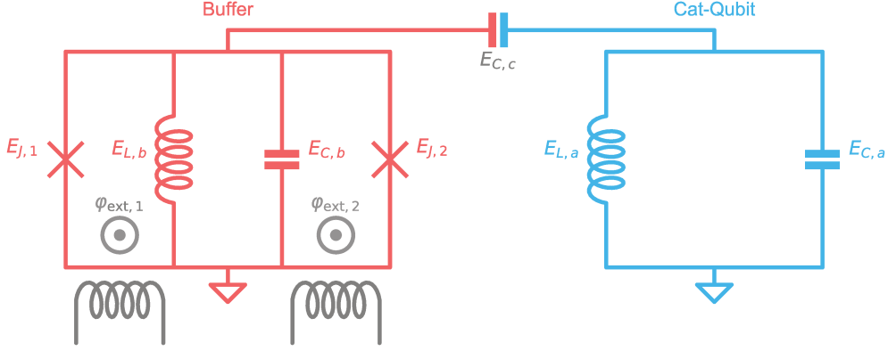
Figure 6.7: Equivalent circuit diagram. The cat-qubit (blue), a linear resonator, is capacitively coupled to the buffer (red). One recovers the circuit of Fig. 6.2 by replacing the buffer inductance with a 5-junction array and by setting \varphi_\Sigma = (\varphi_{\text{ext},1} + \varphi_{\text{ext},2})/2 and \varphi_\Delta = (\varphi_{\text{ext},1} - \varphi_{\text{ext},2})/2 . Not shown here: the buffer is capacitively coupled to a transmission line, the cat-qubit resonator is coupled to a transmon qubit
