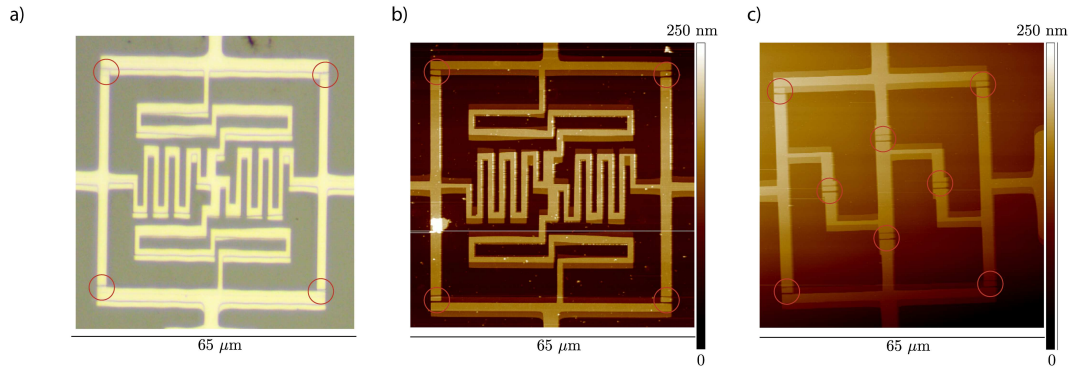
Figure 2.7: a) Microscope image of the JRM made in Al/AlO x /Al on silicon used in this thesis. The Josephson junctions are circled in red. b) AFM topography of the same JRM highlighting the junctions and the three heights due to the two steps of aluminium angle evaporation in the fabrication process. c) AFM topography of a JRM where the shunting inductances were replaced by large Josephson junctions in order to make the JRM smaller with less parasitic inductances. This design was abandoned as the shunting junctions induced unwanted non-linearity. One could reduce this effect by using a chain of larger junctions but this option was not investigated here.
