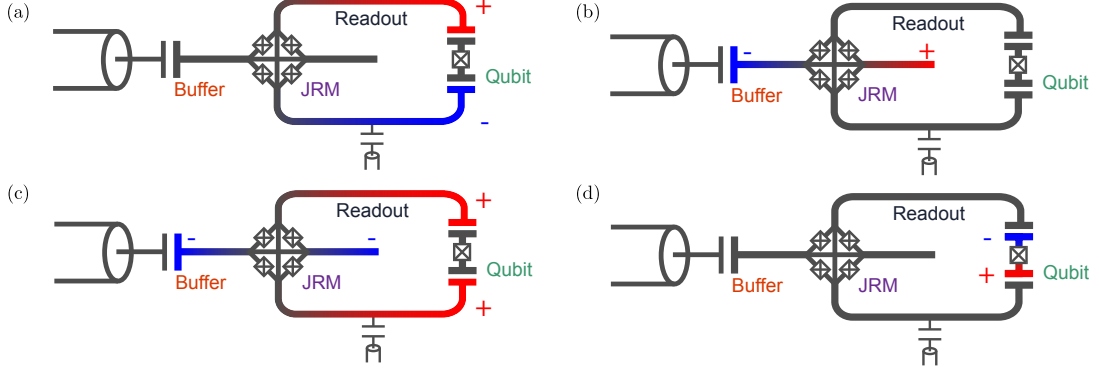
Figure 4.7: Scheme of the resonant modes that are used in the experiment. The color indicates the voltage as a function of position at maximum field amplitude in an oscillation. The readout mode (a) and the buffer mode (b) are \lambda/2 resonators. The common mode (c) extends over both CPW lines and does not couple to the transmon mode (d).
