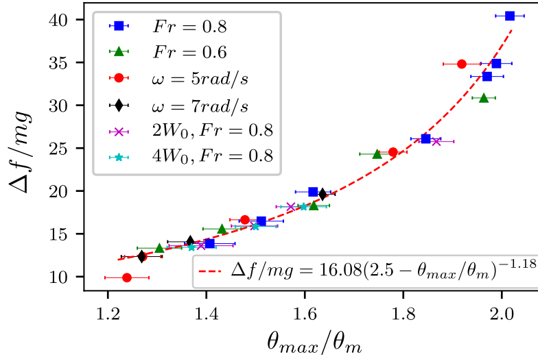
Figure 3.17 – Standard deviation \Delta f of normal force pdf's as a function of \theta_{max} / \theta_m in drums of different sizes and values of system parameters. The dashed line is a power-law fit following equation 3.7.
