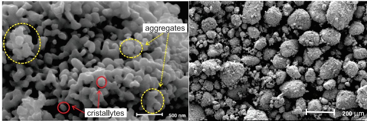
Figure 1.1 – SEM images of the \text{UO}_2 . Left: Powder microstructure, the crystallites, and aggregates can be identified. Right: Agglomerates.
