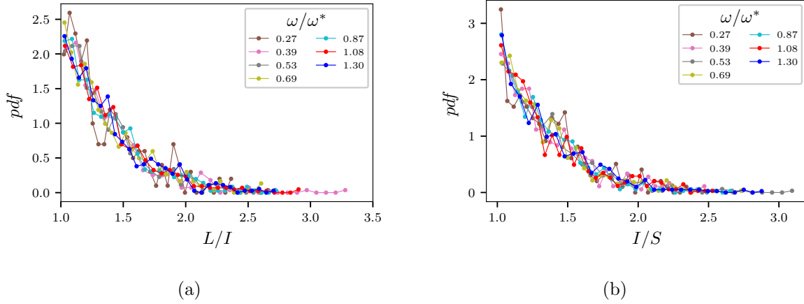
Figure A.9 – Probability density function (pdf) of the fragment a) elongation L/I and b) flatness I/S , for different impact velocities captured in the ratio \omega/\omega^* . The legend in (b) corresponds also to (a).
