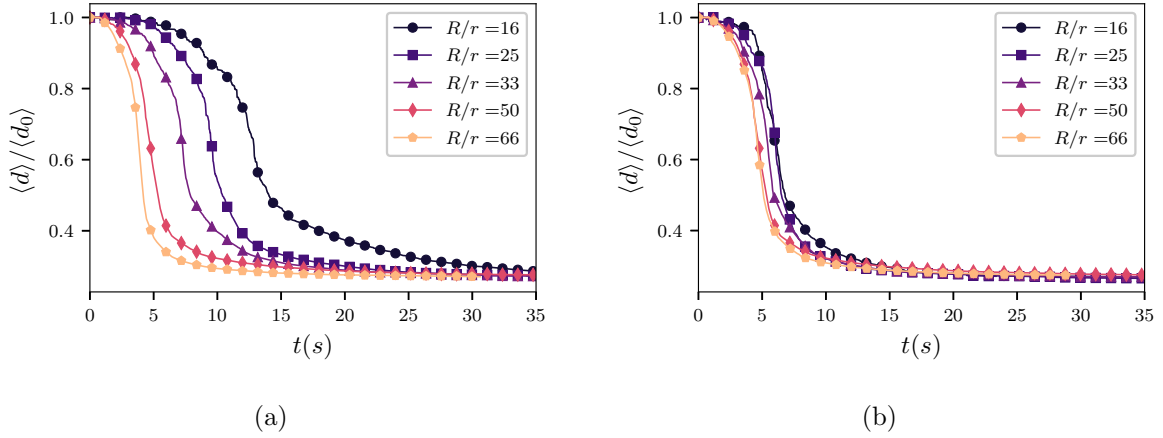
Figure 4.18 – Normalized mean particle size \langle d \rangle / d_0 as a function of time for drums of different sizes R/r for a constant value of \omega (a) and for a constant value of the Froude number (b).
