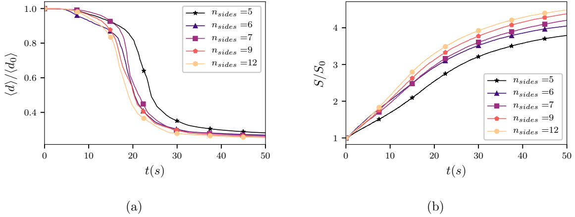
Figure 4.21 – The normalized mean particle size \langle d \rangle / d_0 (a) and normalized specific surface S/S_0 (b) as a function of time in drum flows composed of regular polygons of different numbers of sides for fixed drum size, rotation speed and filling degree.
