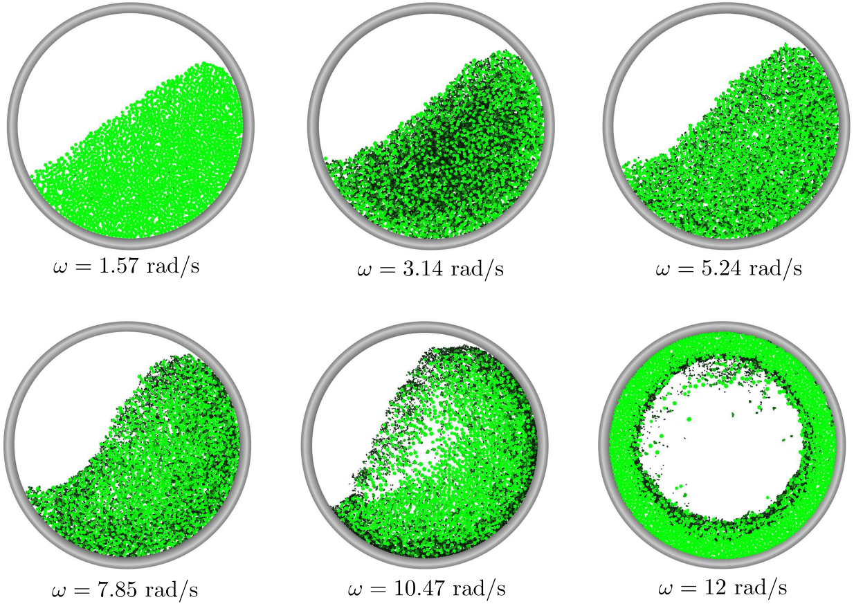
Figure 4.7 – Flow regimes displayed after 13.75 rotations, for R = 0.075 \text{ m} , f = 0.51 , and increasing rotation velocity \omega . By increasing \omega , the Froude number varies from 0.02 to 1. The color is proportional to particle damage, from bright green for intact particles to black for highly-damaged fragments.
