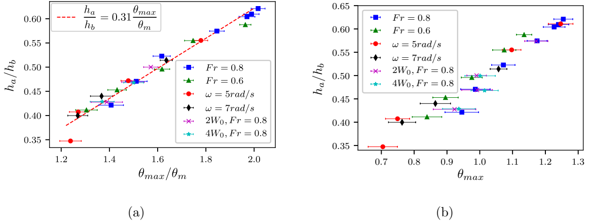
Figure 3.13 – a) Thickness h_a of the active layer normalized by the bed thickness h_b at the center of the drum as a function of \theta_{max}/\theta_m (a) and as a function of \theta_{max} (b), for simulations with different sizes at either constant Fr or \omega . The error bars represent standard deviation of the values of \theta_{max} .
