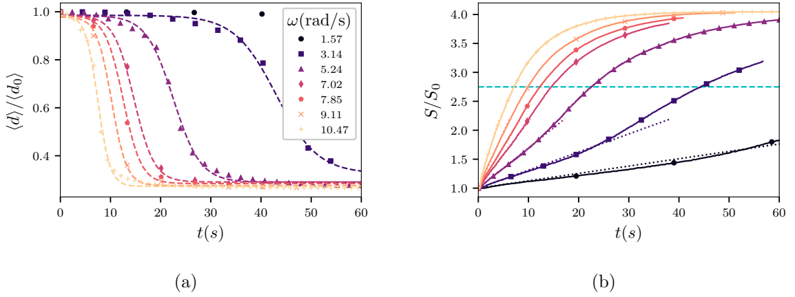
Figure 4.9 – a) Evolution of the mean particle size \langle d \rangle normalized by the initial mean particle size \langle d_0 \rangle for different values of the rotation speed \omega . The dashed lines correspond to a tangent hyperbolic form \langle d \rangle / \langle d_0 \rangle \sim \tanh(t) . b) Evolution of the specific surface S normalized by the initial specific surface S_0 . The dashed lines are linear fits up to a transition point to nonlinear regime.
