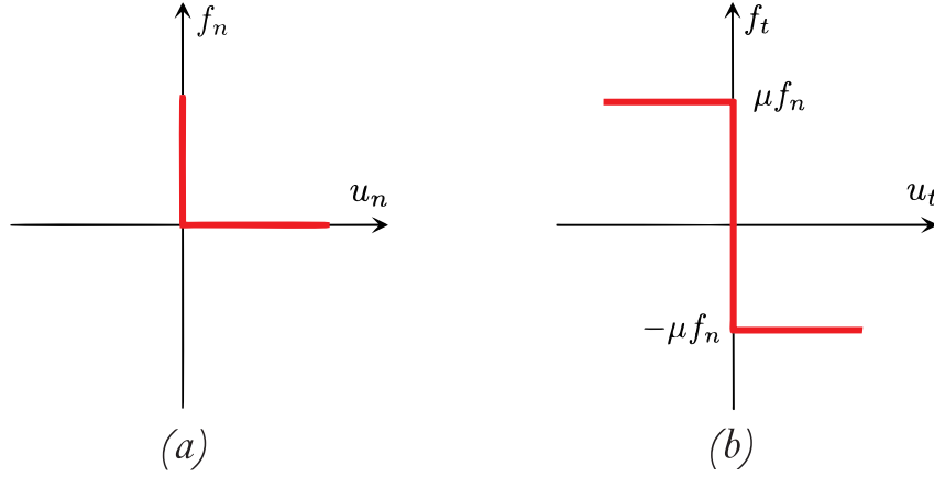
Figure 4.4 – Behavior of a purely frictional contact a) Signorini relation in the normal direction, b) Coulomb friction law in the tangential direction. u_n and u_t denote the contact relative velocities in the normal and tangential directions, respectively.
