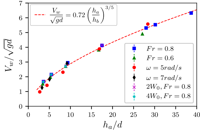
Figure 3.9 – Average speed V_w of the particles at contact with the drum wall normalized by the characteristic velocity \sqrt{gd} versus the thickness h_a of the active flowing layer normalized by particle diameter d for all simulations with different parameter values. Error bars on the data points are smaller than symbol size.
