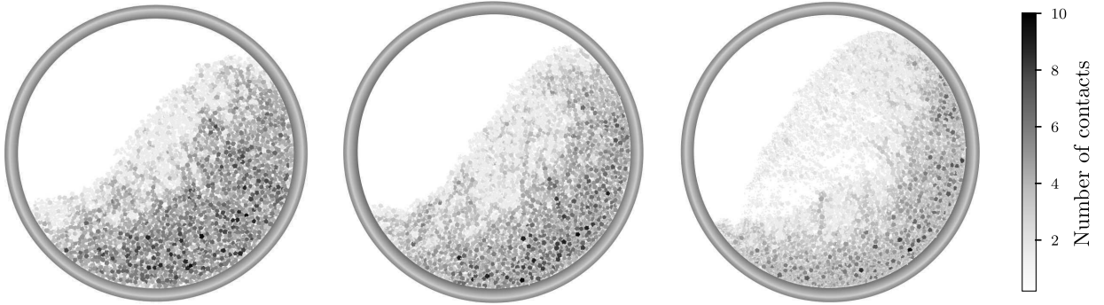
Figure 4.13 – Maps of particle connectivity after 13.75 rotations for \omega = 5.24, 7.85 and 10.47 rad/s. This snapshot corresponds to the instants 0.73t^*, 0.9t^* and 1.16t^* , respectively. The particle gray level is proportional to the number of contacts of the particle.
