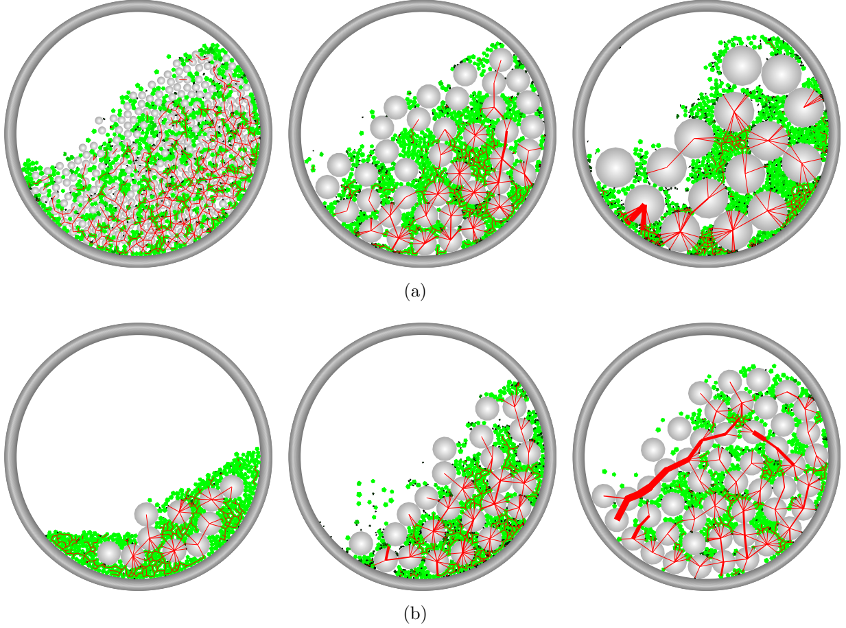
Figure 5.4 – Snapshots of several simulations: a) Systems with ball sizes D_b of 5 mm, 15 mm and 25 mm from left to right; b) Systems with numbers of balls N_b = 10, 25 and 50, with D_b = 15 mm constant. Red line thickness is proportional to normal force.
