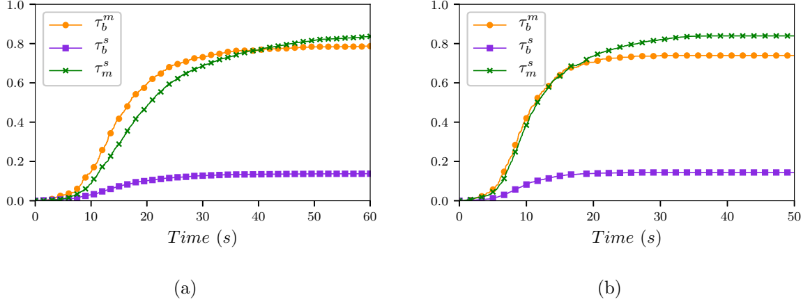
Figure 5.12 – Cumulative volume transfers: from big to small ( \tau_b^s ), from big to medium ( \tau_b^m ), and from medium to small ( \tau_m^s ), for a) D_b = 15 and b) N_b = 32 .
