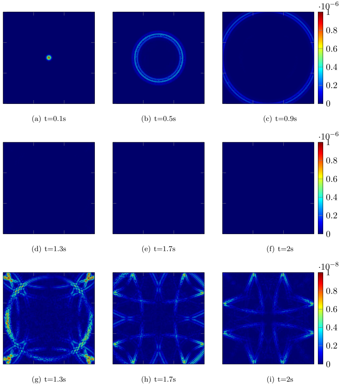
Figure 6.6: Wave propagation in an isotropic elastic domain using DGm with ABC. The three last snapshots are scaled up to see reflections at grazing incidence
