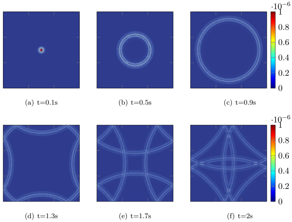
Figure 5.4: Full DGm based simulation: acoustic domain, order 3 in space, RK4 scheme in time.
