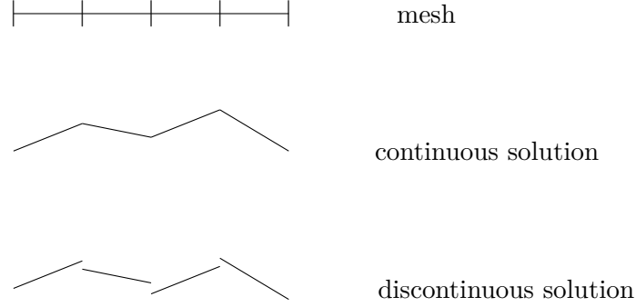
Figure 3.1: Numerical solutions on a 1D mesh (continuous and discontinuous)
