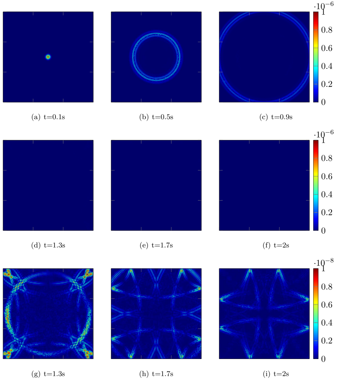
Figure 6.5: Wave propagation in an isotropic elastic domain using DG-SEm with ABC. The three last snapshots are scaled up to see reflections at grazing incidence
