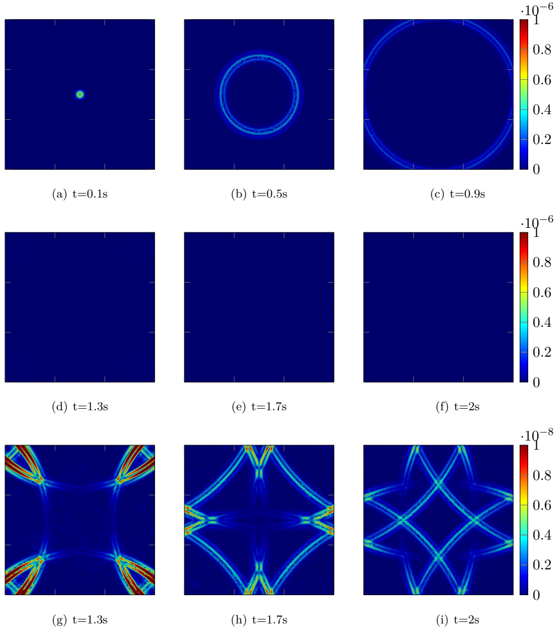
Figure 6.3: Wave propagation in a fluid domain using DG-SEm with ABC. The three last snapshots are scaled up to see reflections at grazing incidence
