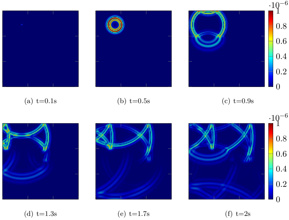
Figure 3.30: Speed modulus propagation, SEm of order 3, Leap Frog scheme, 10000 squared cells, bi-layered acoustic domain, staircase interface
