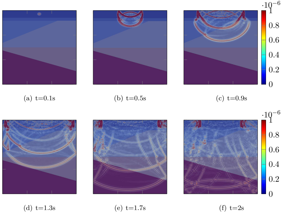
Figure 5.12: Heterogeneous domain, DGm of order 2 in the triangles and DGm of order 8 in the squares, RK4 in time.
