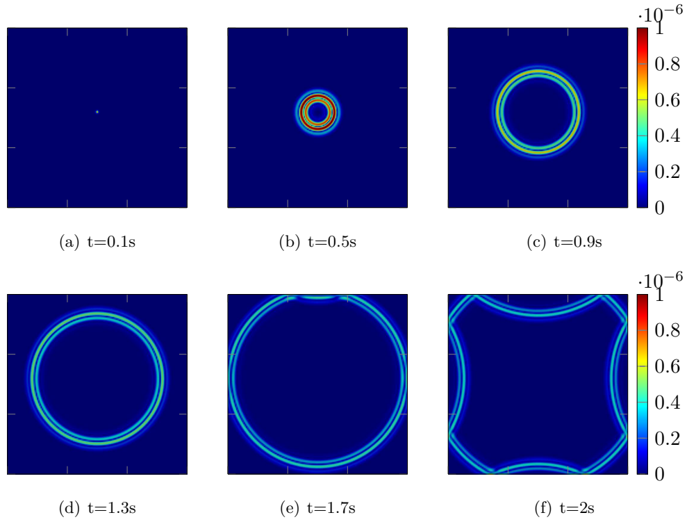
Figure 3.7: P-wave propagation in a mesh with 22500 quadrilaterals using DGm
