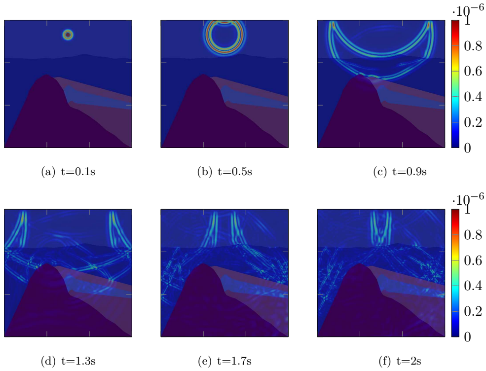
Figure 5.17: Heterogeneous domain, full DGm of order 3, RK4 in time.
