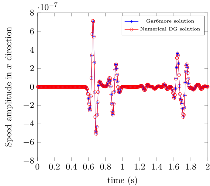
Figure 5.18: Seismograms of the reference solution (in blue) and numerical solution using DGm (in red).
