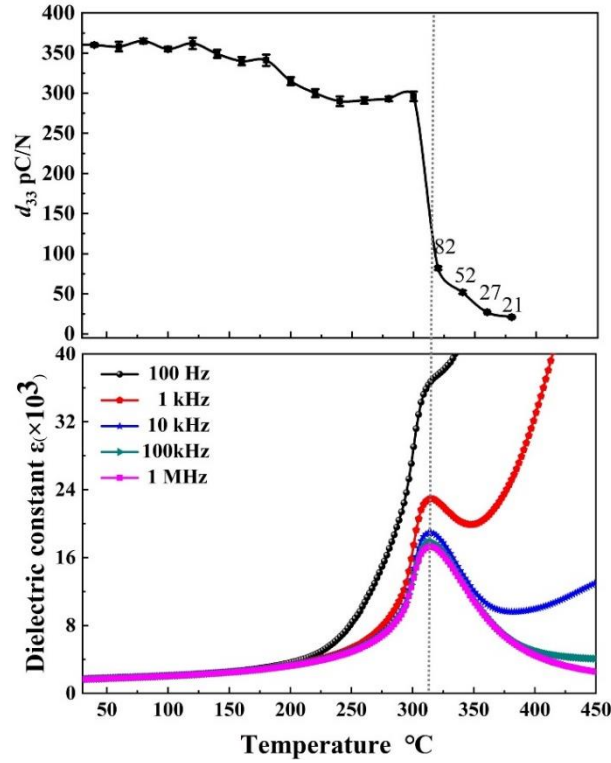
Figure 3.22 The piezoelectric constants of PSL(ZT) 0.990 -Fe 0.010 ceramics dealt with different temperatures.
