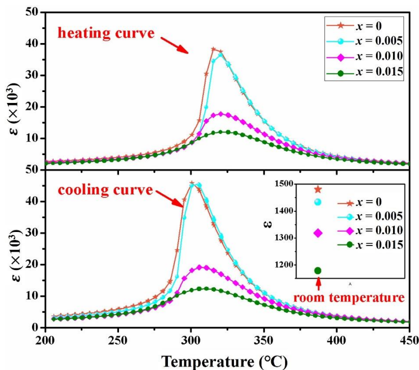
Figure 3.17 Temperature dependence of dielectric constants \epsilon of PSL(ZT) 1-x -Fe x ceramics on heating curves and cooling curves respectively.
