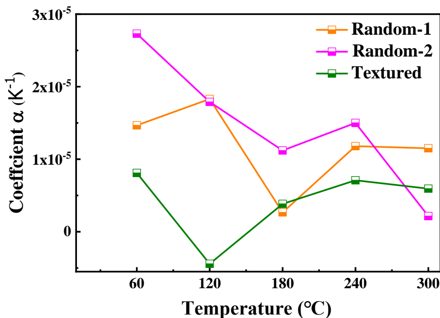
Figure 5.9 Thermal expansion of lattice parameter a as a function of temperature in random and textured BFG-BT samples
