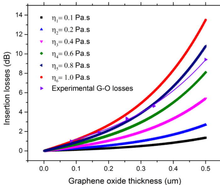
Figure 3-14 The analytical calculated attenuation coefficient versus the GO layer thickness, under different viscosity parameters and correlation between the experimental GO insertion losses (triangles) and their rheological behavior.
