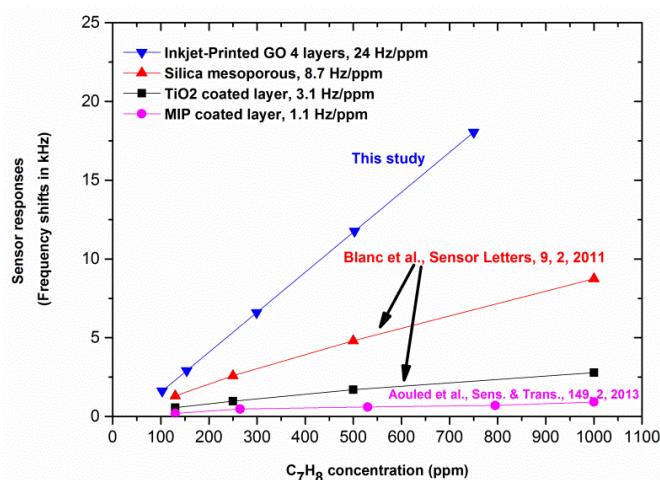
Figure 4-14 Toluene ( C_7H_8 ) comparison responses of different sensing layers such as GO (this study), Silica mesostructured [19], MIP [20] and TiO_2 [19] coated on Love wave devices.
