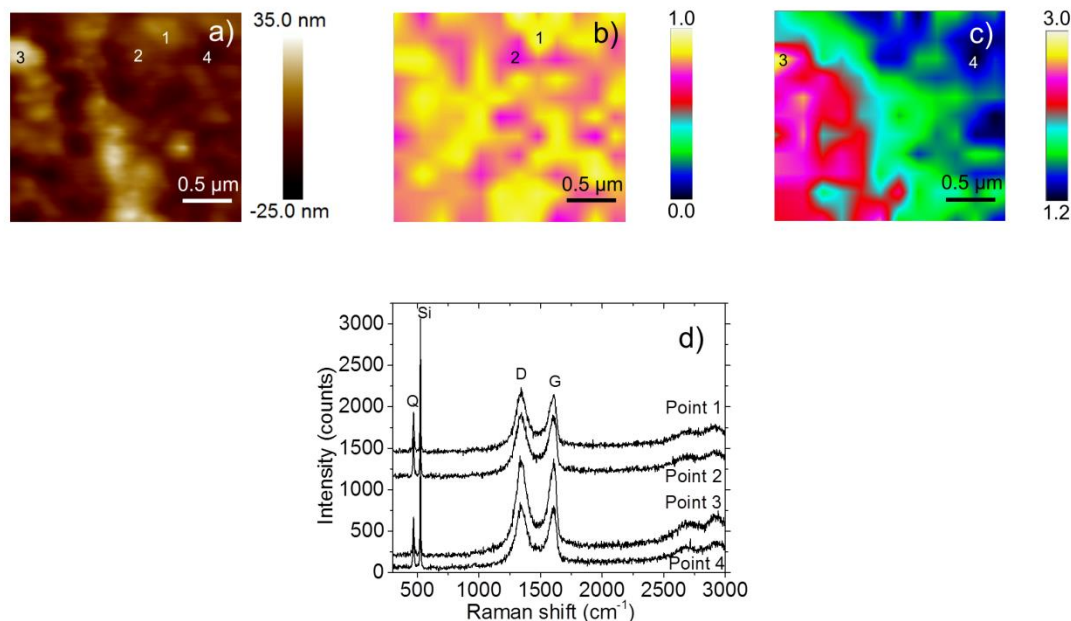
Figure 2-18 (a) Typical topographic tapping-mode AFM image of the device covered by 4 G-O inkjet-printed passes, and corresponding Raman maps showing the variation of (b) the intensity ratio ID/IG, and (c) the intensity ratio ID+G/IQ. (d) Raman spectra associated with 4 different areas (points 1, 2, 3 and 4). D and G bands assigned to G-O are indicated, as well as Q and Si bands attributed to the quartz substrate and the silicon AFM probe.
