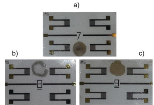
Figure 2-7 Drop-Casting deposition technique of different graphene-based materials, such as (a) Upraised-GO, (b) Graphene flakes, and (c) Standard-GO structures, respectively.
