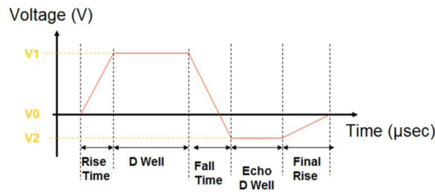
Figure 2-13 Bipolar actuation pulse of the print-head.
