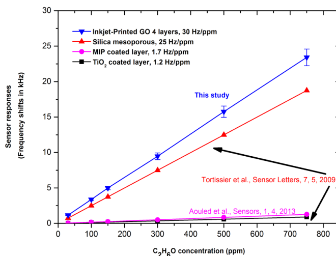
Figure 4-13 Ethanol ( C_2H_6O ) comparison responses of different sensing layers such as GO (this study), Silica mesoporous [17], MIP [18] and TiO_2 [17] coated on Love wave devices.
