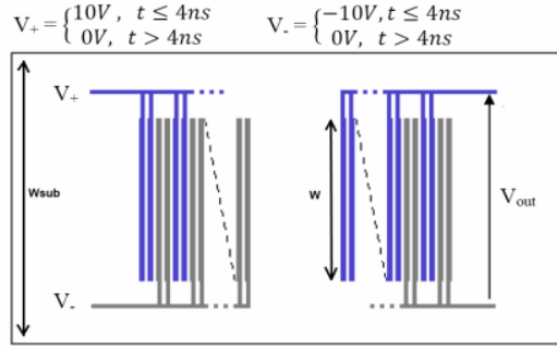
Figure 3-3 Illustration of the impulsive excitation of the emitter IDTs, and the measurement of the output voltage of the receiving IDTs.
