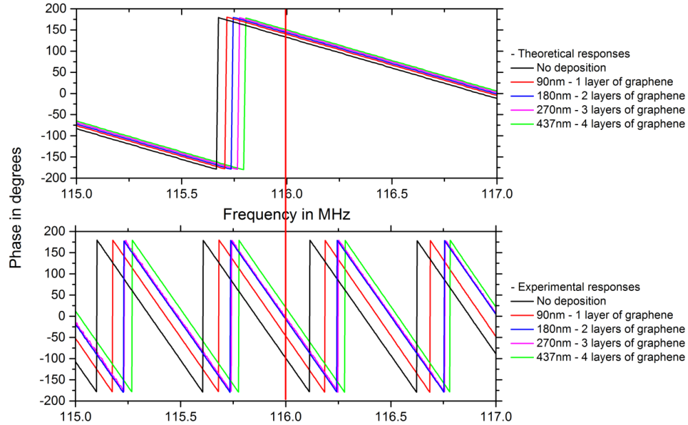
Figure 3-11 Theoretical and experimental phase of the Love wave recorded at the receiver IDTs.
