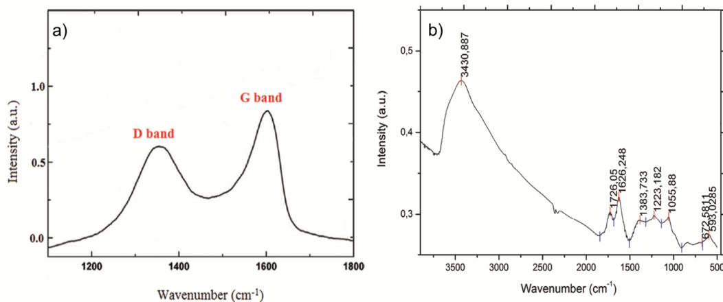
Figure 2-4 (a) Raman spectra recorded with \lambda = 514.5 nm Ar ion laser excitation source. D-G bands are indicated, and (b) Infrared Spectroscopy of GO powder. Characteristic vibrations of OH (3430 cm -1 attached heteroatoms), of COOH (1726 cm -1 ), of C = C (1626 cm -1 ) and C - O (1055 cm -1 ), respectively, can be seen.
