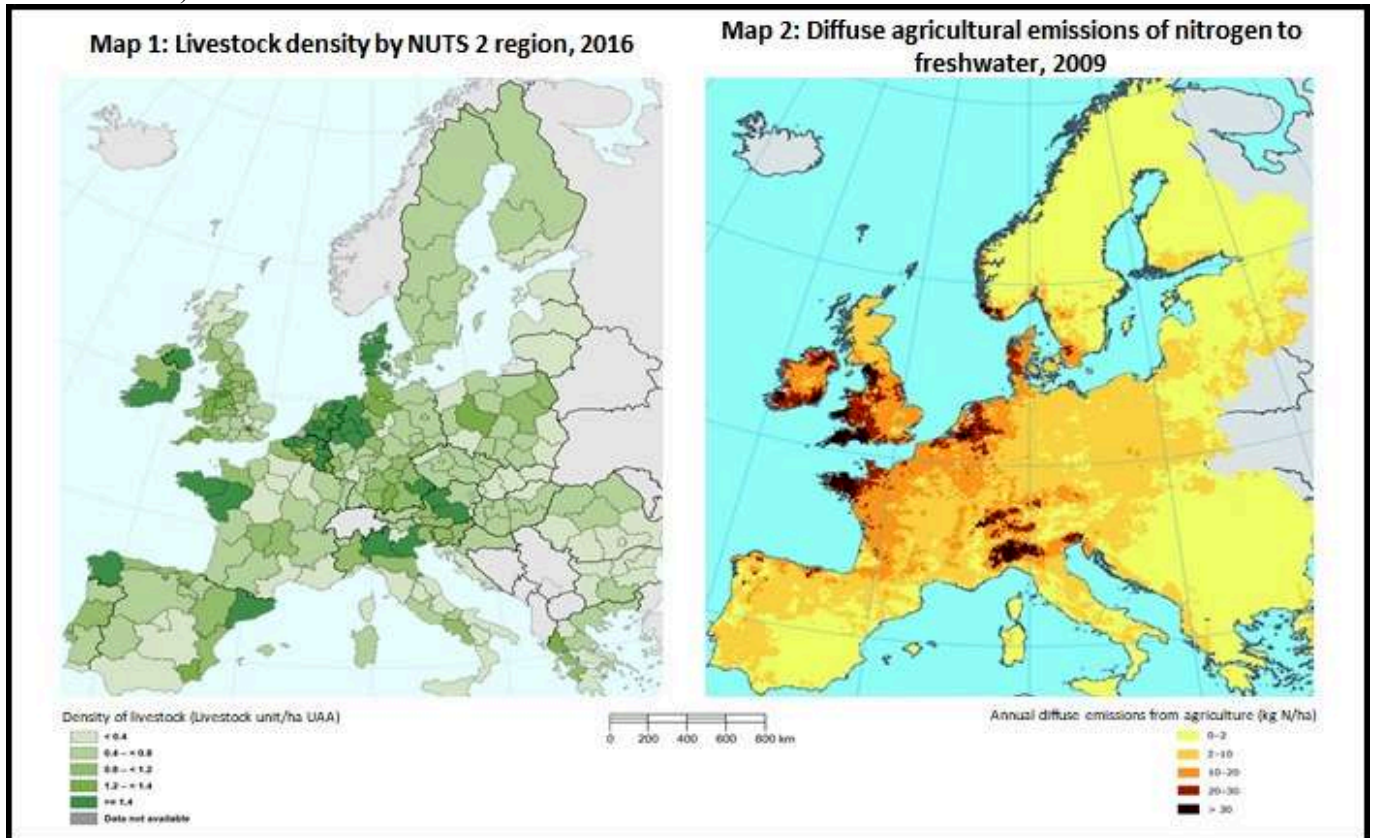
Figure B1. Livestock density in EU and modelling of agriculture N emissions to freshwater (Bouraoui et al. 2009; Eurostat 2019c)
