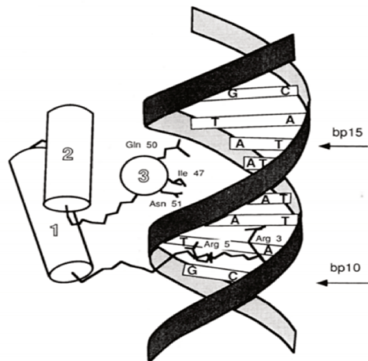
Figure 2. Homeodomain-DNA interaction
