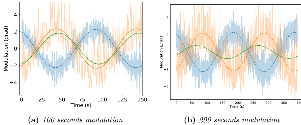
Figure 4.14: Comparison of measured amplitude for different modulation periods for the three classical sensors: Tiltmeter (yellow trace), Titan accelerometer (blue), Trillium seismometer (green).
