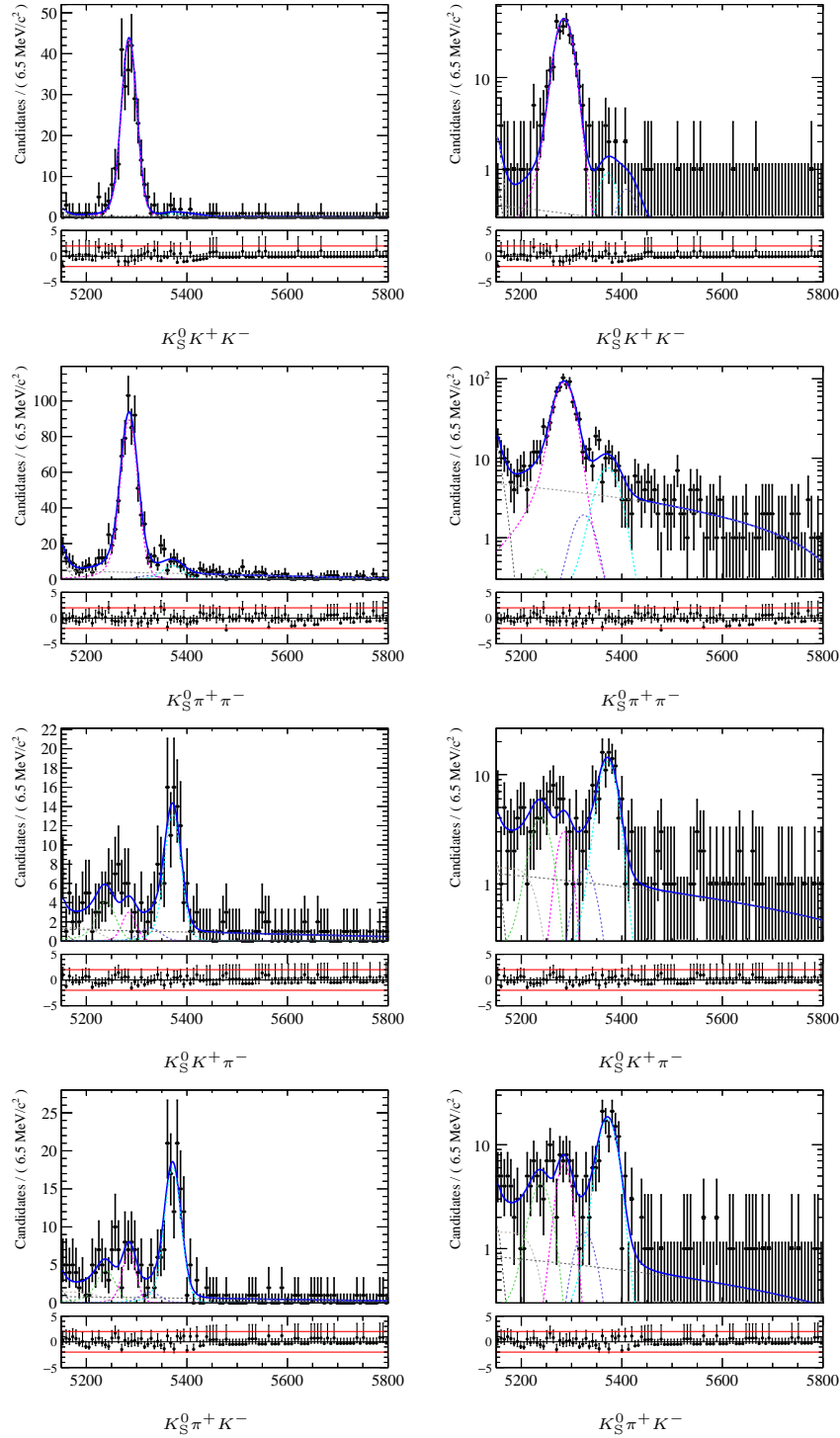
Figure B.2: Simultaneous fit to the data in the 2012b LL samples, shown on linear (left) and logarithmic (right) scales. The four spectra, K_S^0 K^+ K^- , K_S^0 \pi^+ \pi^- , K_S^0 K^+ \pi^- and K_S^0 \pi^+ K^- , are displayed from top to bottom. On each plot, the total PDF is shown in solid blue and the individual components are shown as dashed lines: the B^0 signal in pink, the B_s^0 signal in light blue, the crossfeeds from B^0 in green and those from B_s^0 in purple, the combinatorial background in grey, and the partially reconstructed backgrounds in grey to the left.
