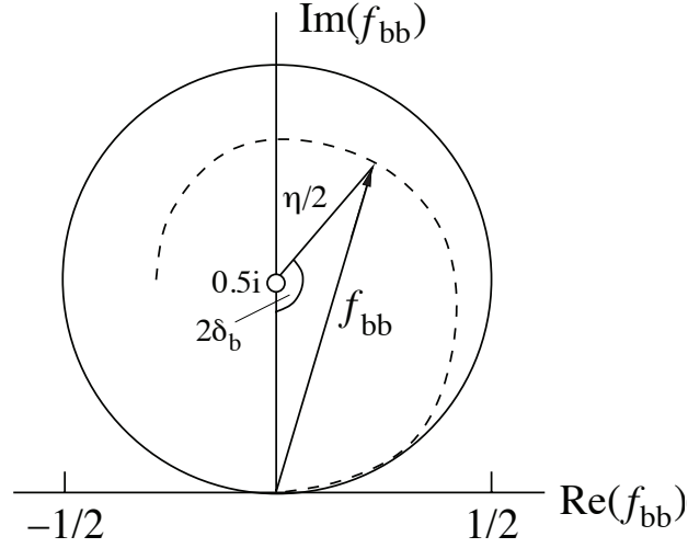
Figure III.4: Trajectory of a partial-wave amplitude, noted f_{bb} here, as a function of the energy. The unitary circle represents the case where the scattering is purely elastic ( \eta_l = 1 ) [15]. The dashed line corresponds to inelastic scattering ( \eta_l < 1 ). It clearly appears in this diagram that at \delta_b = \pi/2 the energy is real, which corresponds to the pole mass of the resonance.
