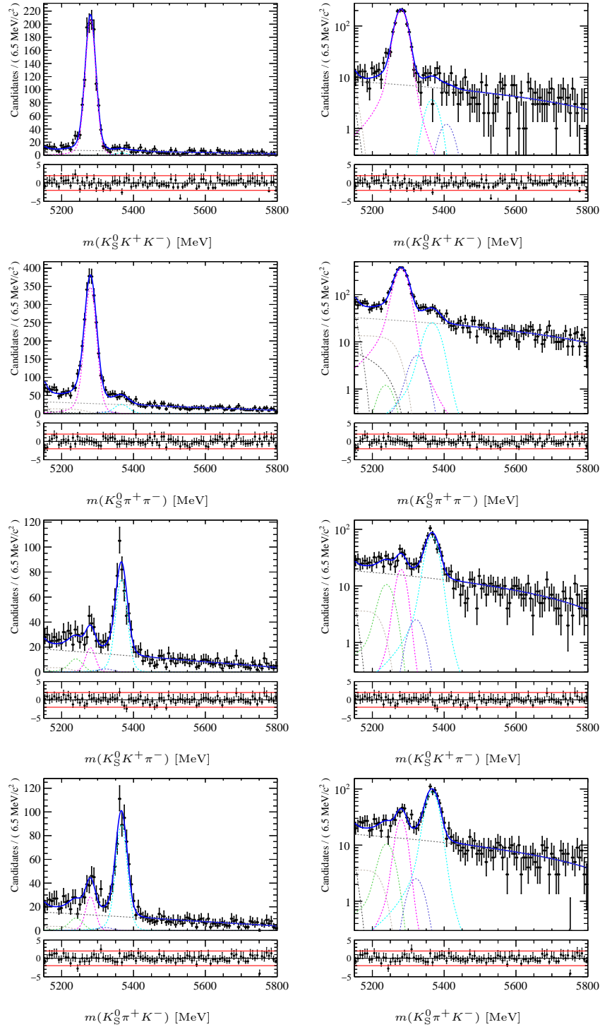
Figure VI.17: Simultaneous fit to the data in the 2016 LL samples, shown on linear (left) and logarithmic (right) scales. The four spectra, K_S^0 K^+ K^- , K_S^0 \pi^+ \pi^- , K_S^0 K^+ \pi^- and K_S^0 \pi^+ K^- , are displayed from top to bottom. On each plot, the total PDF is shown in solid blue and the individual components are shown as dashed lines: the B^0 signal in pink, the B_s^0 signal in light blue, the crossfeeds from B^0 in green and those from B_s^0 in purple, the combinatorial background in grey, and the partially reconstructed backgrounds in grey to the left.
