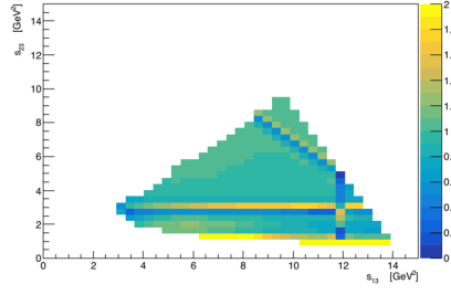
(a) \gamma = 12^\circ , \langle\alpha_{SU(3)}\rangle = 1.06
