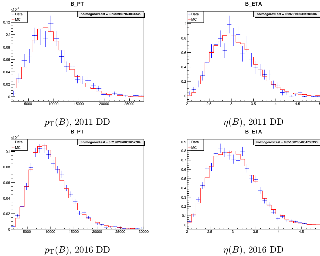
Figure VI.18: Comparison between the distributions of the p_T (left) and \eta (right) of the B meson in signal MC and s Weighted data for the B^0 \rightarrow K_S^0 \pi^+ \pi^- decay mode in 2011 (upper) and 2016 (lower) DD samples. The blue markers correspond to s Weighted data and the red curve to MC signal. Good agreement is seen between the two.
