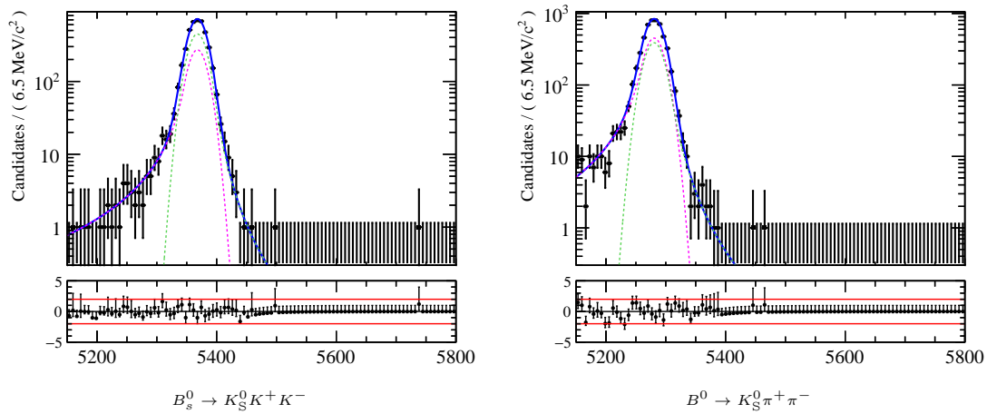
Figure VI.13: Examples of fits to the invariant mass of simulated data, corresponding to B_s^0 \rightarrow K_S^0 K^+ K^- (left) and B^0 \rightarrow K_S^0 \pi^+ \pi^- (right) signal modes. The samples were obtained with running conditions analogous to 2012b data taking period and the K_S^0 is reconstructed in the LL category. The x -axis shows the reconstructed candidate mass in MeV.
