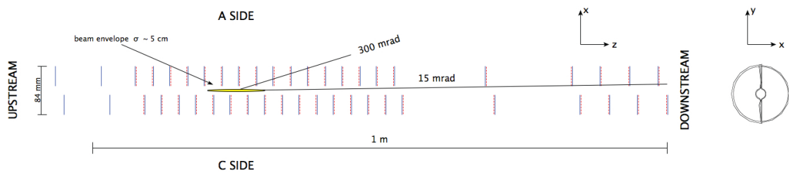
Figure V.5: View of the VELO sensors in xz plane at y = 0 in the closed position [117]. The R sensors are represented with a with solid blue lines and the \Phi sensors are shown by dashed red lines.
