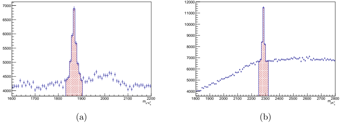
Figure VI.2: Example of vetoed peaking background in B^0 \rightarrow K_S^0\pi^+\pi^- DD sample 2016, after trigger, stripping and preselection cuts. (a) The shaded region corresponds to the veto applied on D^+ \rightarrow \pi^+K_S^0 in the \pi^+K_S^0 invariant mass. (b) The shaded region corresponds to the veto applied on \Lambda_c^+ \rightarrow pK_S^0 in the \pi^+K_S^0 invariant mass with the proton misreconstructed as a pion.
