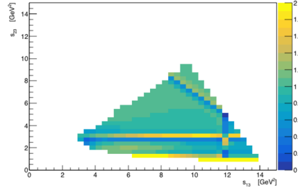
(f) \gamma = 307^\circ , \langle\alpha_{SU(3)}\rangle = 1.05
