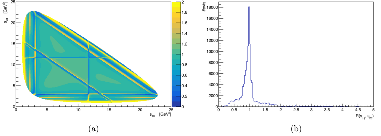
Figure IV.6: (a) Ratio of amplitudes R(s_{13}, s_{23}) over the whole fully symmetrised DP. Note that the R(s_{13}, s_{23}) scale is truncated at 2.0. (b) Histogram of the different values of the ratio of amplitudes R(s_{13}, s_{23}) .
