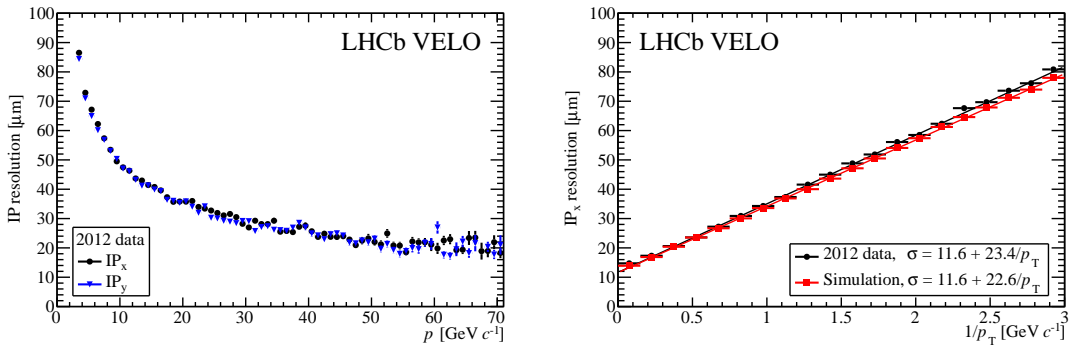
Figure V.11: (Left) IP resolution in the x and y directions as a function of the momentum, obtained from data collected in 2012. (Right) Comparison between data and simulation of the IP resolution in the x direction as a function of 1/p_T . [117].
