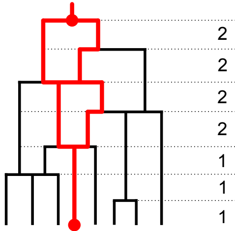
Figure 4.2: In red, the ancestry of a leaf and on the right the process counting the number of lineages in this ancestry.
