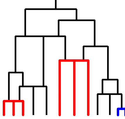
Figure 4.10: A RTCN with its only cherry (in blue) and its two reticulated cherries (in red).
