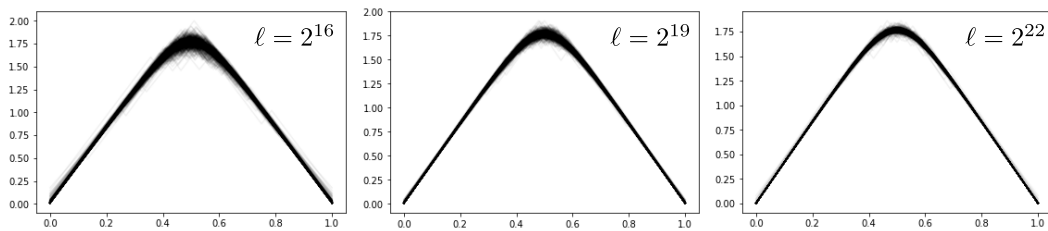
Figure 4.3: 500 superimposed trajectories of the process \tilde{X}^{(\ell)} , rescaled so that their domain is [0, 1] and that the total area under each curve is equal to 1.
