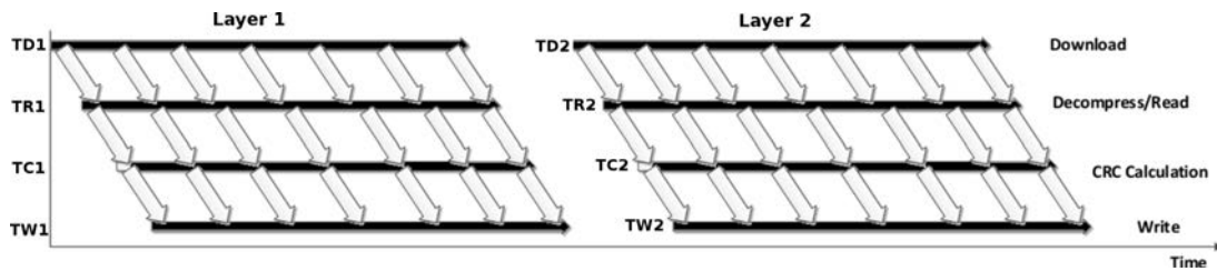
Figure 5.7 – Docker pull operation with I/O pipelining.
