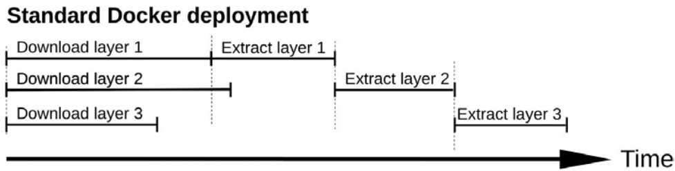
(a) Standard Docker pull with parallel layer download.
