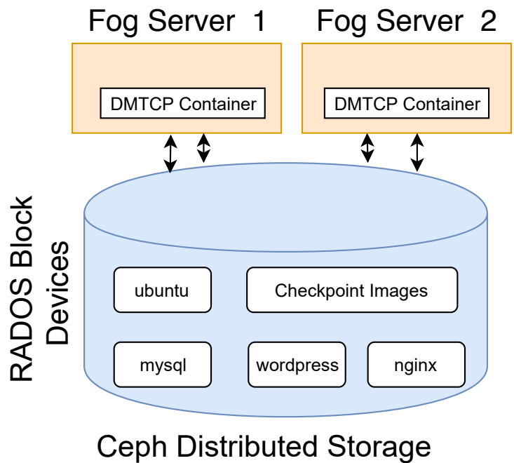
Figure 6.2 – Proposed container deployment with DMTCPC
