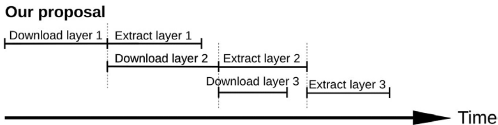
(b) Docker pull with sequential layer download.
