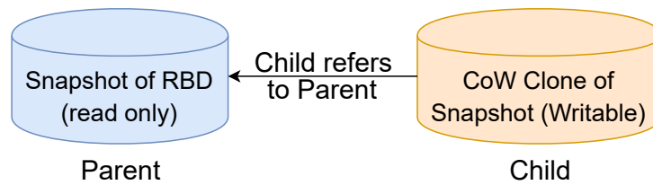
Figure 6.3 – Snapshot and clone feature of Ceph
