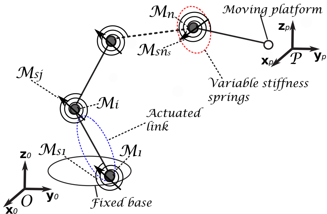
Figure 2.4: A general serial robot with variable stiffness torsional springs in parallel configuration with the links.
