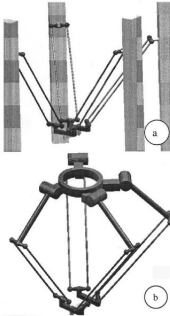
(a) H4 robot with symmetrical design [Pierrot 2001].
