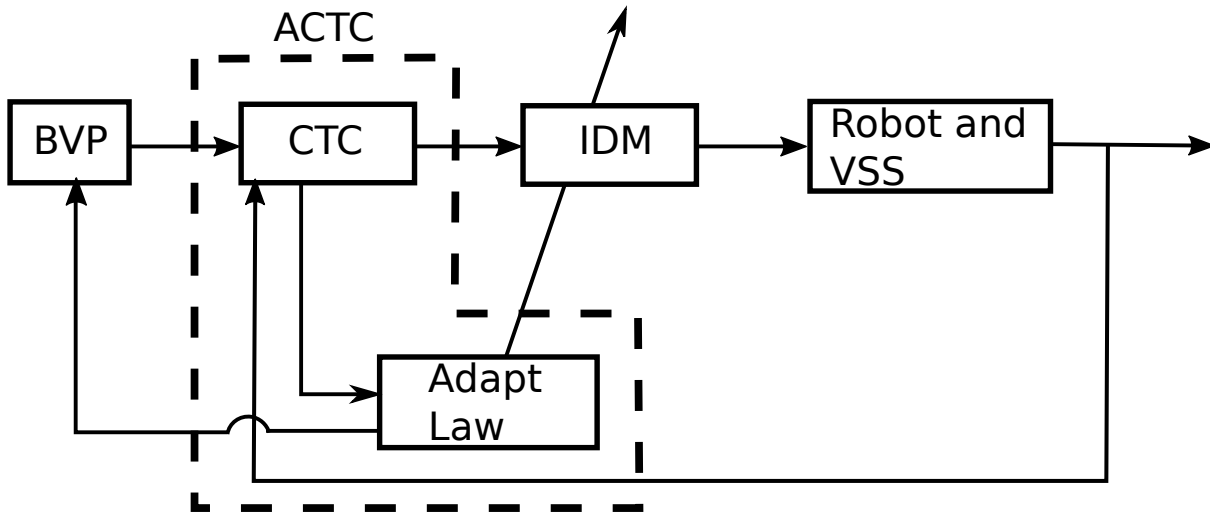
Figure 3.32: Block diagram of online solution of the BVP combined with adaptation law for dealing with dynamics uncertainties.
