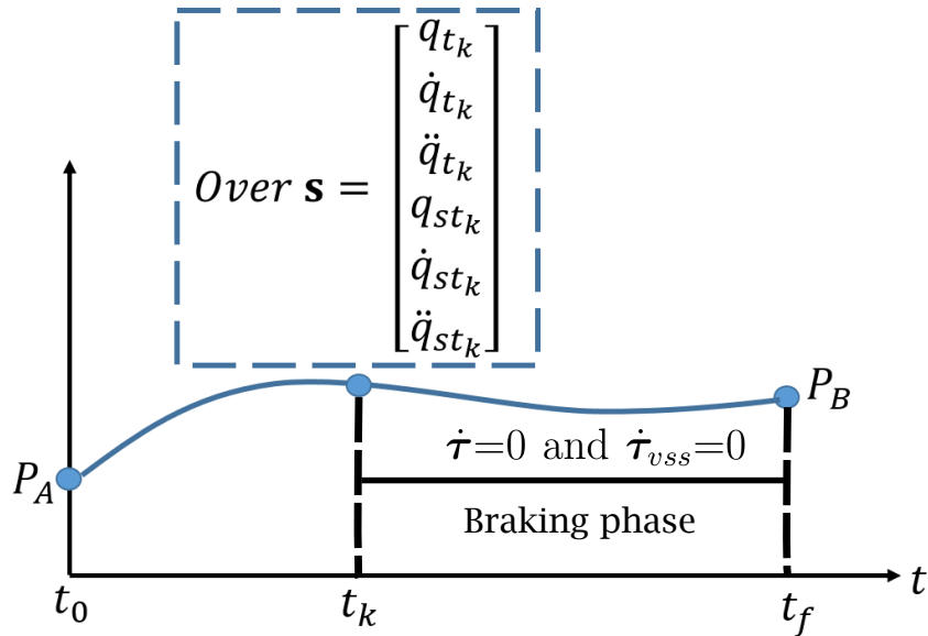
Figure 3.3: Graphical interpretation of shooting method for solving the BVP for the robot-plus-VSS system.
