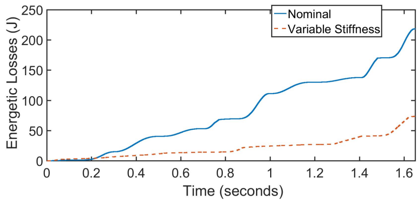
Figure 3.39: Energetic losses for the two cases compared: Nominal and by using VSS.
