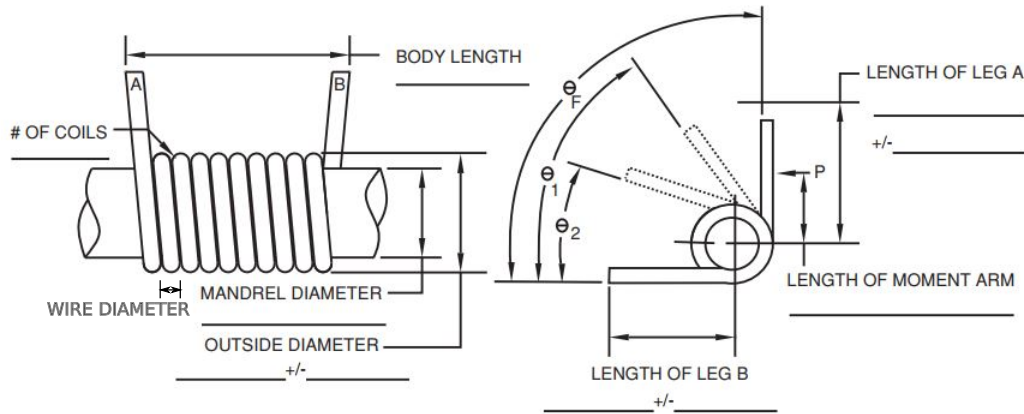
Figure 4.3: Spring schematic
