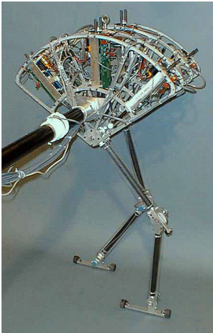
(a) Flamingo robot [Pratt 1998].
