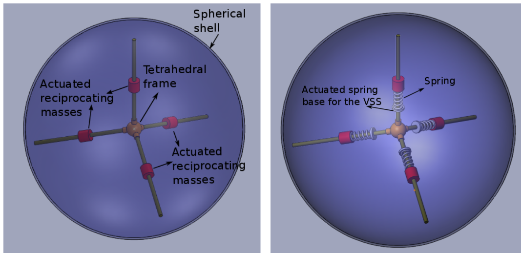
(a) Rolling robot without elastic elements (b) Rolling robot with spring/VSS
