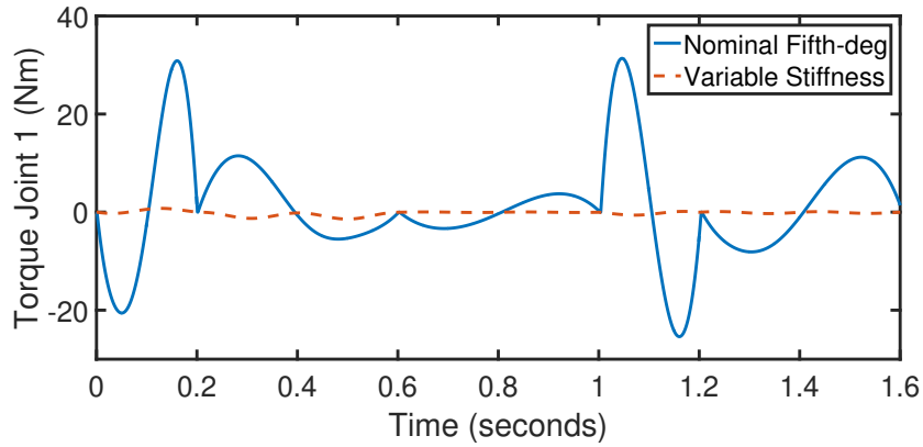
Figure 3.6: Input torques for the first joint of the parallel robot for the two cases: Nominal fifth-degree polynomial and variable stiffness with trajectories from BVP with constant payload.
