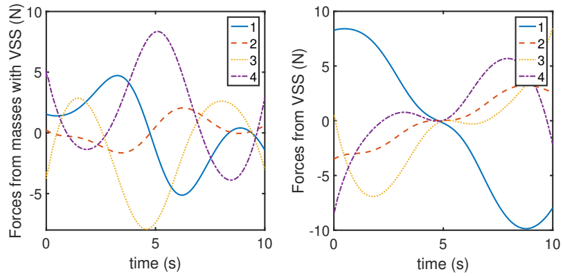
Figure 5.10: On the left the forces computed along the masses trajectories are shown when VSS are placed in parallel. On the right the forces from adjusting the VSS springs bases are shown.
