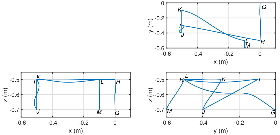
Figure 3.26: Pick-and-place sequence for the Delta robot in the three planes: G \rightarrow H (travel time: 0.12 s), H \rightarrow I (travel time: 0.06 s), I \rightarrow J (travel time: 0.1 s), J \rightarrow K (travel time: 0.06 s), K \rightarrow L (travel time: 0.1 s), L \rightarrow M (travel time: 0.08 s). The pick-and-place points are connected through the trajectories generated from the shooting method.
