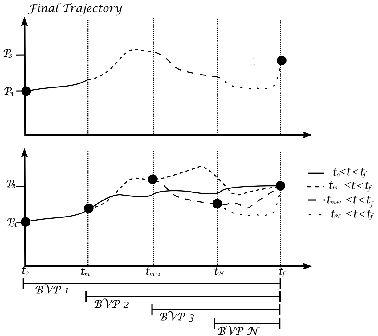
Figure 3.33: BVP solved online for generating the desired optimal trajectories within the control system.
