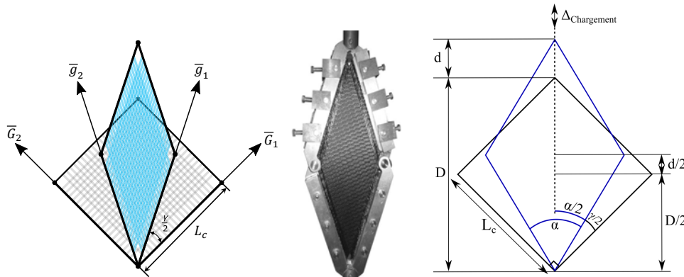
FIGURE B.1 – Picture Frame Test
