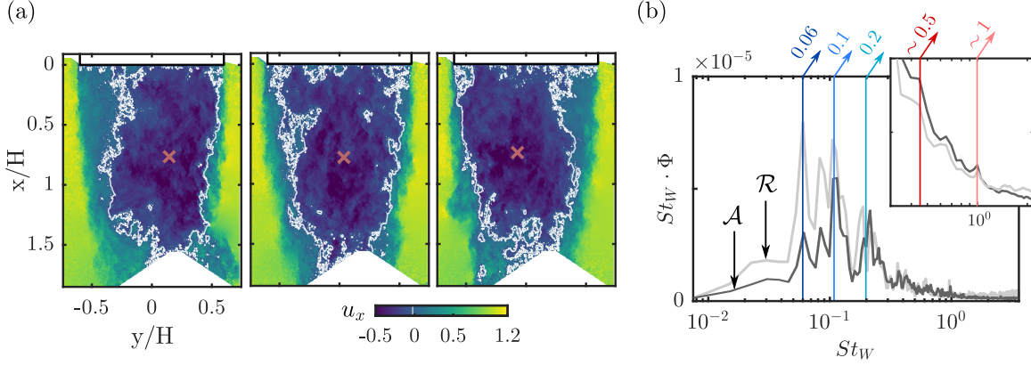
Figure 4.9: Dynamics of the recirculation region. (a) Instantaneous recirculation region in white contour and position of the wake momentum deficit barycenter indicated by the red cross. Snapshots are taken in the states L , S tr and R from left to right respectively. (b) Premultiplied spectra of the recirculation intensity \mathcal{R} and the recirculation area \mathcal{A} when the wake is locked in the asymmetric state R . Vertical arrows indicate the dominant dynamics.
