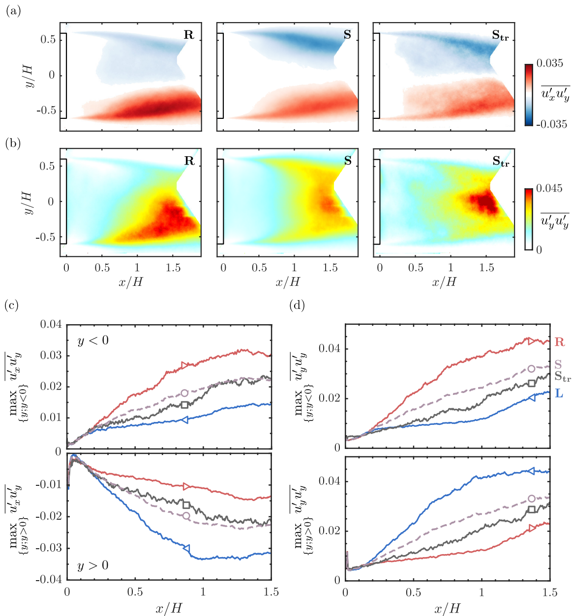
Figure 4.7: Conditionally-averaged mean Reynolds stresses for the different wake states. (a) Streamwise-lateral component \overline{u'_x u'_y} and (b) lateral-lateral component \overline{u'_y u'_y} . (c,d) Streamwise profiles of maximum of Reynolds stresses \overline{u'_x u'_y} and \overline{u'_y u'_y} for each side of the wake ( y > 0 or y < 0 ). See the details in the text for the exact definition of the velocity fluctuations for each state.
