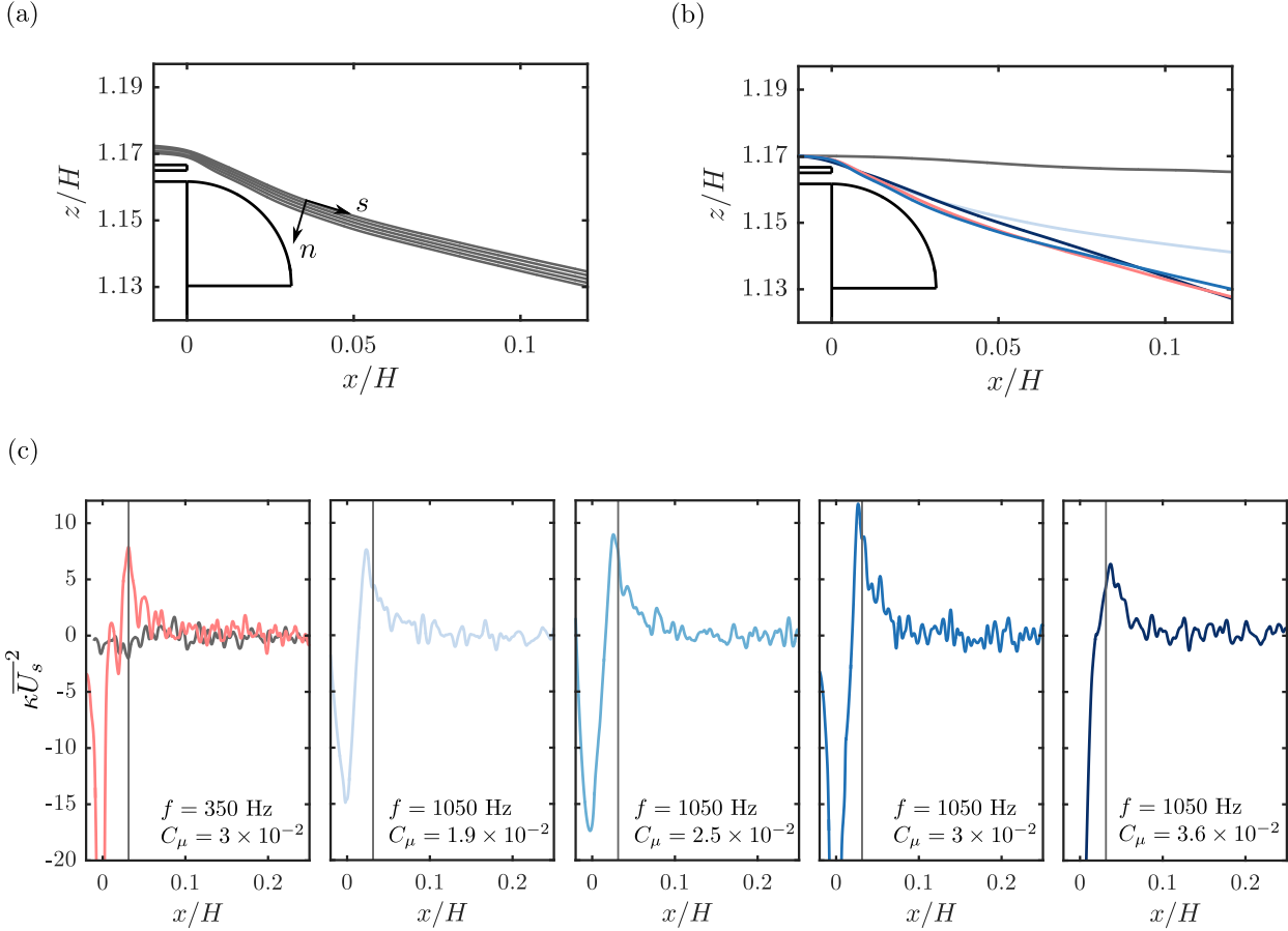
Figure 5.13: Streamwise evolution along the separating streamline of the normal pressure gradient \frac{\partial p}{\partial n} related to curvature obtained from equation 5.17. (a) Example of an ensemble of 5 streamlines originating around z \sim G + H + \theta used for averaging the curvature \kappa and the normal pressure gradient \frac{\partial p}{\partial n} estimation. (b) Separating streamlines originating from the same point for unforced and various forced cases. The colours are defined the same as in (c). (c) Streamwise evolution of the normal pressure gradient estimated from the curvature part of equation 5.17 for forcing at f = 350\text{ Hz} and C_\mu = 3 \times 10^{-2} , and at f = 1050\text{ Hz} and C_\mu = \{1.9, 2.5, 3, 3.6\} . The unforced case is additionally shown in grey in the first graph. Thin vertical grey lines indicate the streamwise extent of the curved surface.
