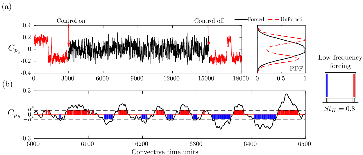
Figure 1.13: Closed-loop control of lateral bi-stability in the wake of an Ahmed body (adapted from Li et al. (2016)). Forcing is provided by pulsed jets at low frequency ( St_H = 0.8 ) from the lateral edges of the base. The forced edge is chosen based on the detection of the sign of the lateral pressure gradient at the base of the model C_{py} as shown in (b). This control strategy leads to a relative symmetrisation of the wake (see (a)), but the associated drag reduction is quite small (less than 2 %) because of the enhancement of the shear layer activity by the low frequency forcing.
