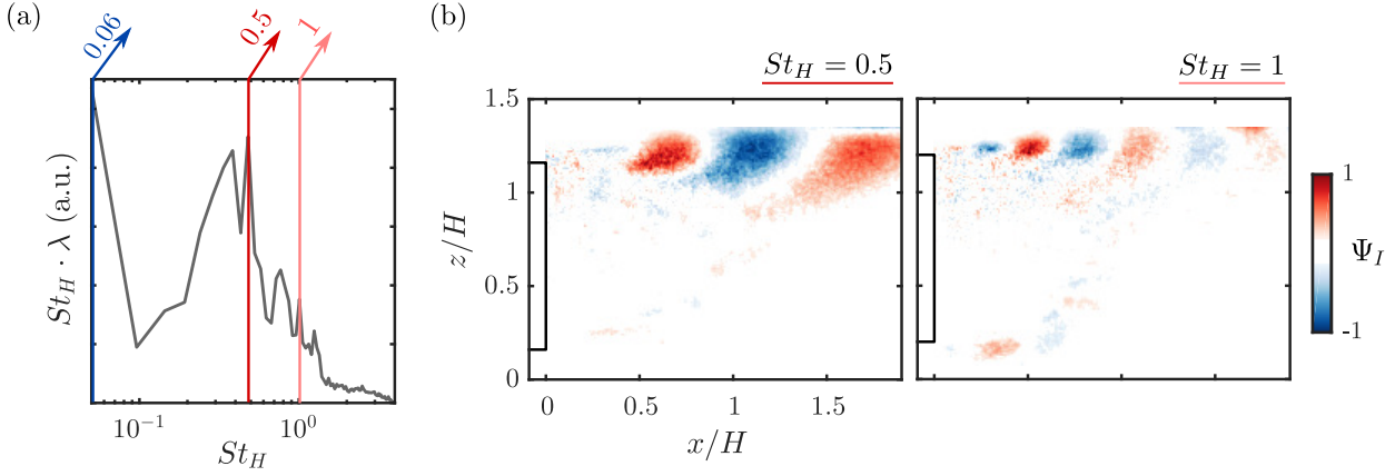
Figure 4.14: Spectral proper orthogonal decomposition (SPOD) of the light intensity field for the Ahmed body wake flow at low Re_H \sim 9 \times 10^3 locked in a vertical asymmetric state B . (a) Premultiplied spectrum of the first SPOD modes \lambda_{St_H}^{(1)} . Dominant dynamics are highlighted by colored vertical arrows. (b) Spatial organization of the dominant dynamics shown by first mode at the given frequency \psi_{St_H}^{(1)} .
