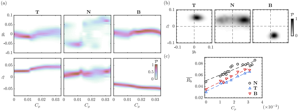
Figure 6.7: Effect of global forcing F_{TBLR} on the base pressure for T , N and B configurations. (a) Sensitivity maps of the CoP position y_b and z_b to forcing amplitude C_\mu . (b) P.d.f. \mathcal{P}(y_b, z_b) of the CoP at maximal base pressure recovery ( C_\mu = 0.024 for N , C_\mu = 0.034 for T and C_\mu = 0.031 for B ). (c) Evolution of the mean wake asymmetry \overline{R}_b = \sqrt{y_b^2 + z_b^2} with C_\mu . Dashed lines indicate linear fits to the evolution.
