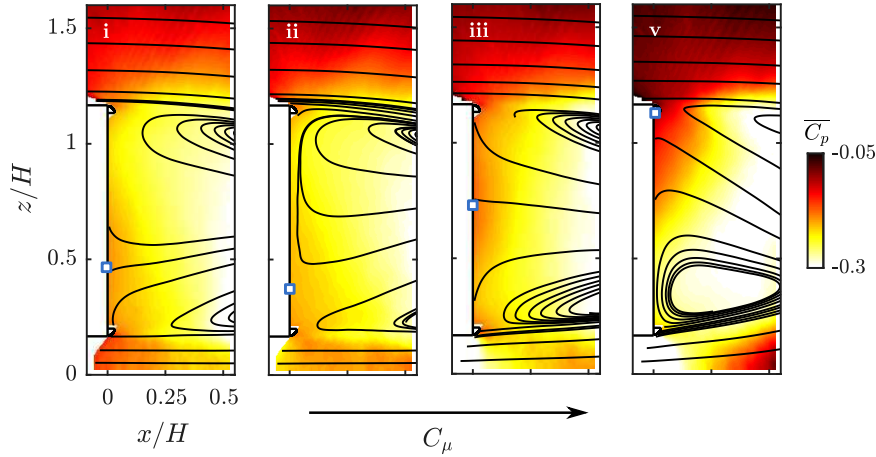
Figure 6.10: Mean pressure field \overline{C_p} in the near-wake superimposed with mean velocity streamlines under F_{\text{BLR}} forcing for forcing amplitudes indicated by the roman numerals in figure 6.9(a). Blue square symbols indicate the position of the mean reattachment point on the base.
