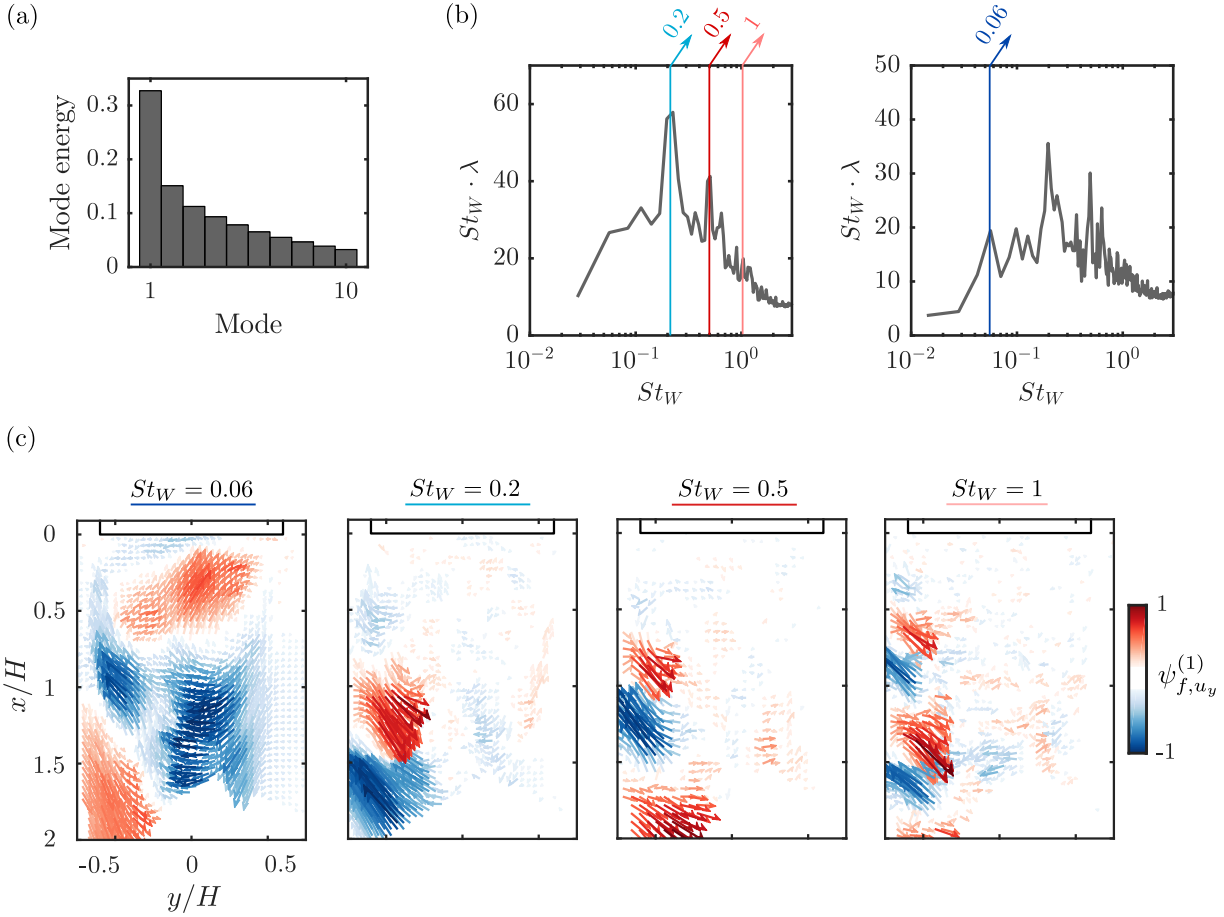
Figure 4.11: Spectral proper orthogonal decomposition (SPOD) of the velocity field for the wake locked in the lateral asymmetric state R . (a) Energy ratio of the 10 first modes spectra \int \lambda_f^{(i)} df / \sum_i \int \lambda_f^{(i)} df . (b)
