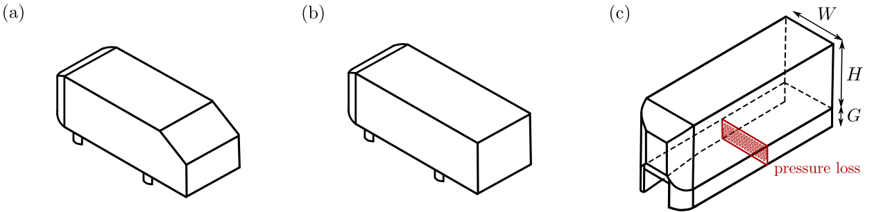
Figure 1.6: Simplified ground vehicles. (a) Original slanted Ahmed body introduced by Morel (1978) and Ahmed et al. (1984) representative of hatch-back vehicles. (b) Square-back Ahmed body. (c) Heavy-truck model introduced by Szmigiel (2017) and Castelain et al. (2018) . The underbody is closed by skirts and crossed by drilled plates to alter the momentum of the underbody flow and be more representative of heavy-trucks flows.
