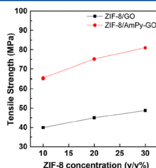
Figure 10. Tensile strength of ZIF-8/pristine GO and ZIF-8/4AmPy-GO composites containing different concentrations (v/v%) of ZIF-8.
