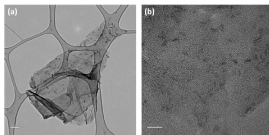
Figure 9. TEM images of ZIF-8/4AmPy-GO nanosheets. (ZIF-8:4AmPy-GO = 3:7) Scale bar = 0.2\text{ }\mu\text{m} (Figure 9a) and 50\text{ nm} (Figure 9b), respectively.
