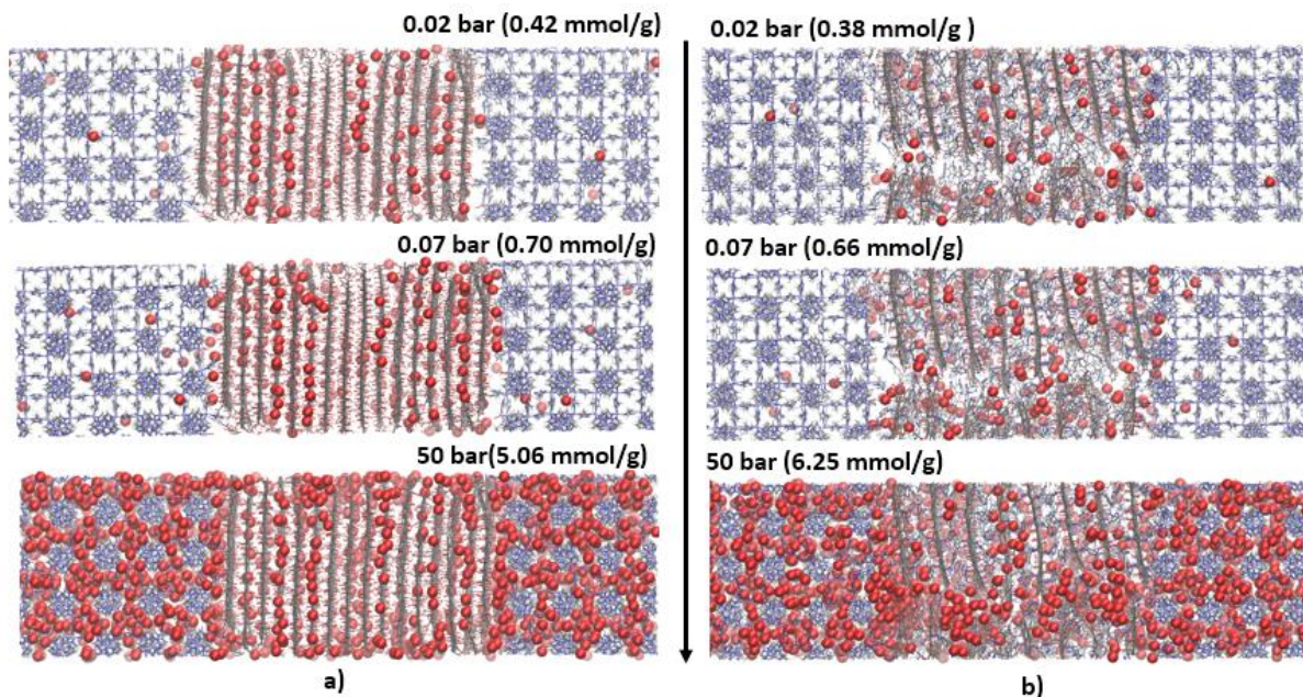
Figure 5.19 Illustration of the CO 2 adsorption at 298 K and varying pressures in a) ZIF-8/pristine-GO and b) ZIF-8/FGO
