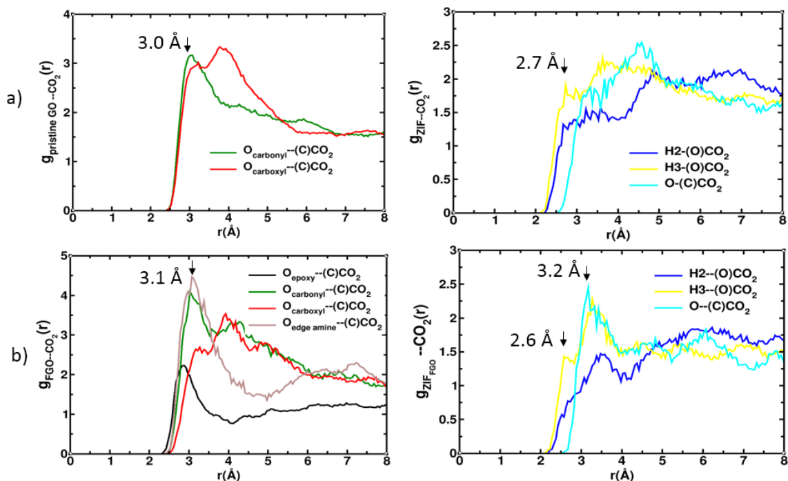
Figure 5.21 RDFs of CO 2 molecules with a) ZIF-8/pristine-GO and b) ZIF-8/FGO composites with respect to GO sites(left) and MOF sites (right) calculated from the GCMC simulations performed at 1 bar and 298 K
