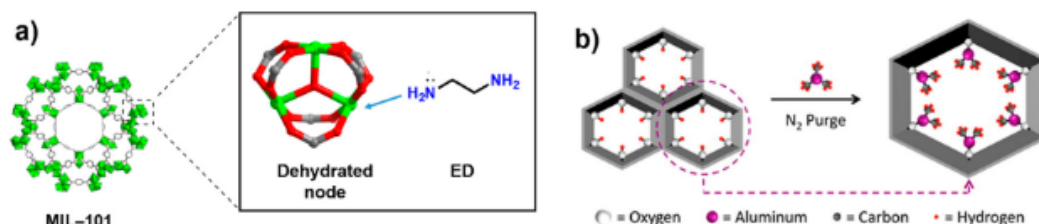
Figure 1.8 a) The preparation of ED-MIL-101, b) \text{AlO}_x clusters on NU-1000 using ALD. Adapted from Ref.[98]
