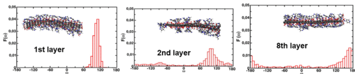
Figure 5.12 Dihedral angle distributions of the 1st, 2nd and 8th layers of FGO attached to the ZIF-8 surface averaged over the MD simulations
