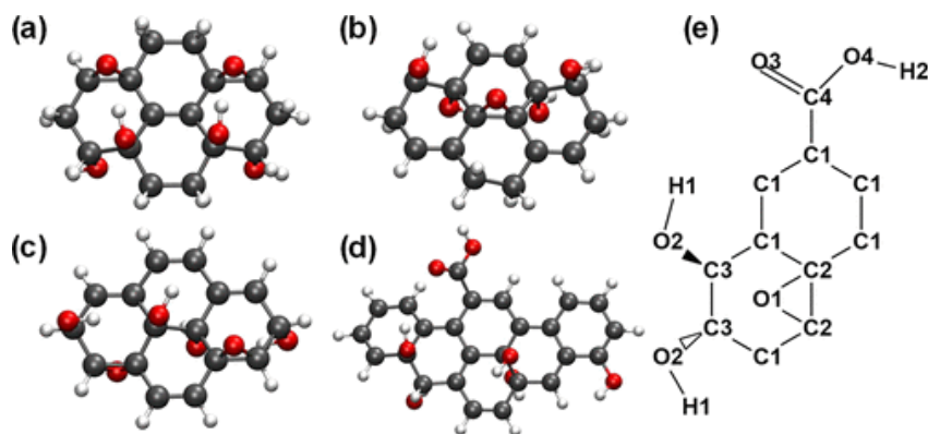
Figure 3.3 (a–c) and d) are the molecular fragments that were considered for charge calculations in the structural models of GO-OH and GO-CO 2 H, respectively. e) Labels of the atoms present in the GO-OH and GO-CO 2 H models
