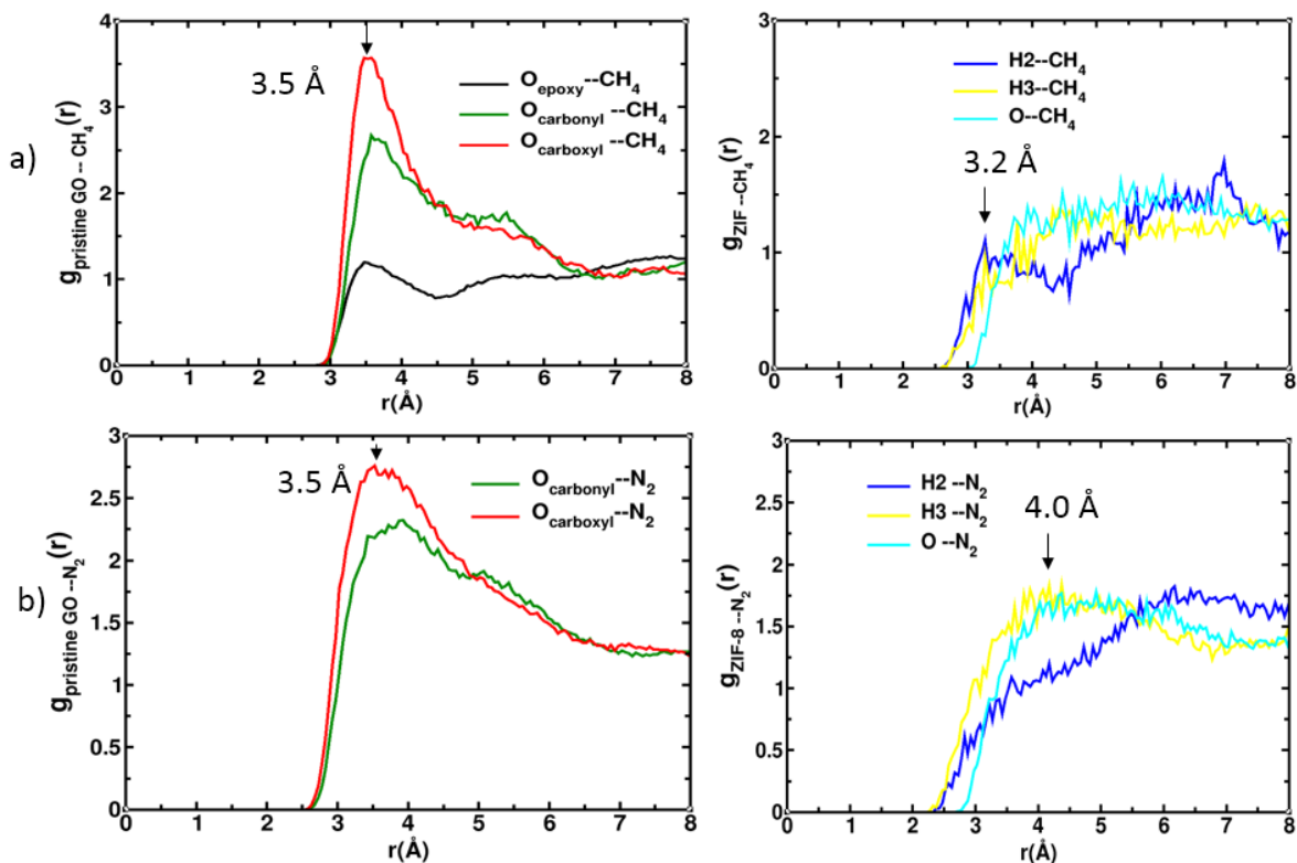
Figure 5.22 RDFs calculated for ZIF-8/pristine-GO a) CH 4 molecules performed at 1 bar and 298 K and b) N 2 molecules performed at 5 bar and 298 K with respect to GO sites(left) and MOF sites (right) calculated from the GCMC simulations
