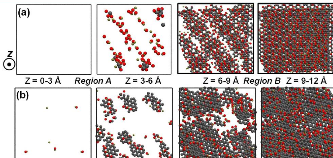
Figure 7. Snapshots of the slices of GOs of z = 3 Å width plotted as a function of the z distance away from the top of the MOF surface: (a) ZIF-8/GO-OH and (b) ZIF-8/GO- CO_2H . Zn atoms in the most external layers of ZIF-8 are considered as a reference for z = 0 .
