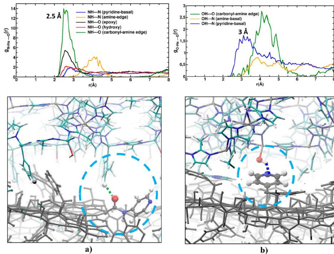
Figure 6. Radial distribution functions plotted for different ZIF-8/4AmPy-GO atom pairs above. (a) \text{-NH} (ZIF-8) and (b) \text{-OH} (ZIF-8) terminations with all the oxygen and nitrogen containing groups of 4AmPy-GO. Subsequent snapshots are shown below as illustrations. The color scheme of ZIF-8 and GOs are kept the same as in the above figures.
