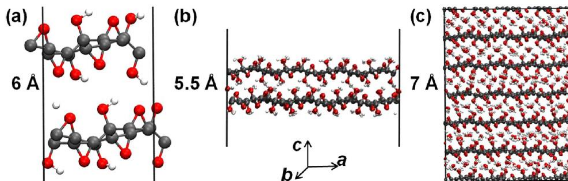
Figure 1. Optimized periodic models of GO-OH: (a) DFT simulations resulting in a desolvated model of 9 \text{ Å} \times 9 \text{ Å} \times 30 \text{ Å} dimensions with an interlayer distance of 6 Å; (b) force-field-based molecular dynamics (MD) simulations resulting in a desolvated model of 36 \text{ Å} \times 36 \text{ Å} \times 90 \text{ Å} dimensions (a higher value along the c axis is considered to exclude the interactions along this direction within the classical force field limit due to periodic boundary conditions with an interlayer distance of 5.5 Å); (c) force-field-based MD simulations resulting in a model containing 15 wt % water of 34 \text{ Å} \times 36 \text{ Å} \times 42 \text{ Å} dimensions with an interlayer distance of 7.0 Å. Color scheme: C, gray; O, red; and H, white.
