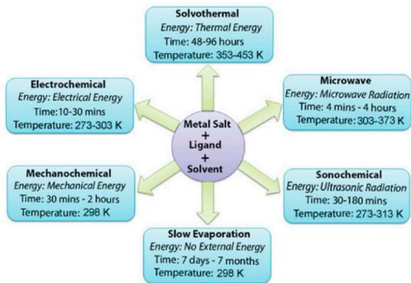
Figure 1.7 Synthesis methods of MOFs preparation. Adapted from Ref.[ 93 ]
