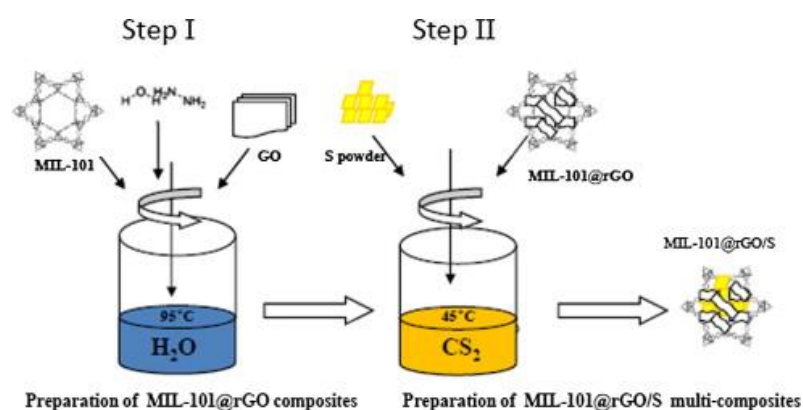
Figure 1.15 Direct mixing method used to prepare MIL-101(Cr)@rGO composite and MIL-101(Cr)@rGO/S multi-composites. Adapted from Ref.[ 195 ]
