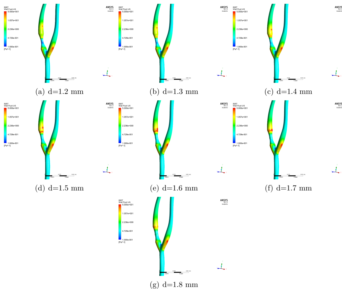
Figure 3.14: Relative Residency Time Near wall quantities for simplified model with different stenosed lumen diameter ( d )
