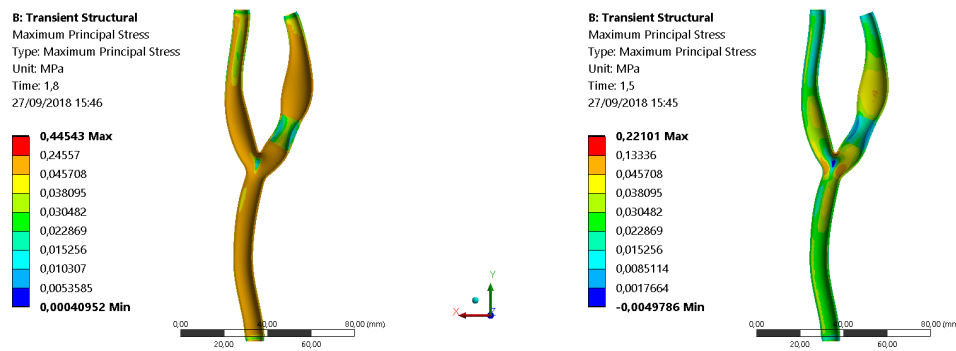
Figure 4.4: Maximum principal stress of the simplified carotid artery during systole (left) and diastole (right)
