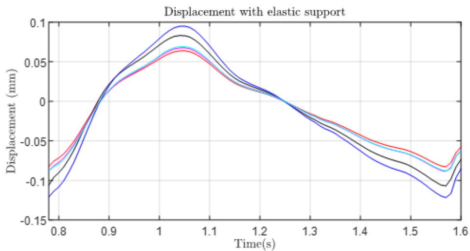
Figure 4.19: Displacement of specific nodes of the carotid model with elastic support
