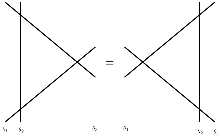
Figure 1.2: Factorization of the scattering process of 3 particles : the Yang-Baxter equation. Each line of the picture is interpreted as a trajectory of one of the particles (with rapidities \theta_{1,2,3} ) in the two dimensional space-time. An intersection between the lines correspond to the occurrence of a scattering process described by the corresponding entry of the S matrix.
