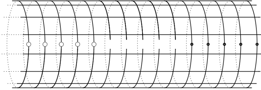
Figure 4.3: 19 vertex model on a cylinder with quasi-local insertion. The broken lines represent the spaces where the action of \mathcal{O} is non trivial, full circles represent the operator q^{\kappa H_j} , empty circles represent the operator q^{(\kappa+\alpha)H_j} .
