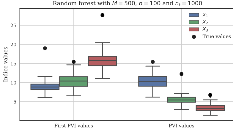
Figure 3.8 Estimation of the PVI and fPVI values when using a random forest model \hat{\eta}_M with M = 500 and a trained sample of n = 100 and a test-sample size n_t = 1000 .
