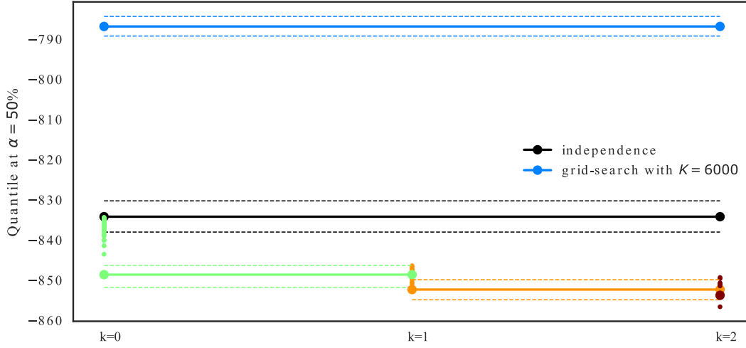
Figure 5.8 Minimum quantile results with the iteration k of the iterative procedure. The quantile at independence is shown in dark line. The minimum quantiles from Method 1 is shown in blue lines. The other lines and dots colors are the results from Method 2. For each iteration, the small dots are the estimated quantiles of all candidates and the point is the minimum. The 95 % bootstrap confidence intervals are also displayed for the independence and each minimums.
