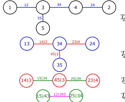
Figure 5.11 R-vine structure for d = 5 .
