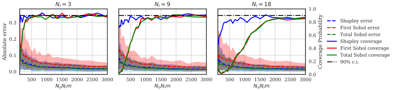
Figure 4.3 Variation of the absolute error and the POC with m for three values of N_i = 3, 9, 18 and N_o = 3 for the random permutation algorithm.
