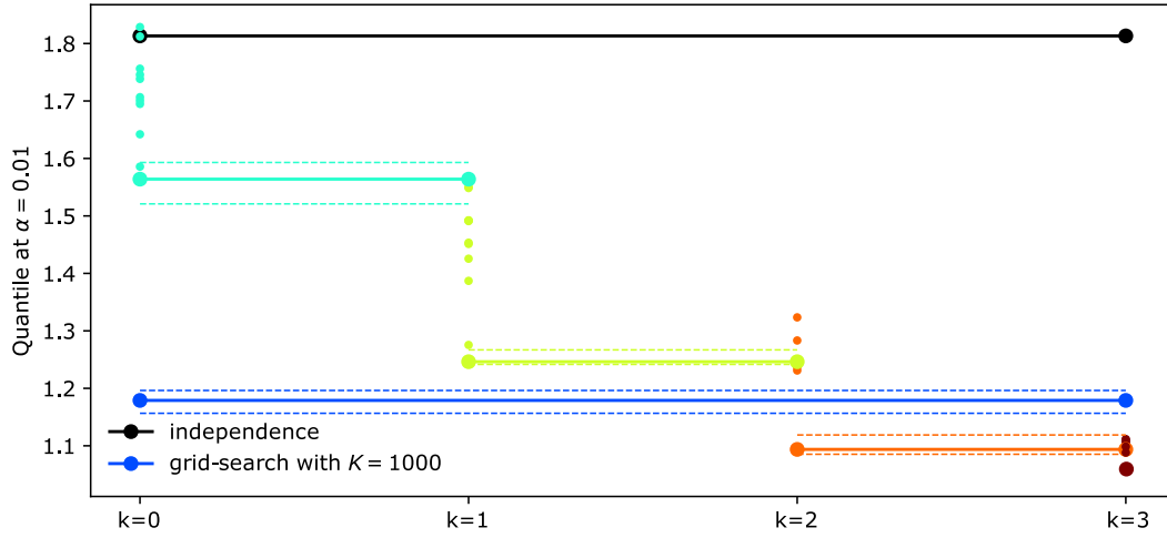
Figure 5.10 Minimization of the output quantile using a grid-search and the iterative procedure for \alpha = 1\% . The description is the same as in Figure 5.8.
