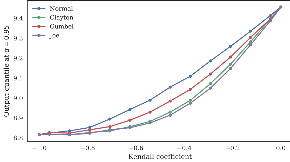
Figure 5.3 Variation of the quantile of the overflow distribution with the Kendall coefficient \tau for \alpha = 95\% and different copula families (Gaussian, Clayton, Gumbel and Joe).
