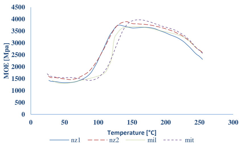
Figure 1: Thermomechanical analysis (TMA) of wood panels prepared with tannin-hexamine adhesives: comparison of elasticity modulus (MOE, MPa) obtained for different laboratory-made wood bark extracts area. With Nz=Nzamaligue ; Mil=Milole ; Mit= Mitzic
