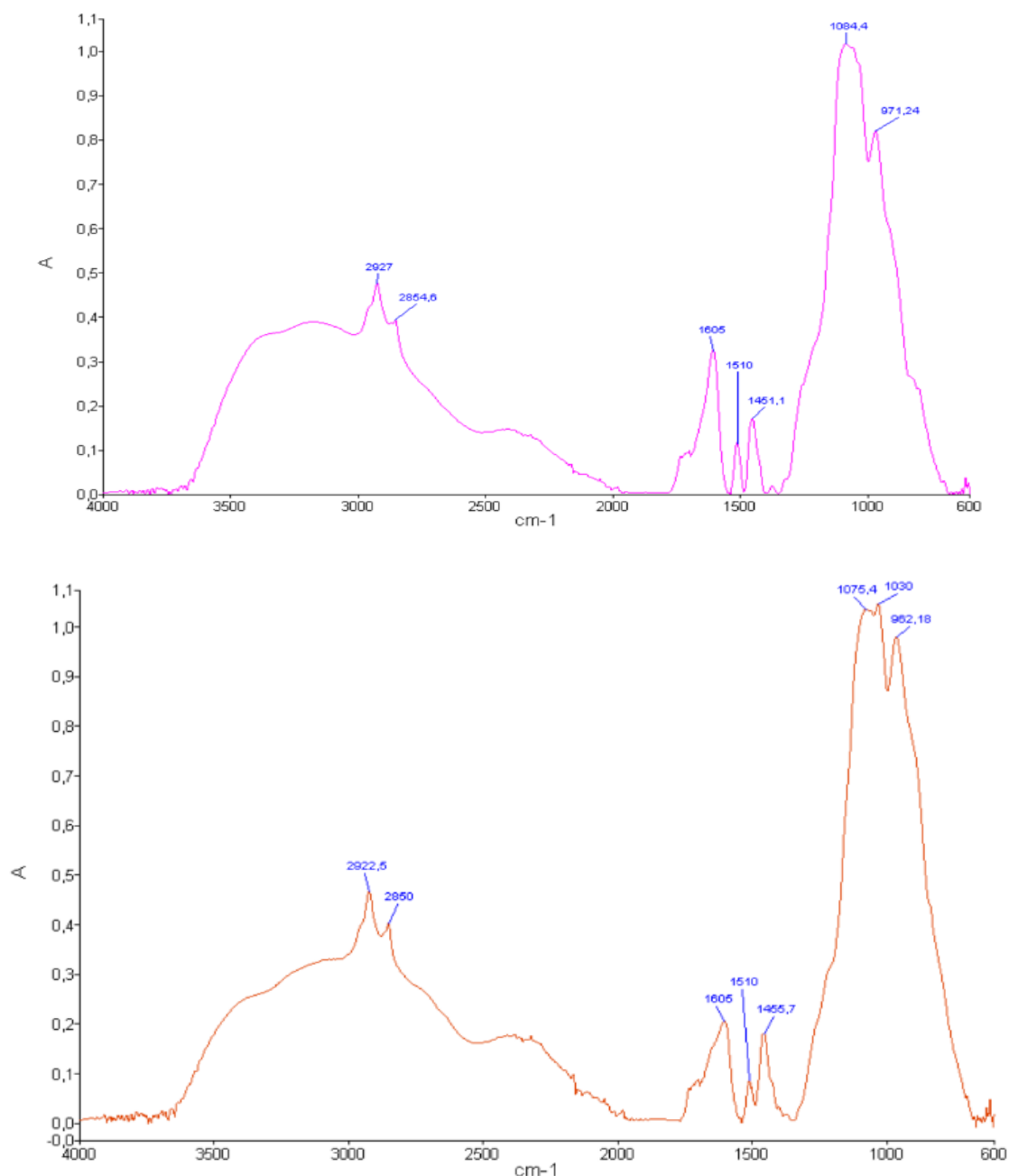
Figure 7. FTIR spectra of heartwood (a) and sapwood (b) extractives
