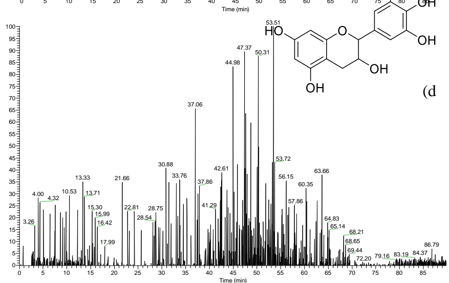
Figure 2. Mass fragments of the main monomers ( a =glucose; b =trihydroxyflavan-3-ol; c =fisetinidin; d =galocatechin).
