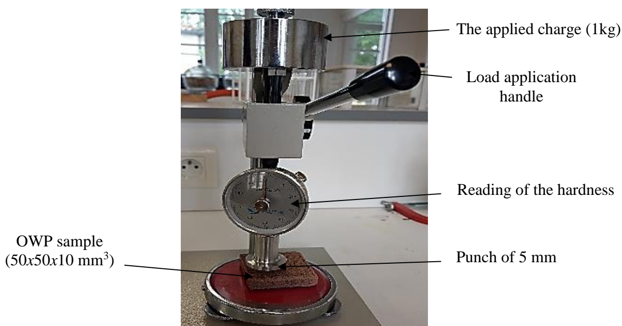
Figure 4: Shore AO hardness-testing device
