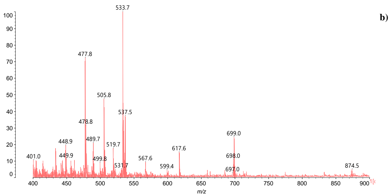
Figure 5. Maldi-ToF spectra of heartwood (a) and sapwood (b) in the range 400-900 Da
