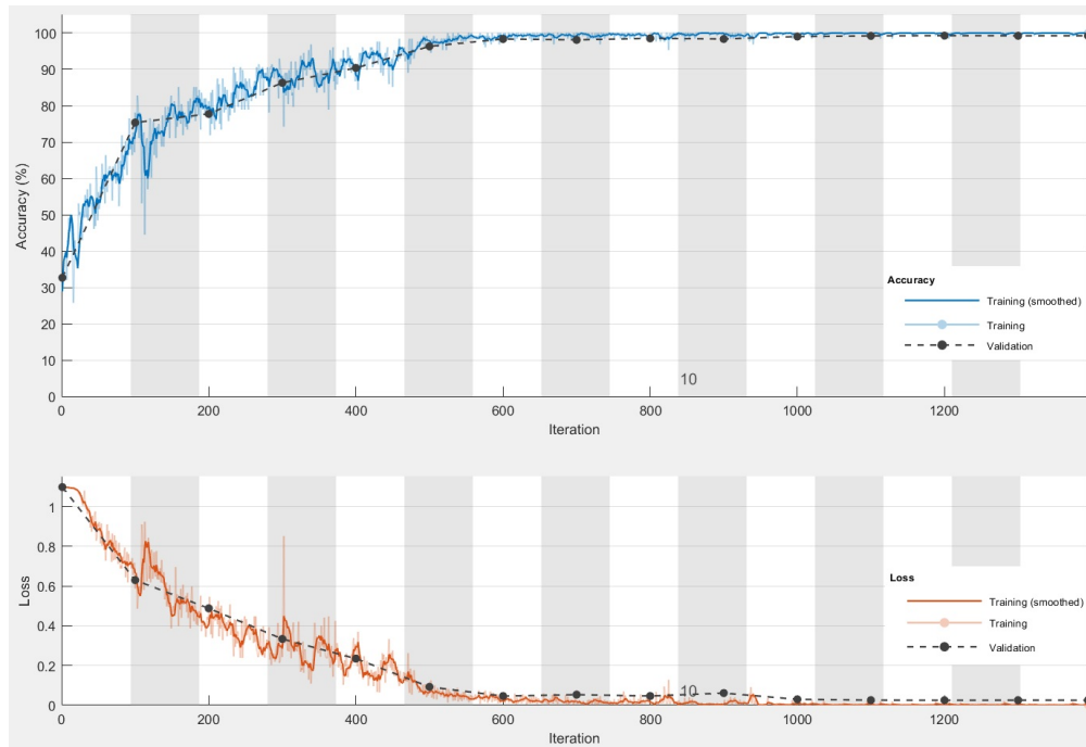
Figure (5.17) Training vs validation performance of the CNN architecture 1
