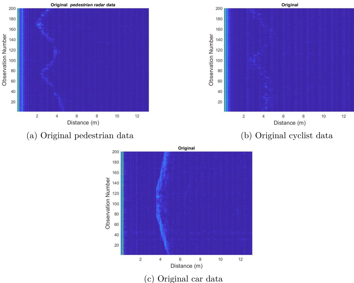
Figure (5.1) Original B-scan radar data for three different targets
