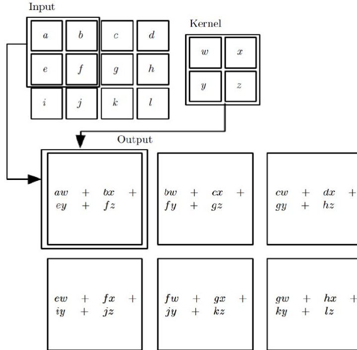
Figure (5.11) Illustration of 2-D convolutional process (source: [87])
