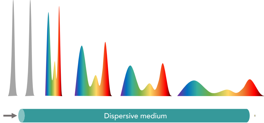
Figure 5.6 Schematic of dispersive-Fourier transform principle. Figure adapted from [48].
