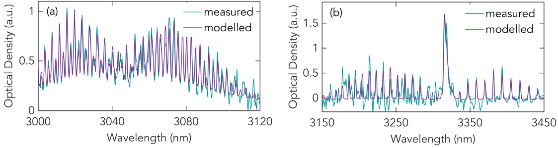
Figure 3.5 Optical density of (a) acetylene with 5 ppm concentration and (b) methane with 4 ppm concentration. The blue line corresponds to experimental measurements and the purple line to a least-square fit model using Eq. (3.13). Adapted from Publication I.
