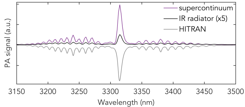
Figure 4.6 Comparison of the mid-infrared ro-vibrational methane absorption lines measured with the 400 kHz SC source (purple) and black-body source (black). The theoretical absorption computed from the HITRAN 2012 database is also shown (gray). All the measurements presented were averaged over 10 scans in order to reduce the noise level. Adapted from Publication II.
