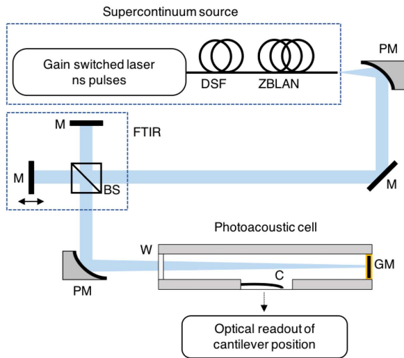
Fig. 1. Experimental setup. PM, off-axis parabolic mirror; M, mirror; BS, beam splitter; W, window; GM, gold mirror; C, cantilever.
