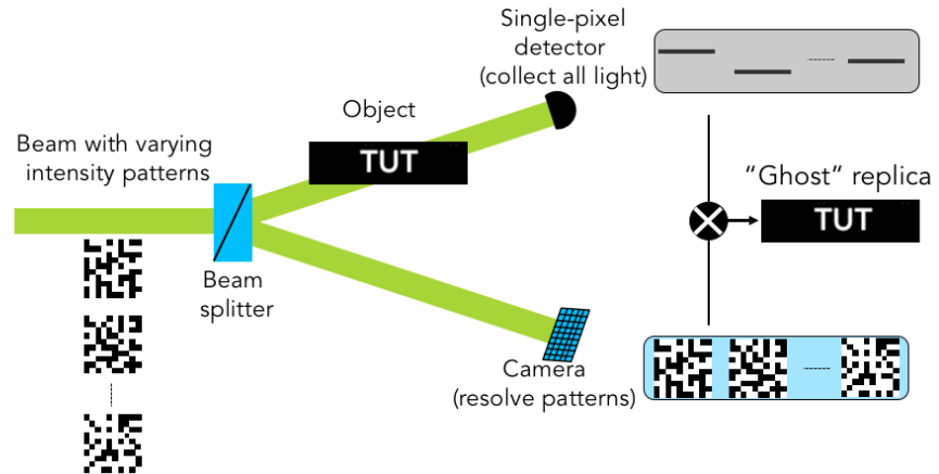
Figure 5.2 Schematic illustration of spatial ghost imaging.
