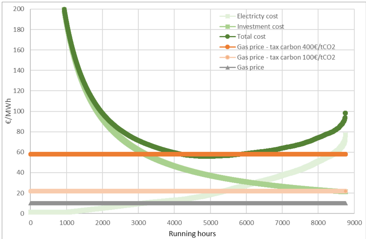
Figure 75 : P2G total cost and gas price in function of carbon tax – Ampere case
