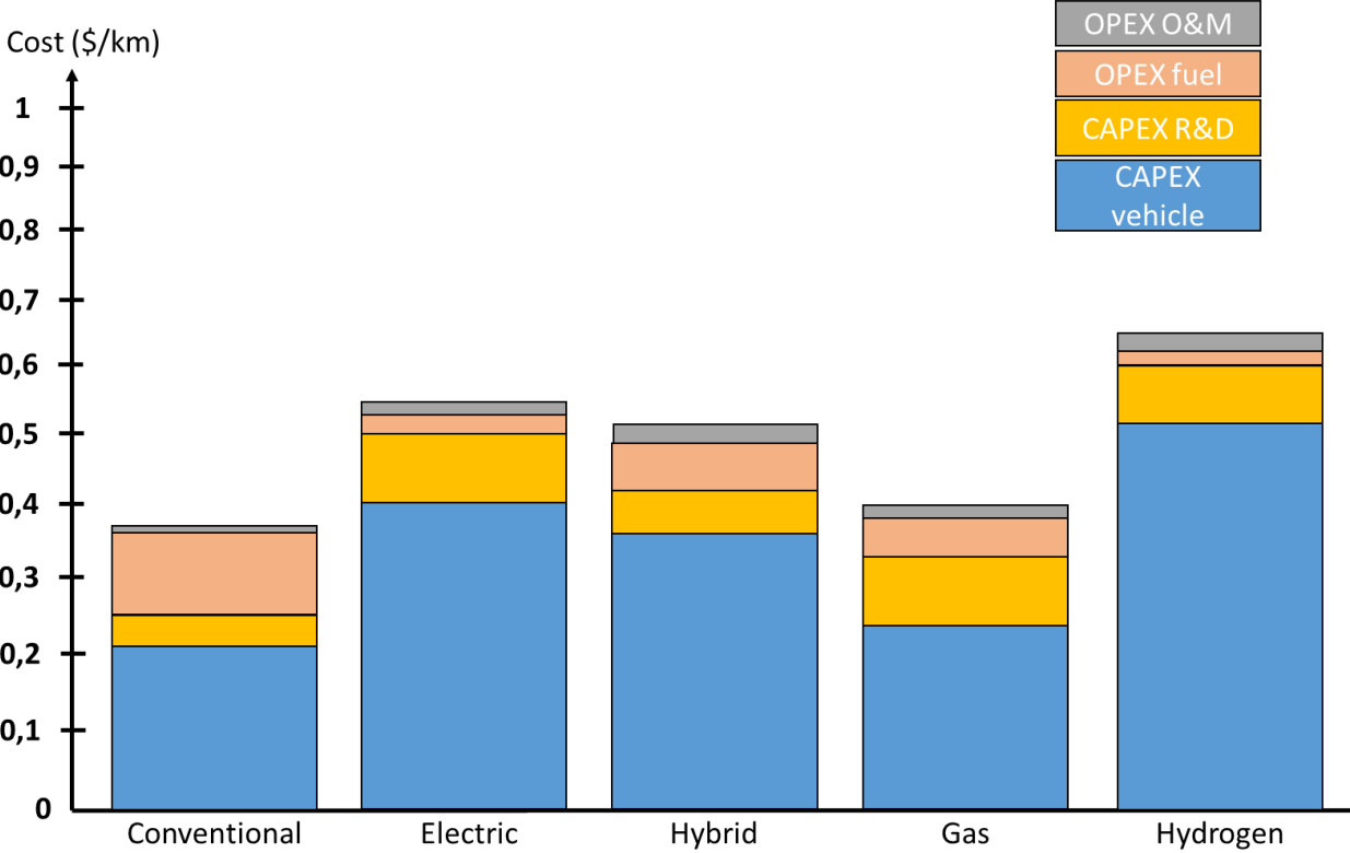
Figure 49 : Vehicles costs structure in POLES model in 2017
