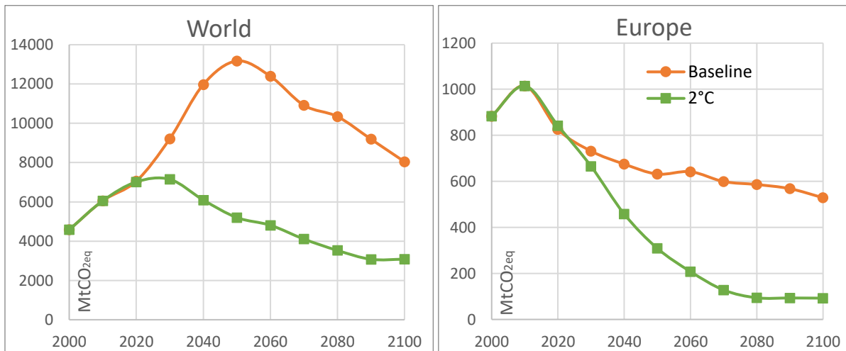
Figure 33 : World and Europe GHG emissions by gas Scenarios baseline and 2°C POLES-GAEL
