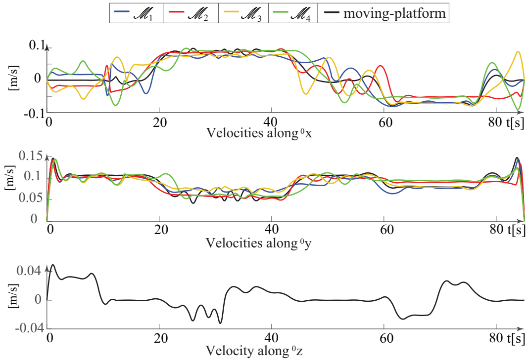
Figure 6.14: MoPICK velocity profiles for a test scenario
