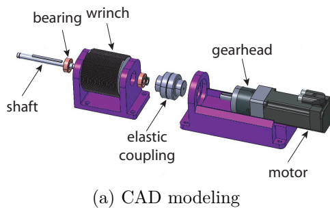
Figure 1.7: FASTKIT actuation and transmission system
