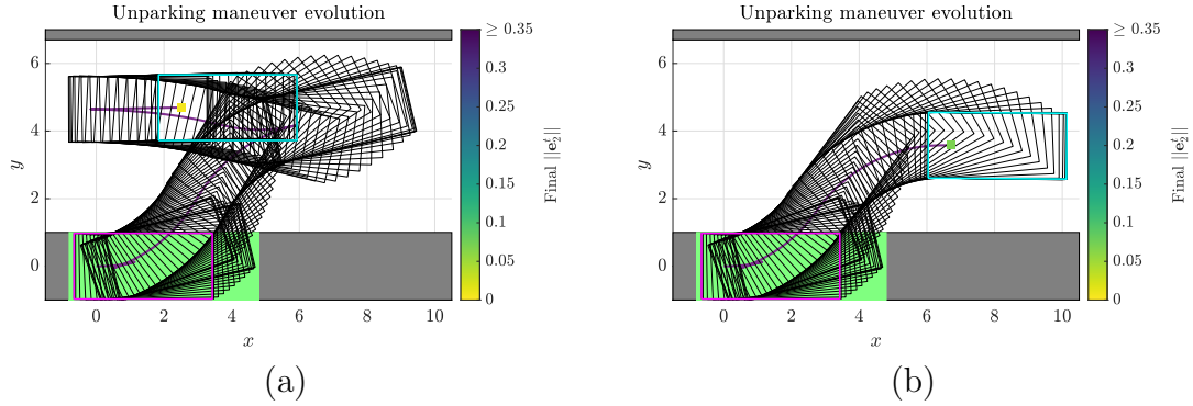
Figure 4.20: Constrained \| forward unparking maneuvers. (a) Desired pose = (2.5 m, 4.7 m, 0^\circ ), (b) Initial pose = (6.7 m, 3.5 m, 0^\circ )
