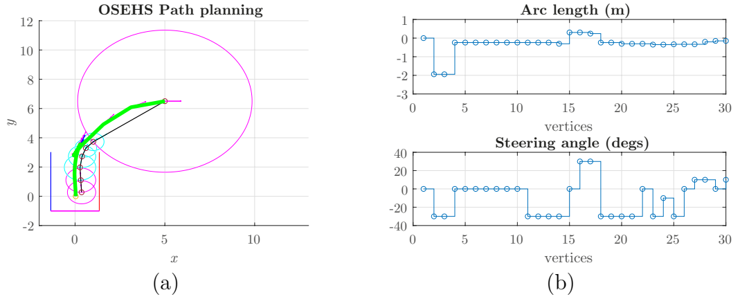
Figure 3.17: OSEHS Path planning approach results: three maneuvers are required. Initial pose = (5m, 6.5m, 0°).
