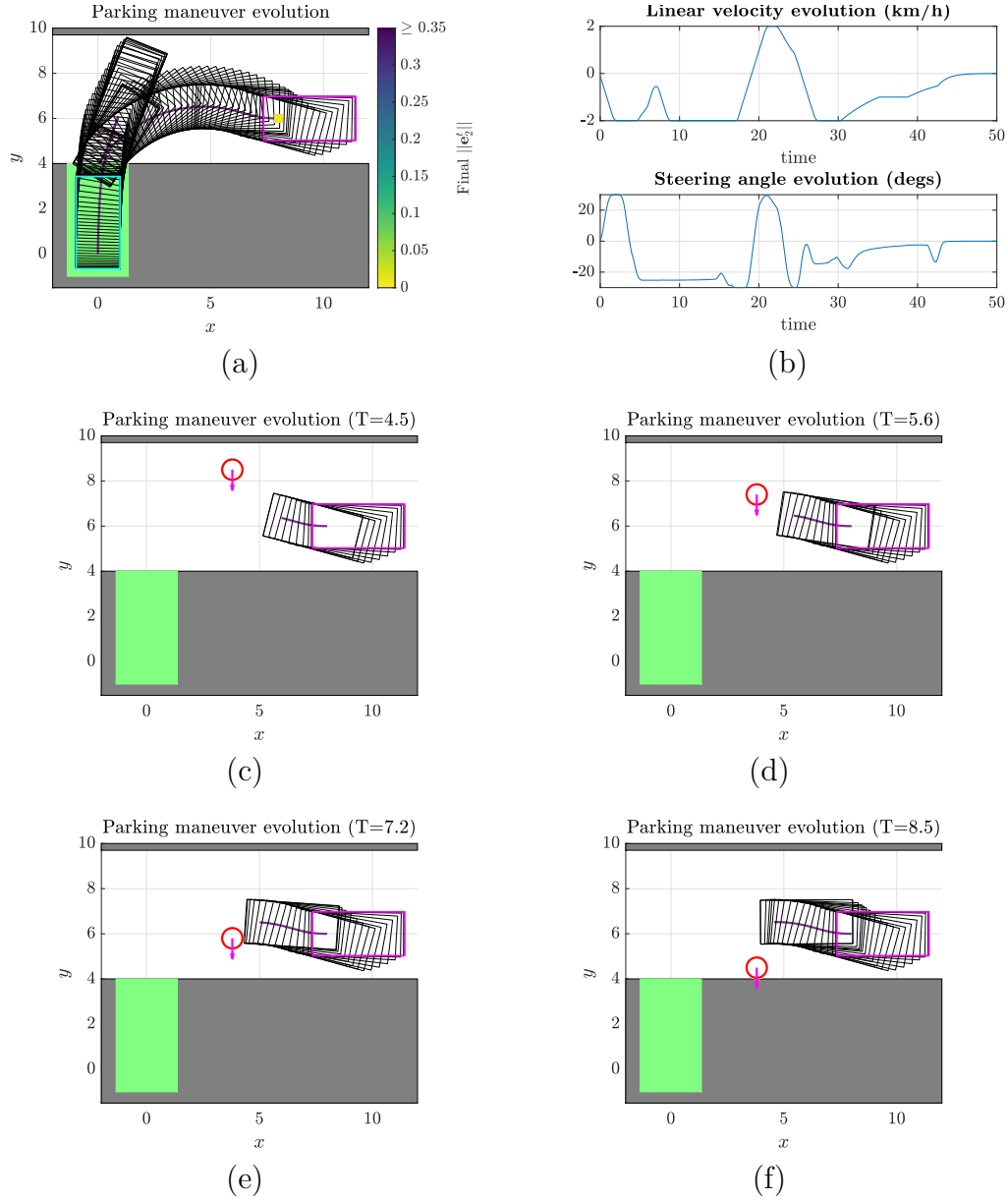
Figure 4.15: Constrained \perp backward parking maneuver with a moving obstacle traveling from top to bottom
