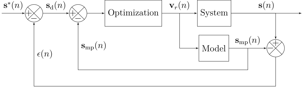
Figure 4.3: Control structure [63]
