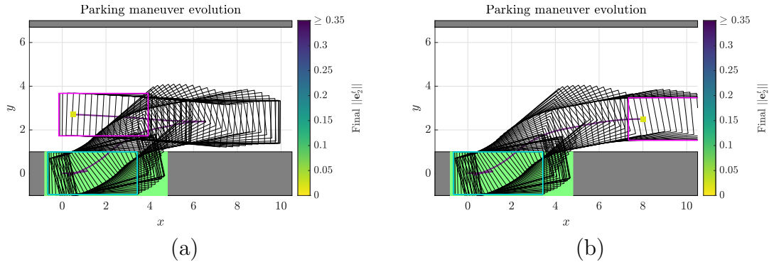
Figure 4.9: Constrained \parallel backward parking maneuvers. (a) Initial pose = (0.5 m, 2.7 m, 0^\circ ), (b) Initial pose = (8 m, 2.5 m, 0^\circ )
