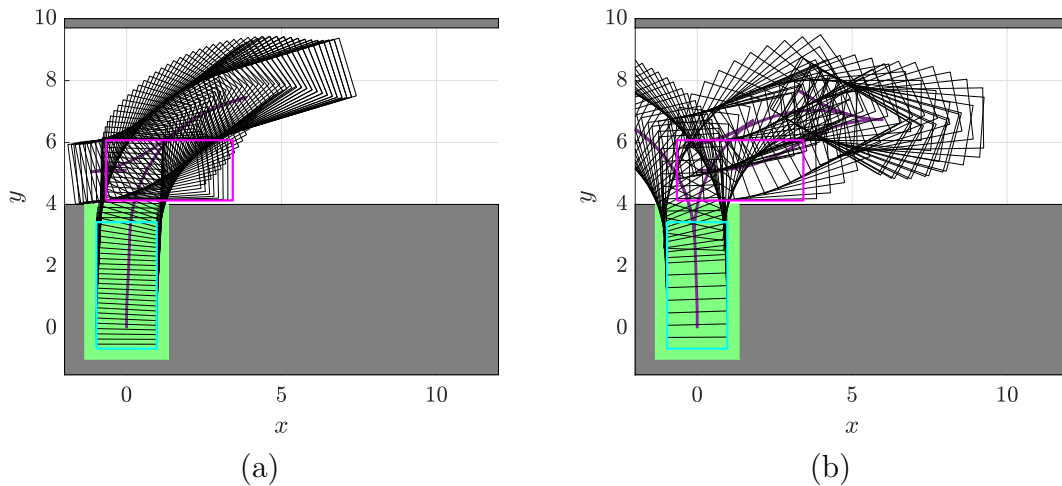
Figure 4.12: RRT* path planning results using HC^{00} -RS steering function. Initial pose = (0m, 5.1m, 0^\circ)
