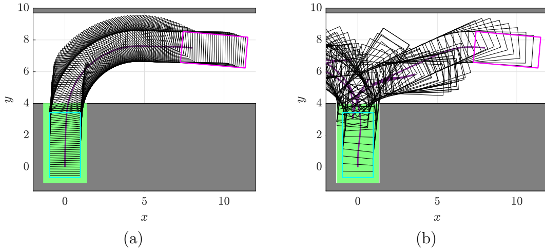
Figure 4.11: RRT* path planning results using HC^{00} steering function. Initial pose = (8m, 7.5m, -5^\circ)
