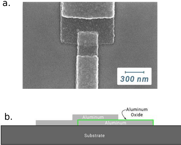
Figure 1.2: In panel (a.) is a scanning electron microscope image of a Al/Al 2 O x /Al Josephson junction from Ref. [13]. In panel (b.) a transverse diagram of the junction. Aluminum is superconducting at T < 1.2K while the oxide remains metallic at this temperature.
