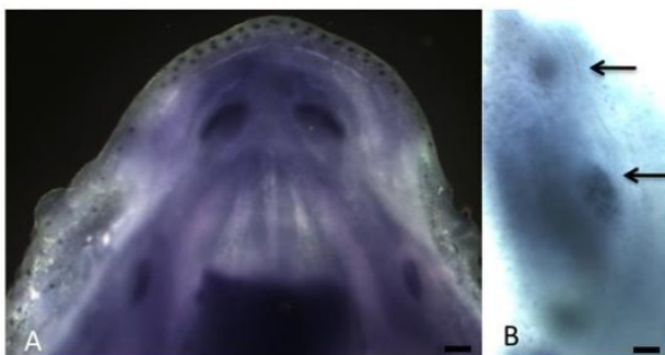
Figure 6. Whole mount in situ hybridization showing the molar and incisor placodes within the mandible at E14.5 in a wild-type mouse (A) and Rsk2 - Y mouse (B: detail of the right-side mandible) labelled with a Shh riboprobe. Two molar placodes are clearly visible in B (arrows) Scale bars 200 \mu m (A), 100 \mu m (B). doi:10.1371/journal.pone.0084343.g006
