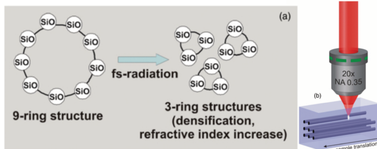
Figure 1.11: fs-laser writing of waveguide arrays in fused silica. (a) The intense fs-laser breaks the silica ring into small rings, which leads to densification or an increase in the refractive index in that region, and this is done by shining (b) a fs-laser along with a lens to focus on a particular region of interest. This supports a mode at wavelength \lambda = 633 nm, Fig. is from (Szameit and Stefan Nolte 2010)
