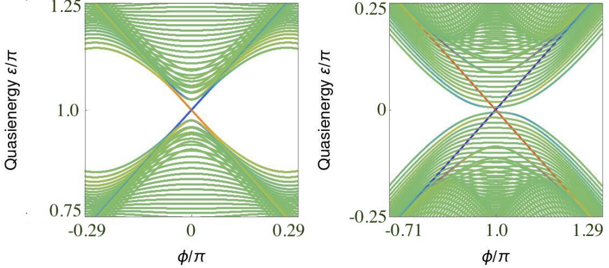
(a) Spectral flow associated to B_\pi
