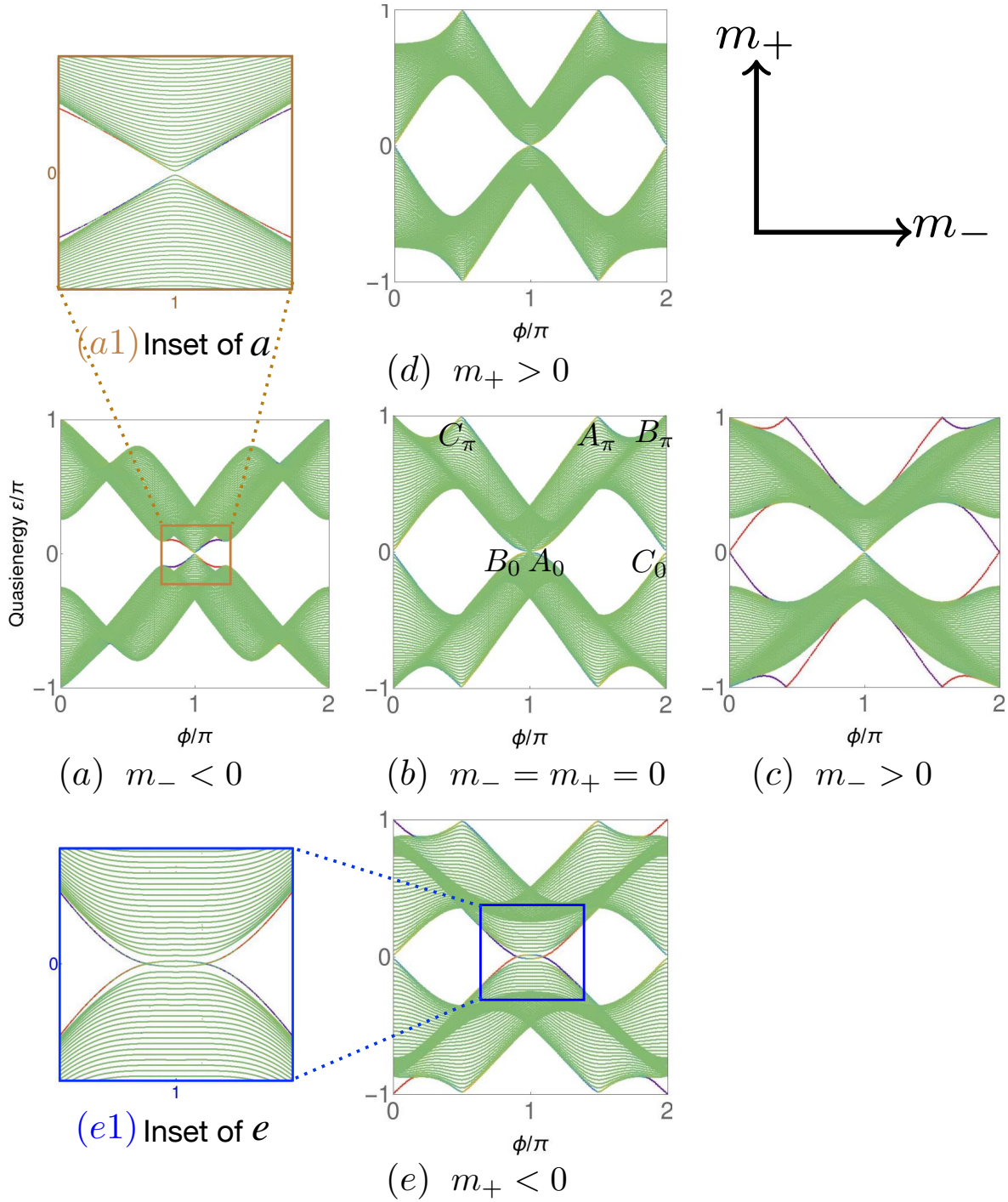
Figure 4.10: Quasienergy spectra of the four-step Floquet operator for \phi_1 = -\phi_2 = \phi_3 = -\phi_4 = \phi in finite geometry as a function of either m_+ or m_- . Imposing a vanishing of either m_+ or m_- prevents a gap opening at 0 and \pi so that all the spectra are gapless. The two insets (a1) and (e1) show edge states at \varepsilon = 0 that merge to the bulk bands and disappear, unlike other chiral edge states for m_\pm < 0 that live in local gaps.
