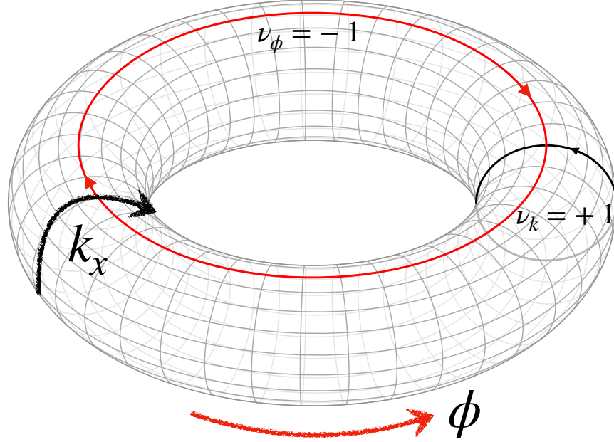
Figure 3.25: A general winding is made up of \{\nu_\phi, \nu_k\} and they can be represented on a torus using the underlying manifold of BZ. Then the number of windings along the bigger circle represents \nu_\phi and smaller one \nu_k , where the counter-clockwise direction can be chosen as a convention for positive values.
